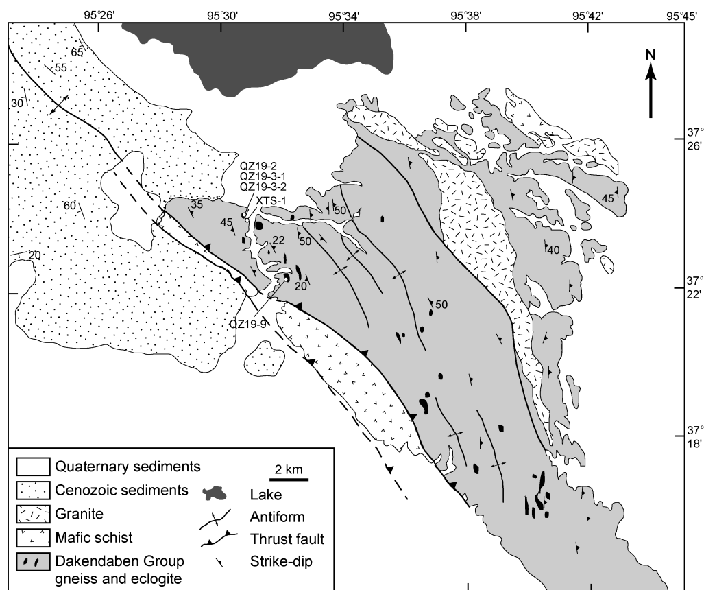
FIG. 3. Geologic map of the Xitie Shan area showing sample locations. The town of Xitie Shan is approximately 5 km south of map area. Modified from Zhang et al. (2005c).
