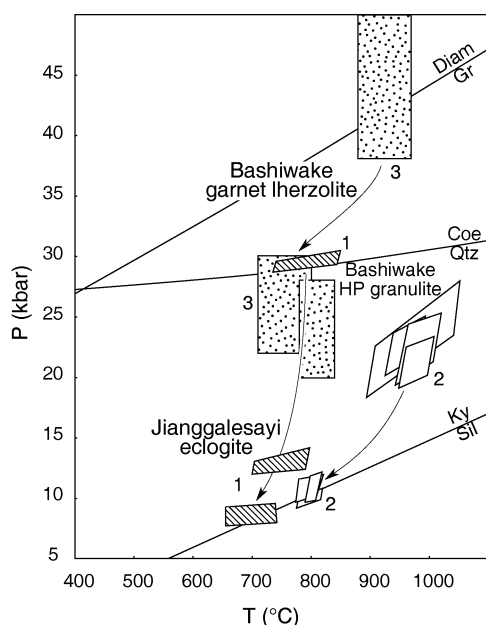
FIG. 12. Summary of thermobarometry from the Bashiwake and Jianggalesayi areas. Polymorphic transitions calculated from Holland and Powell (1998). References: 1 = Zhang et al., 2001, 2002; 2 = Zhang et al., 2005b; 3, Liu et al. = 2002.
