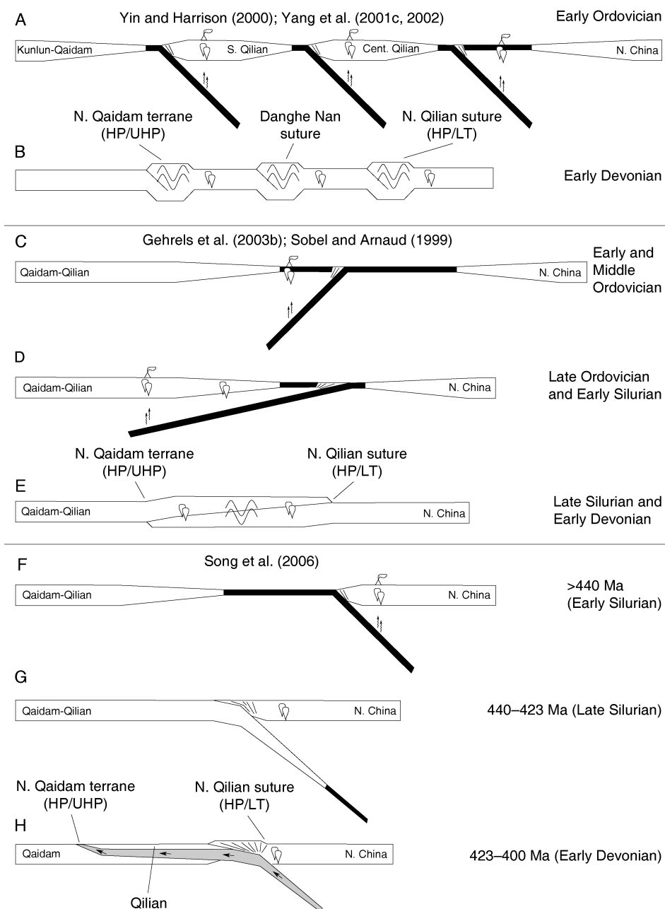
FIG. 15. Summary of proposed tectonic models, looking west. A–B. Model of Yin and Harrison (2000), Yang et al. (2001c). C–E. Model of Gehrels et al. (2003b). F–H. Model of Song et al. (2006).
