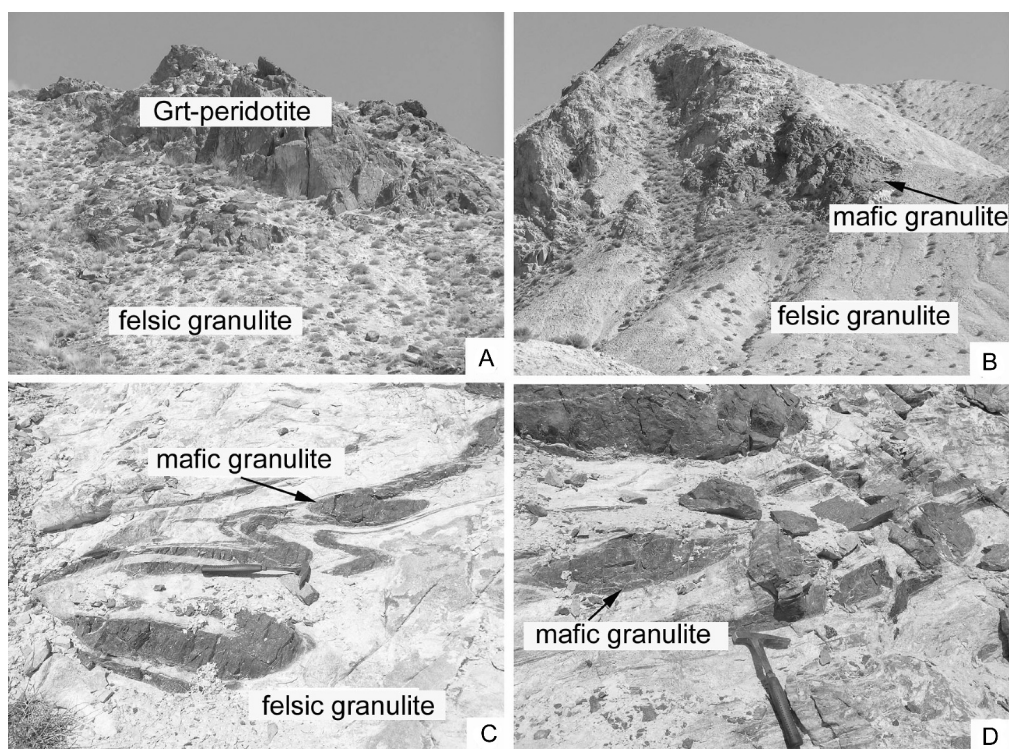
FIG. 11. Bashiwake felsic granulite enclosing garnet peridotite (A) and mafic granulite (B–D). Field of view in (A) and (B) is approximately 50 m.
