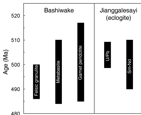
FIG. 13. Summary of geochronology from the Bashiwake and Jianggalesayi areas. Height of bars represents 2\sigma uncertainty. Data for Bashiwake from Zhang et al. (2005b), and data from Jianggalesayi are from Zhang et al. (2001).
