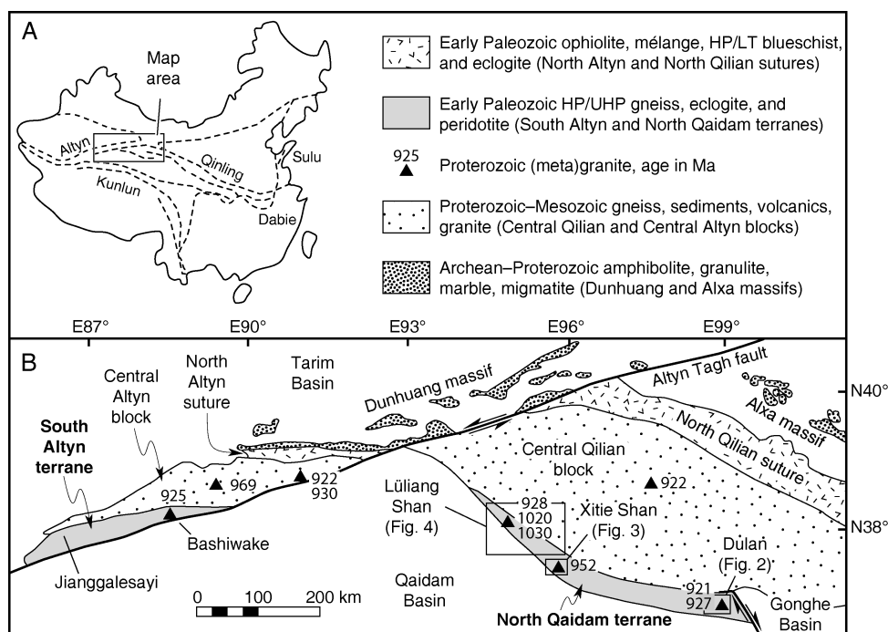
FIG. 1. A. Map of China showing the location of this study (box) and the trends of major mountain belts (dashed lines). B. Schematic map of the Qaidam-Qilian-Altnn Tagh region showing major tectonic units, and locations of eclogite and garnet peridotite. The boxes indicate the locations of Figures 2–4. Ages of Proterozoic (meta)granites are referenced in Table 2. The Wenquan fault is located in the southeast corner of the map, between the North Qaidam terrane and the Gonghe Basin. Modified from Zhang et al. (2005b).
