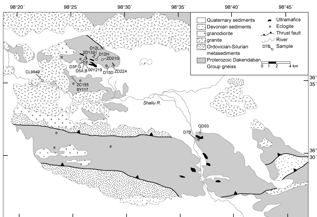
FIG. 2. Geologic map of the Dulan area showing sample locations. The town of Dulan is approximately 30 km southwest of map area. Modified from Yang et al. (2000), Wu et al. (2004), and new mapping by C.G. Mattinson.
