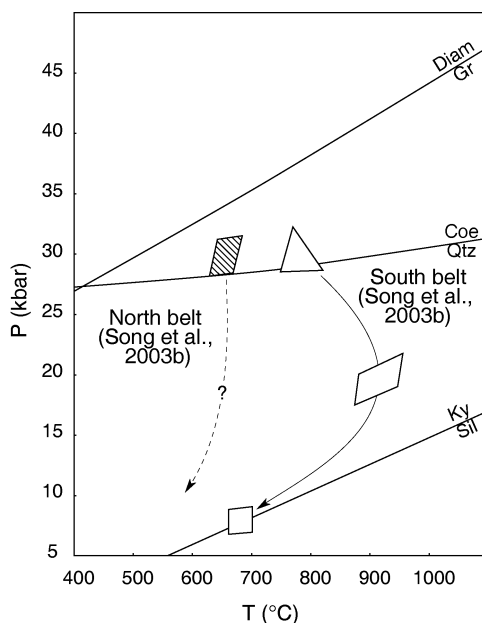
FIG. 6. Summary of thermobarometry from the Dulan area (Song et al., 2003b). Polymorphic transitions calculated from Holland and Powell (1998).
