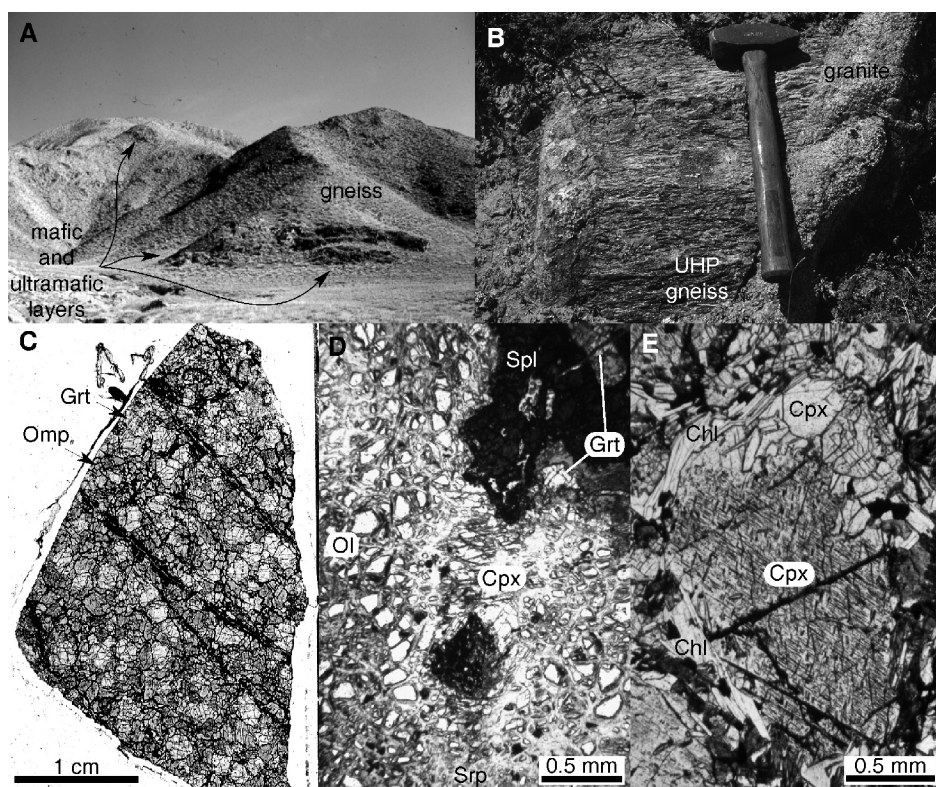
FIG. 5. A. Mafic and ultramafic layers in gneiss, north belt, view to the north. B. Yematan granite truncates foliation in Dakendaban gneiss. C. Thin section of typical coarse-grained eclogite. D. Strongly serpentinized garnet peridotite; garnet is largely replaced by spinel. Plane-polarized light. E. Chlorite clinopyroxenite, plane-polarized light. Clinopyroxene porphyroblasts contain oriented rods and plates of Cr-magnetite and Cr-chlorite. Note that inclusion-free porphyroblast rims and matrix clinopyroxene contact Cr-chlorite on straight grain boundaries.
