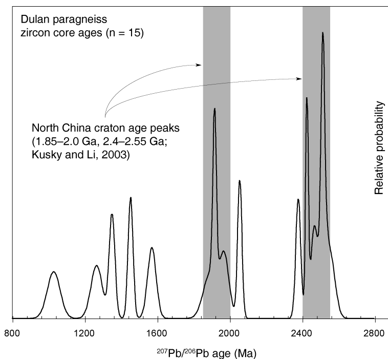
FIG. 8. Relative probability plot of zircon core ages from Dulan paragneiss samples. Probability peaks are similar to North China craton age peaks (grey bands).
