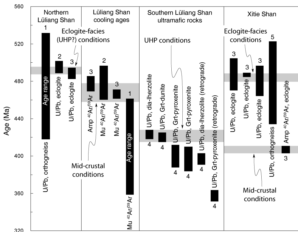
FIG. 10. Summary of geochronology from the Xitie Shan and Lüliang Shan areas. Height of bars represents 2\sigma uncertainty, except for bars labeled "age range," which represent the range of multiple analyses. Grey bands indicate age ranges associated with the labeled events. References: 1 = Menold et al., 2004; 2 = Zhang et al., 2000; 3, Zhang et al., 2005c; 4 = Song et al., 2005; 5 = Zhang et al., 2006.
