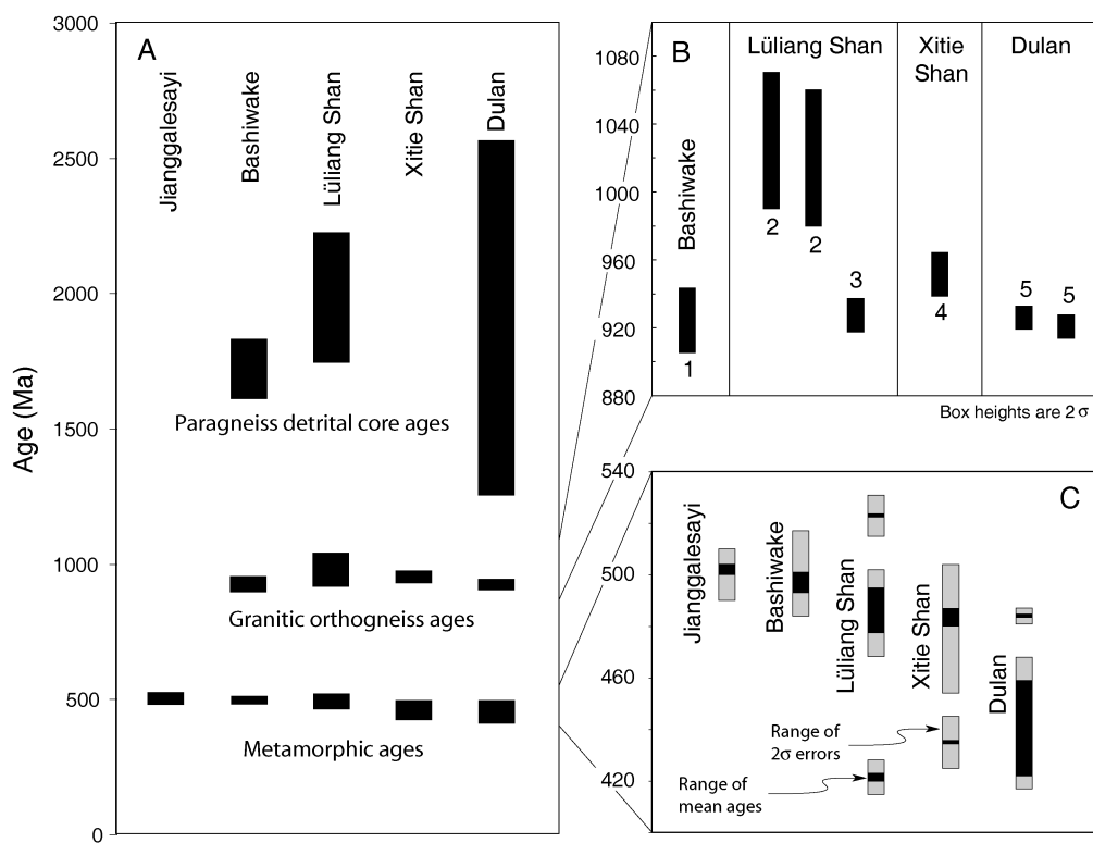
FIG. 14. Summary of zircon geochronology from the South Altyn and North Qaidam localities. A. Ages of paragneiss detrital cores, granitic orthogneiss, and ages interpreted to reflect high-pressure metamorphism. Height of bars represents the age range of multiple analyses. B. Ages of granitic orthogneiss samples, interpreted to reflect magmatic crystallization. Height of bars represents 2\sigma uncertainty. C. Ages interpreted to reflect high-pressure metamorphism. Black bars represent range of weighted mean ages, grey bars represent the range of 2\sigma uncertainty. Individual analyses outside the main group of analyses are plotted separately for Lüliang Shan, Xitie Shan, and Dulan. References: 1 = C. G. Mattinson, unpubl. data; 2 = Wan et al., 2001; 3 = Gehrels et al., 2003b; 4 = Zhang et al., 2006; 5 = Mattinson et al., 2006a.
