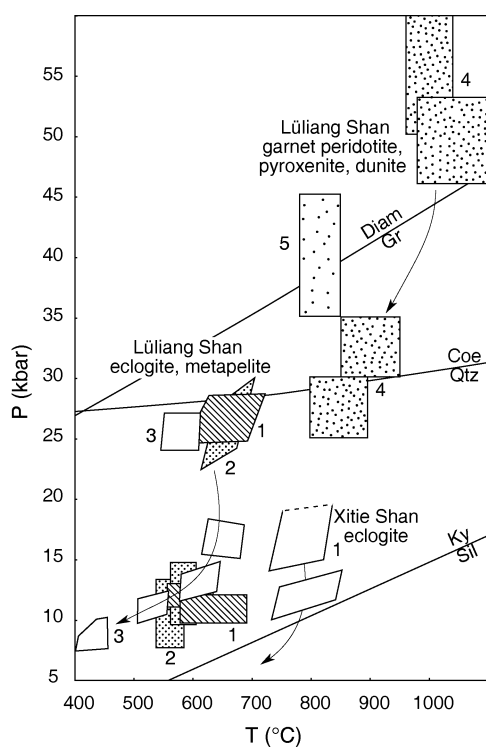
FIG. 9. Summary of thermobarometry from the Xitit Shan and Lüliang Shan areas. Polymorphic transitions calculated from Holland and Powell (1998). References: 1 = Zhang et al., 2005c (Lüliang Shan eclogite hatched, Xitit Shan eclogite unpatterned); 2 = Zhang et al., 2004a (metapelite, fine stipple); 3 = C. A. Menold.
