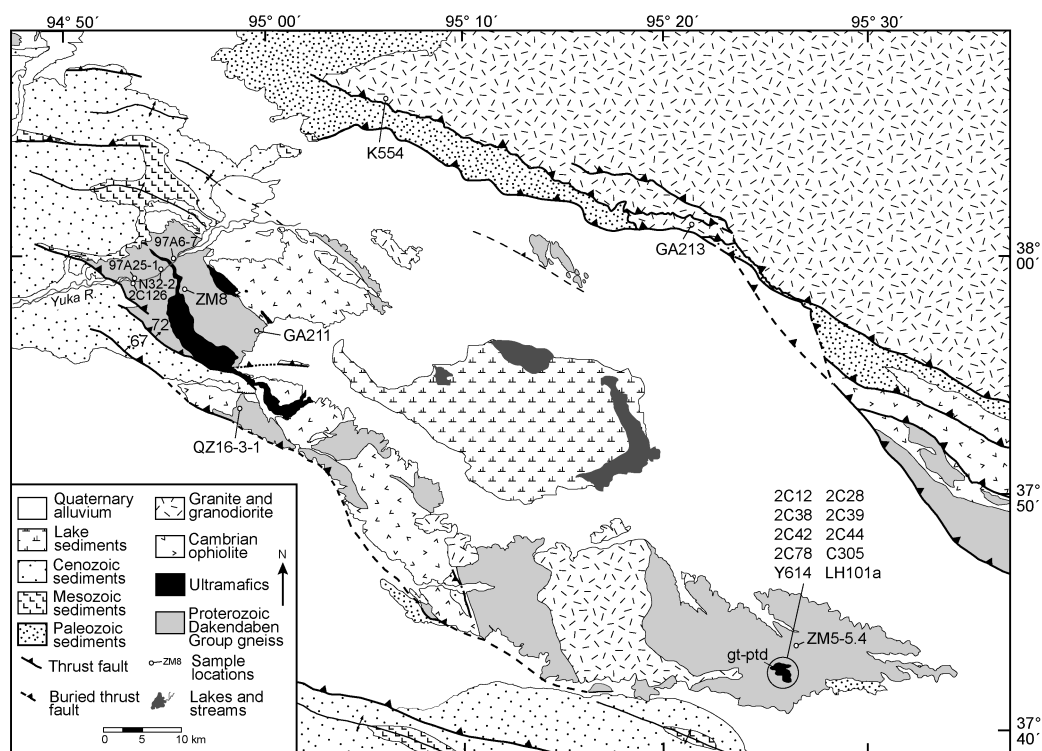
FIG. 4. Geologic map of the Liliang Shan area showing sample locations. Based on mapping by C.A. Menold.
