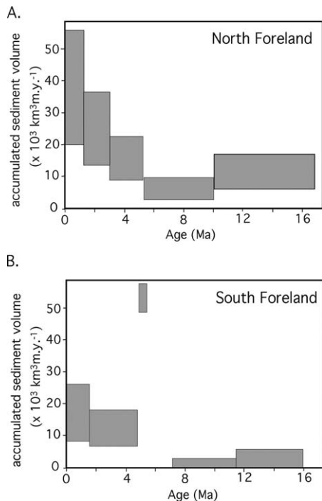
Figure 3. A: Sediment yield from northern Alpine drainages. Data are from Kuhlemann (2000), with modified range to reflect our estimate of uncertainty. B: Sediment yield from southern Alpine drainages (for methodology and data, see footnote 1).
