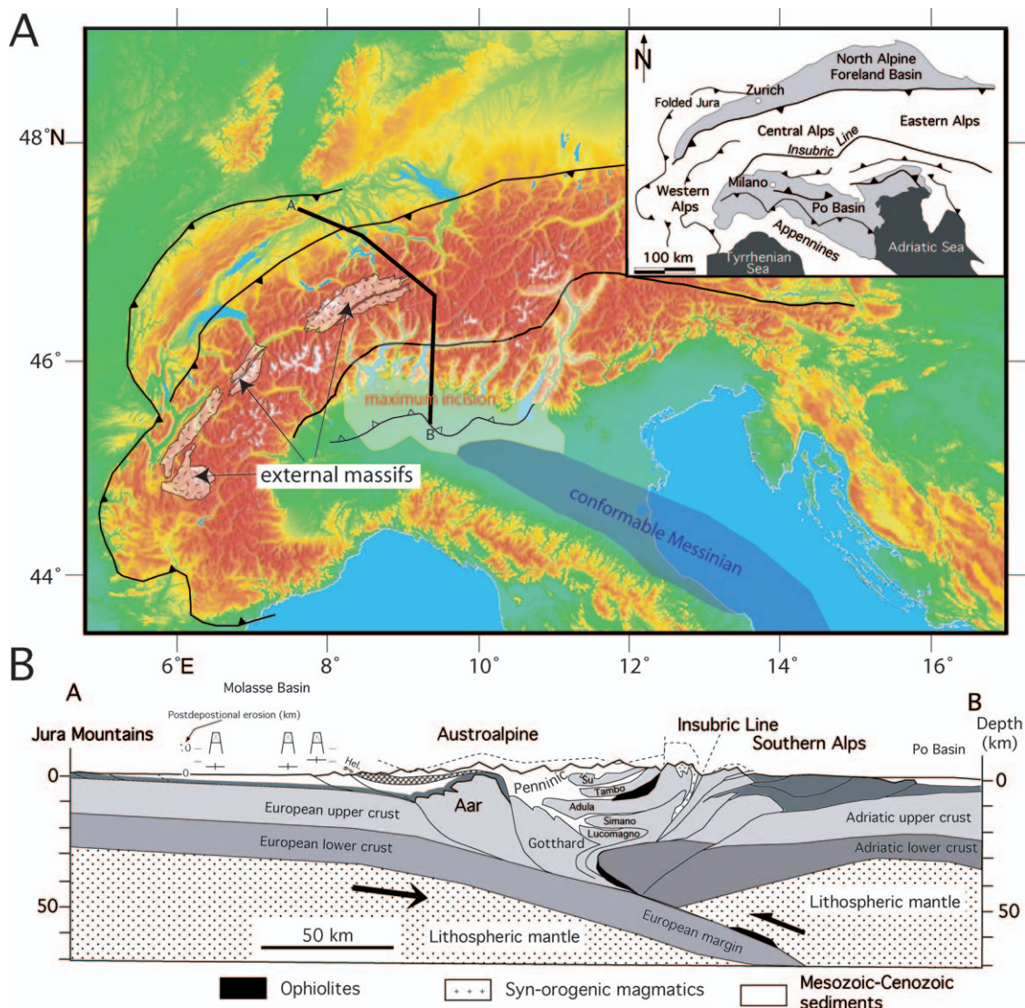
Figure 2. A: Topography and principle tectonic features of Alps. Documented region of Messinian erosion is indicated by shading. Western limit of region is poorly documented; erosion may continue into western Alps. Region of late Messinian deposition is indicated as conformable. B: Cross section of Alps showing major tectonic units. Modified from Pfiffner et al. (2002); erosion estimates in Molasse Basin are from Cederbom et al. (2004).
