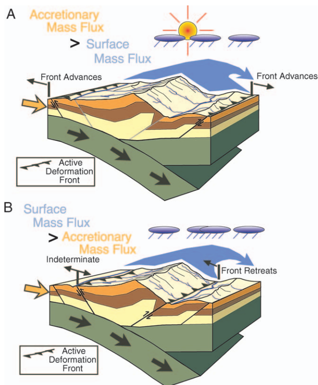
Figure 1. Constructive (A) and destructive (B) states of orogen, based on relative magnitude of accretionary flux, driven by convergence and erosional flux. Note difference in motion of deformation front relative to foreland.
