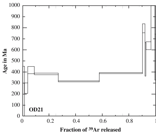
Fig. 6 ^{40}\text{Ar}/^{39}\text{Ar} analysis for the amphibolite OD21 were performed at Geochronology Laboratory at University of Alaska Fairbanks (for details, it is referred to Layer et al. 1987)
