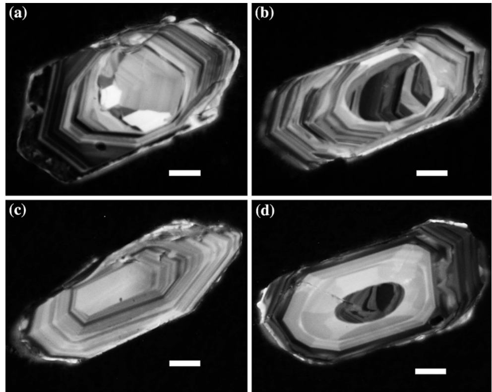
Fig. 3 SEM cathodoluminescence images showing internal growth patterns of typical zircons. a, b Sample BS3, Barenle orthogneiss, Prijakt Area; c, d Sample P1, Anras metaporphryoid, Thurmtal Complex; Scale bars 30 \mu m
