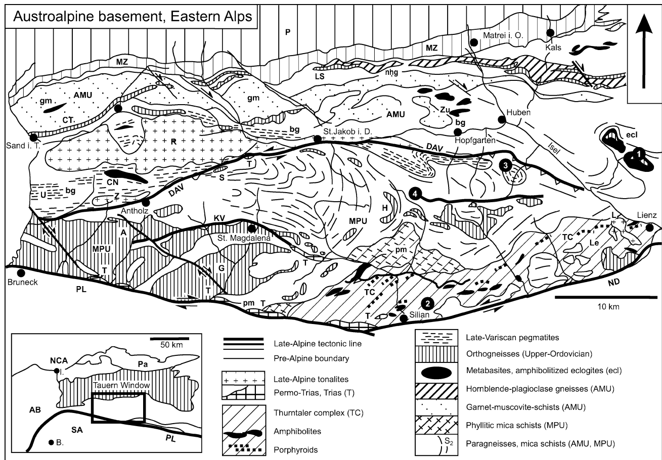
Fig. 1 Geological units in the basement to the south of the Tauern Window, Eastern Alps (after Schulz et al. 2001). Encircled numbers 1–4 refer to sampling locations of the presented isotope data. 1 Sample BS1 (Lake Barenle orthogneiss); 2 Sample P1 (Anras metaporphryoid); 3 Samples ST2-1 and ST2-2 (Lake Stierbichl staurolite- and staurolite-kyanite-schists); 4 Sample OD21 (amphibolite, MPU); A orthogneiss of Antholz; AB Austroalpine basement; AMU metapelite-amphibolite-marble unit (Durreck muscovite-schist and Northern Deferegggen Petzek Group); bg biotite gneisses; CT orthogneiss of Sand i. T. (Campo Tures); CN metabasites of Corda Nera; DAV Deferegggen-Antholz-Vals line; ecl amphibolitized eclogites of the Schober Group (Prijsakt Subgroup); G orthogneiss of Gsies
