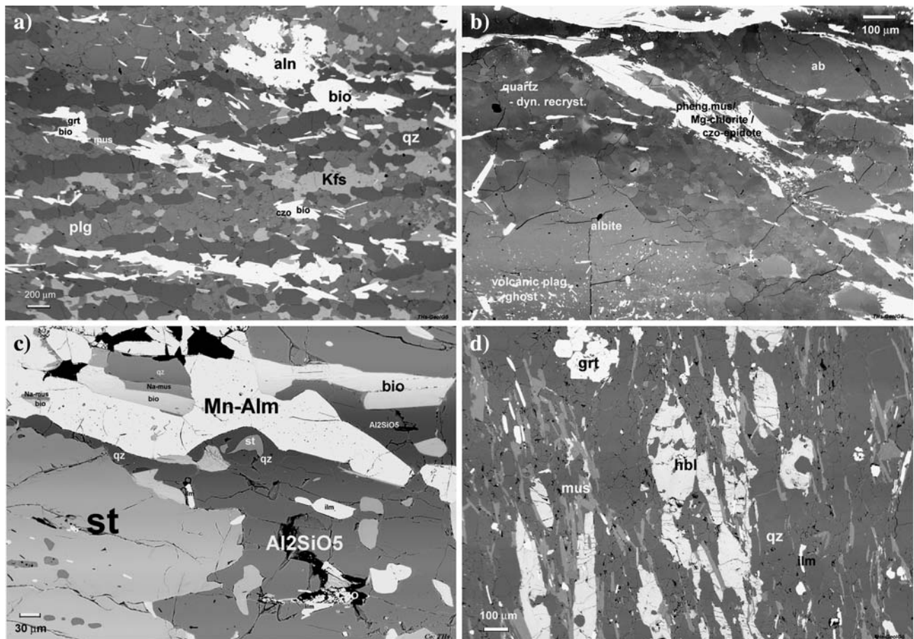
Fig. 2 Microstructures and petrography of selected samples, BSE images. a Sample BS3; orthogneiss, from one of a number of bands intercalated in the eclogitic amphibolite association, Barenle cirque, Prijakt, Hochschöber; aln allanite, kfs microcline, plg oligoclase, qz quartz, grt almandine, czo clinozoisite, mus white mica, bio biotite; frequent accessories not shown: apatite, zircon; macroscopic foliation s_1 results from ribbons and lenses of two-feldspar and quartz polycrystals with biotite; s_1 is cut at an acute angle by a younger foliation of biotite, clinozoisite, and muscovite. b Sample P1; Metaporphyrroid, Thurntaler Complex, forestry road cut ca. 1 km N of the church of Anras/Pustertal, the so-called “Feldspat-Blastengneis”, a metarhyolite with particularly coarse feldspars, consisting of ca. 30% vol of mm-sized feldspar clasts dispersed with little dimensional orientation in a finely laminated dark matrix; image shows detail from the margin of a feldspar clast, a phenocryst ghost of albite with inclusions of phengite, clinozoisite, small zircon, surrounded by a foliated matrix of recrystallized quartz, phengitic muscovite, chlorite, clinozoisite, albite plus accessory
