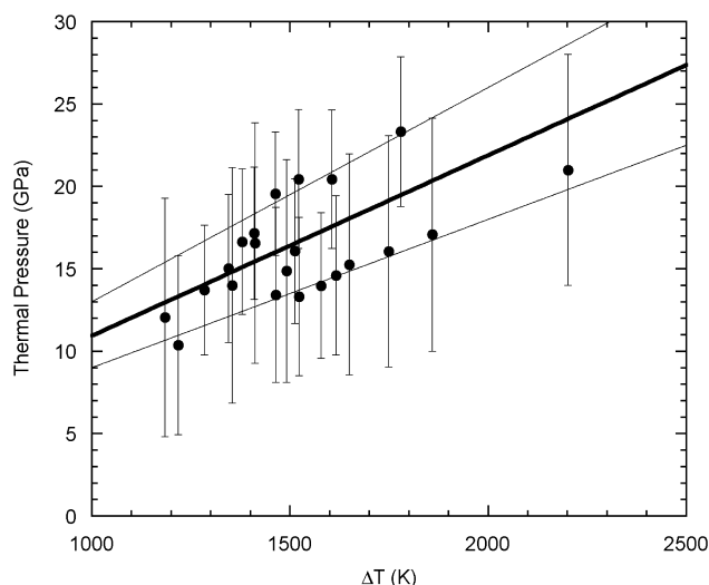
Figure 3. \text{Fe}_3\text{S} thermal pressure. P_{\text{thermal}} = \alpha K_T \Delta T , where \Delta T = (T - 300 \text{ K}) . Thick solid line, best fit \alpha K_T = 0.011(2) \text{ GPa K}^{-1} ; thin solid lines, one sigma error.
