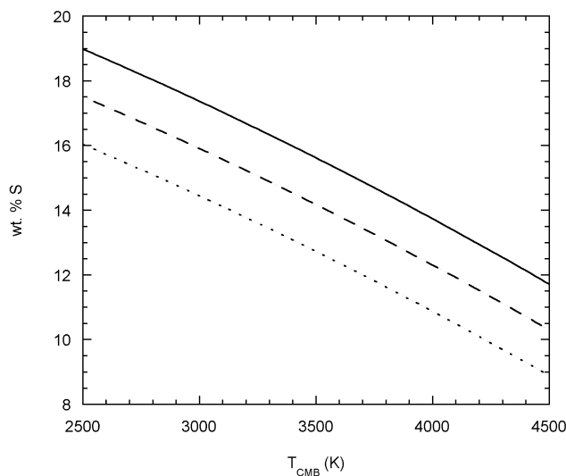
Figure 6. Weight percent sulfur required to resolve the density deficit of the outer core as a function of the temperature at the core mantle boundary. Solid line, \Delta V = 1\% ; dashed line, \Delta V = 2\% ; dotted line, \Delta V = 3\% . The relative uncertainty for a given point is \sim 7.5\% relative, based solely on the uncertainty of the density of \text{Fe}_3\text{S} . See the text for procedure of determining these curves.
