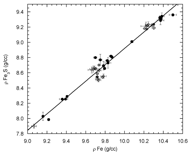
Figure 4. Density comparison between \text{Fe}_3\text{S} and Fe. Open diamonds, data at high temperature; solid circles, data at room temperature; solid line, best fit to the data. The data follow a linear relationship independent of temperature. The best fit yielded \rho(\text{Fe}_3\text{S}) = -1.832(\text{g cm}^{-3}) + 1.075 * \rho(\text{Fe}) , with root mean square 0.069 \text{ g cm}^{-3} .
