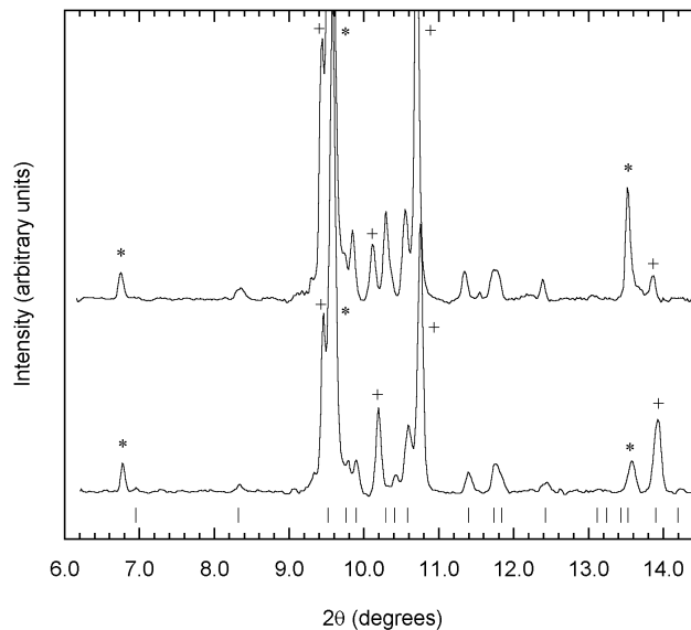
Figure 1. Typical diffraction patterns collected in this study with background subtracted. The patterns clearly show the coexistence of Fe and Fe 3 S at simultaneous high pressure and temperature. Top pattern, P = 79.4(19) GPa, T = 2150 K; bottom pattern, after rapid quenching P = 74.9(7) GPa, \lambda = 0.3344 Å. Stars, NaCl B2 reflections; crosses, hcp-Fe reflections; tick marks, all Fe 3 S reflections allowed by symmetry based on the lattice parameters a = 8.306(6) Å and c = 4.104(5) Å determined from the quenched pattern. The small peak at \sim 11.5^\circ in the high-temperature pattern remains unidentified.
