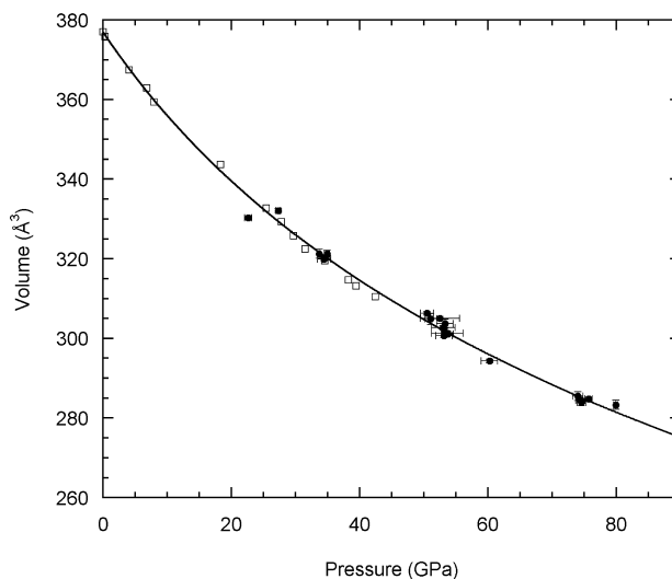
Figure 2. Fe 3 S compression curve at T = 300 K. Solid circle, this study; open square, Fei et al. [2000]; solid line, best fit to our data, K_0 = 156(7) GPa, K'_0 = 3.8(3) .
