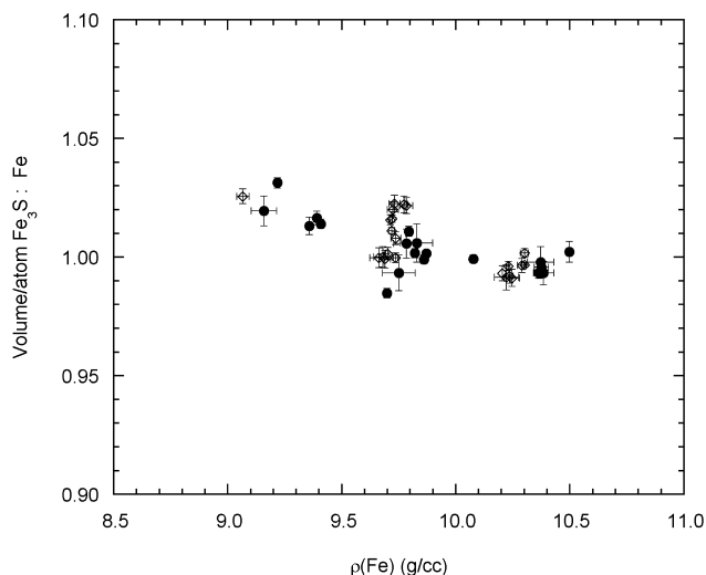
Figure 5. Volume per atom of \text{Fe}_3\text{S}:\text{Fe} . Open diamonds, data at high temperature; solid circles, data at room temperature. Sulfur has the effect of decreasing the average volume per atom relative to pure iron above \sim 50 GPa.
