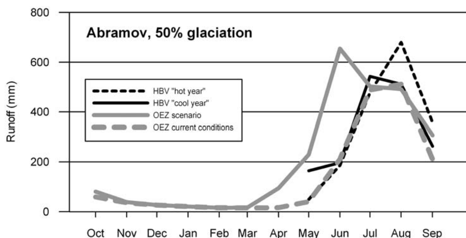
Figure 8 Runoff scenarios of HBV and OEZ hydrological models for Abramov catchment after doubling of \text{CO}_2 , as predicted by the GISS model (KazNIIMOSK, 1999) and for 50% of current glaciation. HBV scenarios were produced for a cool and a hot reference year, the OEZ scenario is based on mean climatological conditions of the simulated period (8 years).
