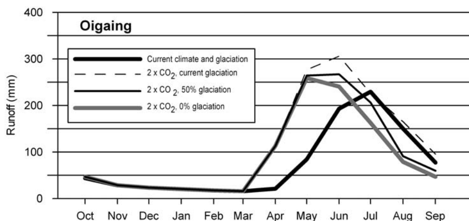
Figure 3 OEZ model results at Oigaing for current climate and for the doubling of \text{CO}_2 in combination with two steps of deglaciation as mean values over the simulated period (8 years).
