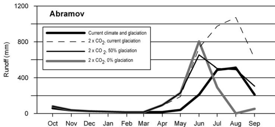
Figure 5 OEZ model results at Abramov for current climate and for the doubling of \text{CO}_2 in combination with two steps of deglaciation as mean values over the simulated period (20 years).
