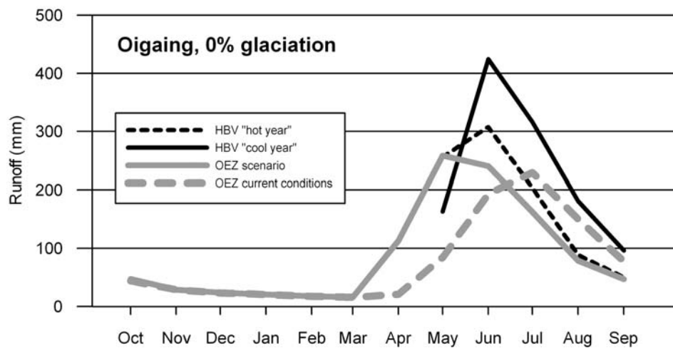
Figure 9 Runoff scenarios of HBV and OEZ hydrological models for Oigaing catchment after doubling of CO 2 , as predicted by the GISS model (KazNIIMOSK, 1999) and for a complete loss of glaciation. HBV scenarios were produced for a cool and a hot reference year, the OEZ scenario is based on mean climatological conditions of the simulated period (8 years).
