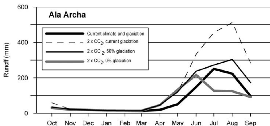
Figure 4 OEZ model results at Ala Archa for current climate and for the doubling of \text{CO}_2 in combination with two steps of deglaciation as mean values over the simulated period (8 years).
