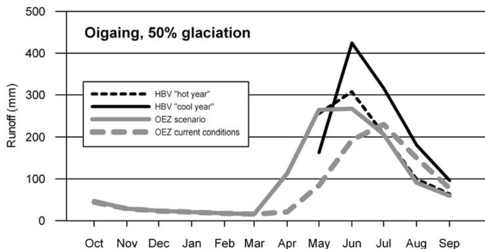
Figure 6 Runoff scenarios of HBV and OEZ hydrological models for Oigaing catchment after doubling of \text{CO}_2 , as predicted by the GISS model (KazNIIMOSK, 1999) and for 50% of current glaciation. HBV scenarios were produced for a cool and a hot reference year, the OEZ scenario is based on mean climatological conditions of the simulated period (8 years).
