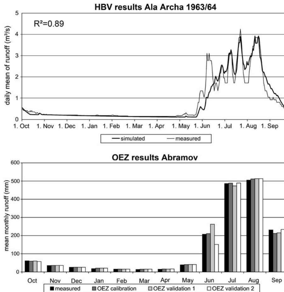
Figure 2 Example hydrographs generated by HBV and OEZ models in comparison to measured runoff (OEZ calibration period: 1968/69–1987/88, validation 1: 1968/69–1977/78, validation 2: 1978/79–1987/88).
