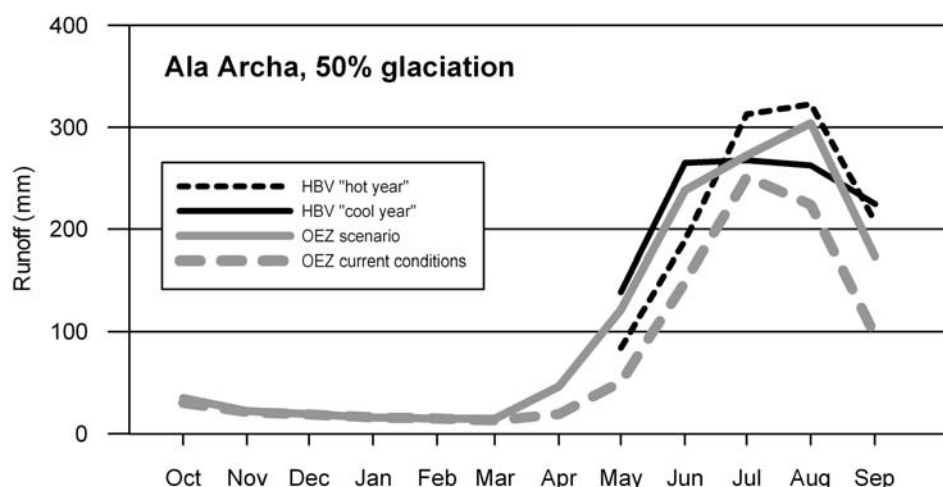
Figure 7 Runoff scenarios of HBV and OEZ hydrological models for Ala Archa catchment after doubling of \text{CO}_2 , as predicted by the GISS model (KazNIIMOSK, 1999) and for 50% of current glaciation. HBV scenarios were produced for a cool and a hot reference year, the OEZ scenario is based on mean climatological conditions of the simulated period (8 years).
