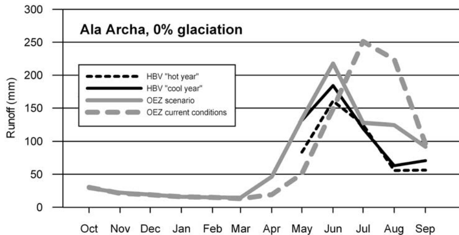
Figure 10 Runoff scenarios of HBV and OEZ hydrological models for Ala Archa catchment after doubling of CO 2 , as predicted by the GISS model (KazNIIMOSK, 1999) and for a complete loss of glaciation. HBV scenarios were produced for a cool and a hot reference year, the OEZ scenario is based on mean climatological conditions of the simulated period (8 years).
