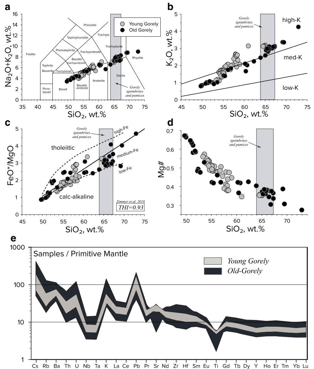
Fig. 3 Gorely sample classifications: a total alkali versus silica ( TAS ) diagram (Le Bas et al. 1986); b K_2O versus SiO_2 , showing that Gorely rocks belong to the medium-K and high-K types (Le Maitre et al. 1989); c SiO_2 versus FeO/MgO ratio with subdivision lines which are after Miyashiro (1974) and Arculus (2003), Tholeiitic Index ( THI ) was calculated using the method of Zimmer et al. (2010). d SiO_2 versus Mg\# illustrates the ranges of SiO_2 and Mg\# for Gorely volcano rocks. e Trace element patterns on selected Gorely samples (ICP-MS analysis only), samples normalized using values from Sun and McDonough (1989). Light gray bar at (a), (b), (c), and (d) demonstrates the range of compositions of caldera-forming eruptions (ignimbrites and pumices)
