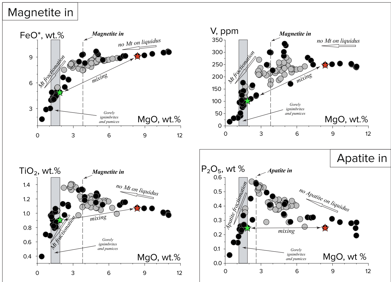
Fig. 5 Interpretation of expected fractional crystallization processes for Old Gorely volcanics (black circles): appearance of accessory minerals. The onset of magnetite crystallization at MgO is \sim 3.8 wt% ( \text{SiO}_2 \sim 55 wt%) illustrated by FeO, \text{TiO}_2 , and V versus MgO diagrams, and
