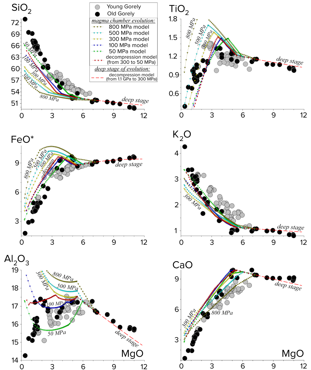
Fig. 16 Several illustrative plots with modeling results compared with actual WR data. Red dashed line demonstrates deep decomposition (from 1.1 GPa to 300 MPa) and Ol + Sp fractionation. Different colored lines with triangles are the models of magma chamber FC at different pressures (from 50 to 800 MPa)
