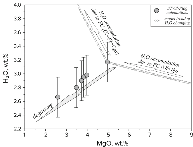
Fig. 17 Old Gorely magma H_2O content variations during magma evolution. H_2O behaves as an incompatible element and should accumulate in the magma during fractional crystallization ( thin model line with small white circles ). However, \Delta T Ol-Plag calculations (after Danyushevsky 2001) for compositions of aphyric/subaphyric Old Gorely rocks ( large gray circles ) demonstrate a water loss (degassing) trend. The \Delta T Ol-Plag calculations were made for the following samples: OG-14, OG-71, OG-73, OG-6A, OG-64
