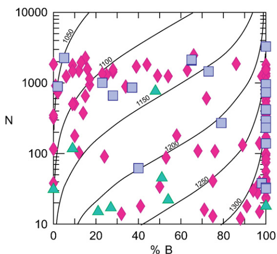
Fig. 9. Nitrogen contents and aggregation states (relative proportion of nitrogen in B-center) for diamonds from K11 (triangles), K91 (squares) and K252 (diamonds). Solid lines are isotherms (°C) for a mantle residence time of 1 Ga (after Taylor et al., 1990).
