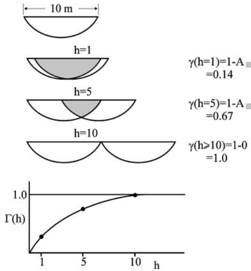
Figure 2. An example geometric object and the resulting geometric semivariogram in the horizontal direction. The semivariogram model is anisotropic.
