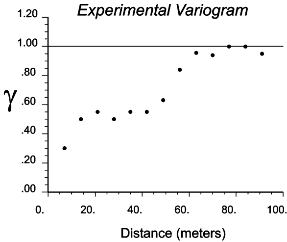
Figure 1. An example semivariogram that is not well fit by nested sets of traditional variogram models.
