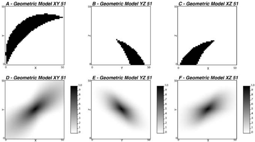
Figure 6. Center slices through the raster geometric object and the resulting covariance table for a possible IHS point bar variogram.
