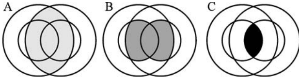
Figure 4. Volumes v_1 , v_2 , and v_3 (A, B, and C): a traditional spherical variogram model is equal to standardized v_1 subtracted from the contribution. The hollowed sphere model is equal to the spherical minus v_2 plus v_3 .
