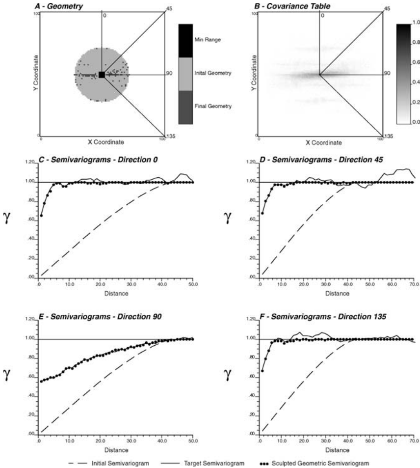
Figure 10. A 2-D geometry and covariance table for a sculpted geometric semivariogram model based on a phenomenon with high anisotropy and large nugget effect. The initial geometry, the target directional models and resulting sculpted geometric semivariogram models in 0°, 45°, 90° and 135° directions are shown. The target models are experimental semivariograms from unconditional sequential Gaussian simulation.
