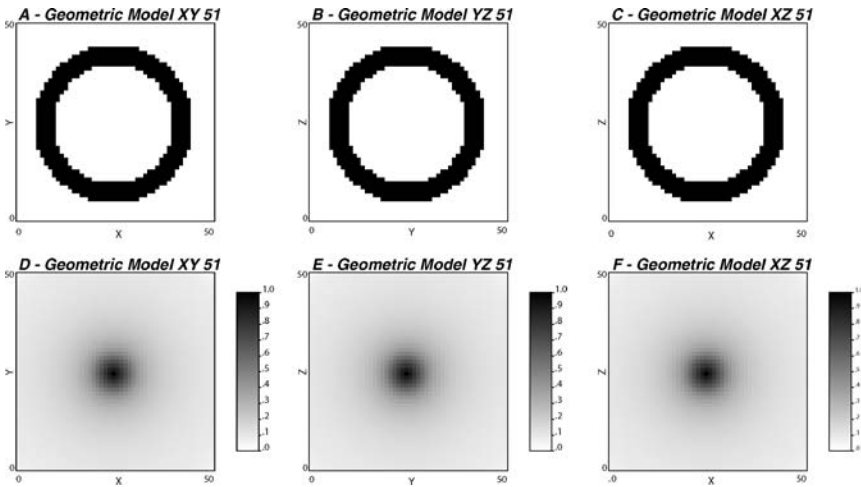
Figure 5. Center slices through the rasterized geometric object and the resulting covariance table for the hollow spherical model with a hollowed fraction of 0.75.
