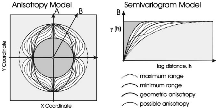
Figure 8. The constraints on sculpted geometric semivariogram models. The major and minor principal directions (directions A and B respectively) and the traditional anisotropy ellipsoid are shown. The sculpted semivariogram model is constrained such that the range in the off-diagonal directions (such as direction B) may not exceed the range in the major direction or be exceeded by the range in the minor direction. The anisotropy may be expressed in various forms within this constraint.
