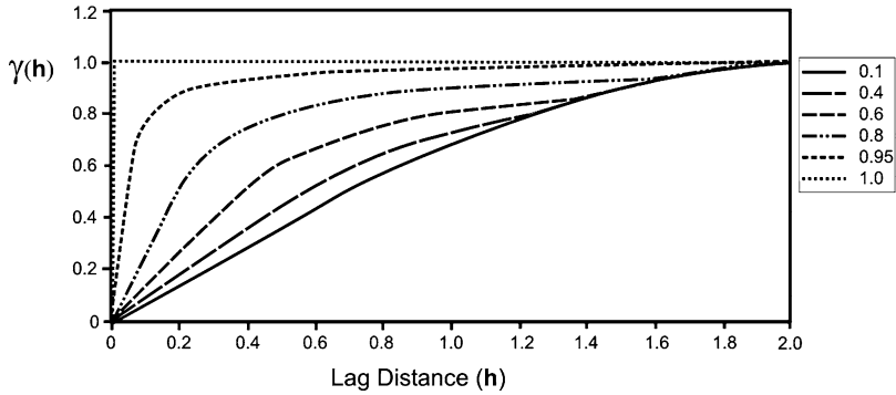
Figure 3. A series of hollowed sphere semivariogram models. The sphere radius, r_2 , is set to 1.0 and the radius of the hollowing is varied.
