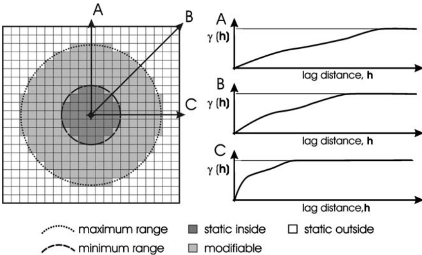
Figure 7. An initial 2-D geometry based on fit semivariograms in three directions. The area outside a circular geometry with a diameter equal to the longest identified range (direction A) is set as permanently outside the geometry. A circular geometry with a diameter equal to the shortest identified range (direction C) is set as permanently inside the geometry. The remainder may be modified iteratively to fit the semivariograms in each identified direction.
