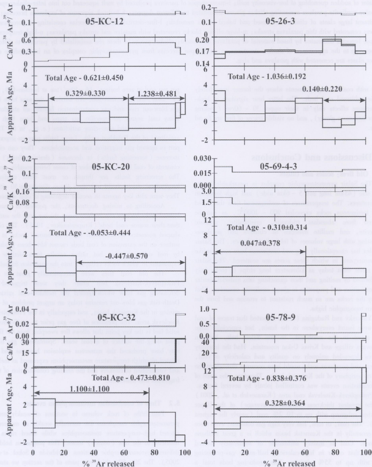
Fig. 4 ^{40}\text{Ar}/^{39}\text{Ar} ages of pyrometamorphic rocks from the Salair combustion metamorphic complex
