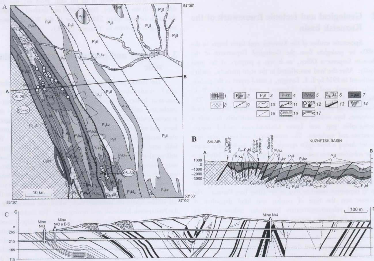
Fig. 2 A. Generalized geology of Prokopyevsk-Kiselevsk area of Salair deformation zone, with sampling sites in pyrometamorphic complexes. B) Geological cross section along line A-B; C) Detailed cross section along line C-D (after Krupennikov, 1935). 1-fluvial deposits in river valleys, 2-Erunak subgroup, 3-Ilyinka subgroup, 4-Kuznetsk subgroup, 5-Upper Balakhon subgroup, 6-Lower Balakhon subgroup, 7-Ostrog Formation, 8-basement rocks of Kuznetsk basin, 9-main faults, 10-towns and villages, 11-geological profiles, 12-examined outcrops (a) and sampling sites for dating (b). Symbols in cross section C-D: 13-coal seams and their names, 14-pyrometamorphic complexes, 15-faults, 16-mines, 17-overburden
