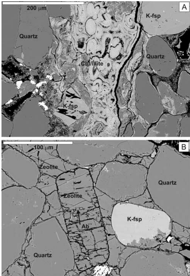
Fig. 8. SEM backscatter images from Clarens Formation sandstone surrounding the Witkop III complex. (a) Possible volcanic material (glass) now altered to chlorite and illite. The texture differs from anything seen in the sediment breccia from the hydrothermal vent complexes. (b) Zeolite-cemented Clarens sandstone (from the upper part of the uppermost dune unit in Fig. 6b). The absence of other authigenic minerals (indicating early zeolite precipitation), and that the zeolite forms pseudomorphs after feldspar (albite), should be noted.
