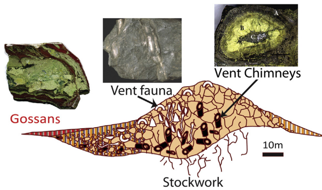
Fig. 2. Schematic cross-section across the Yaman-Kasy deposit (modified from Maslennikov et al., 2009). The fragment of hydrothermal chimney, vent fauna and clastic ore breccia with surrounding gossans are shown. Chimney consists of: A - outer pyrite-marcasite wall; B - inner chalcopyrite wall; C - pyrite-marcasite-sphalerite core.
