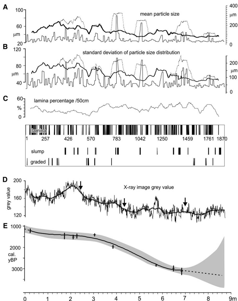
Fig. 3. Sedimentary data and age model of the Alison Sound core VEC02A07. A: Solid line: mean particle sizes of 155 samples; dotted line 50/5 cm moving average of mean particle size; bold line: 50/5-cm moving average of mean particle size after removal of data from slumps; scale on right: raw data, scale on left: smoothed data. B: Solid line: standard deviation (1 s) of particle size distribution of 155 samples; dotted line 50/5 cm moving average of 1 s of particle size distribution; bold line: 50/5-cm moving average of 1 s of particle sizes distribution after removal of data from slumps; scale on right: raw data, scale on left: smoothed data. C: Top: lamina percentage per 50 cm sliding window of total sediment, below: location of all lamina with total lamina count at 1 m intervals, slumps and graded sediment in core; remaining empty space marks homogenous (massive) intervals. Note that lamina concentration appears over represented due to the thickness of the lines. D: X-ray image grey value time series (solid line) and 50/0.25 cm moving average (bold line). Arrows mark intervals with >4 cm of lost core. E: Age–depth model: solid line: 4th degree polynomials; grey shaded area: 95% confidence interval of 4th degree polynomials; crosses: location of ^{14}\text{C} calibrated ages with \pm 95\% confidence intervals.
