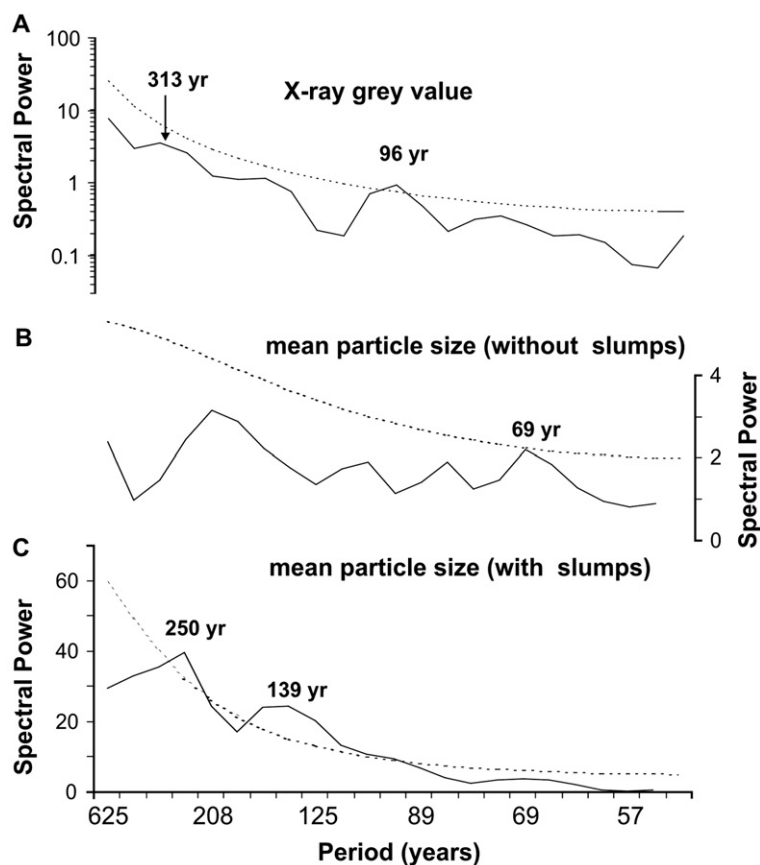
Fig. 7. Spectral power (3-frequency Hanning–Tuckey window, average of two spectra of two 1250-yr sequences each at 25 year sample-intervals); A: X-ray image grey value time series; B: mean particle size with replacement of slumps by interpolated data (135 raw data) time series; C: mean particle size time series from 155 raw data; dashed line mark 95% confidence level for red noise (after Mann and Lees, 1996).
