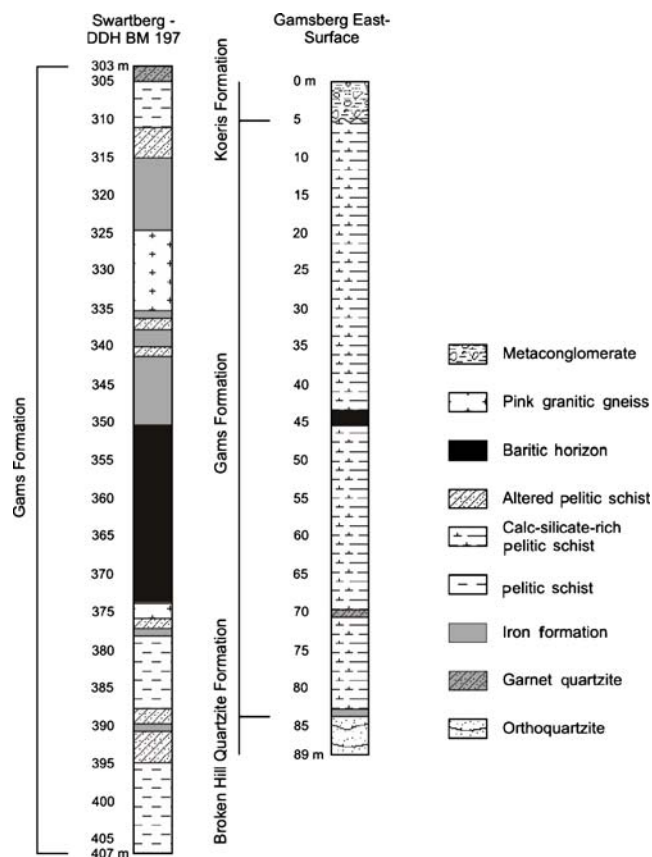
Fig. 4 Detailed section through the Gams Formation at Swartberg and Gamsberg illustrating the location of the barite beds. Note the close spatial association between the barite and iron formation at Swartberg compared to the distal relationship at Gamsberg. Note that the graphite schist was not observed in the stratigraphic section at Gamsberg
