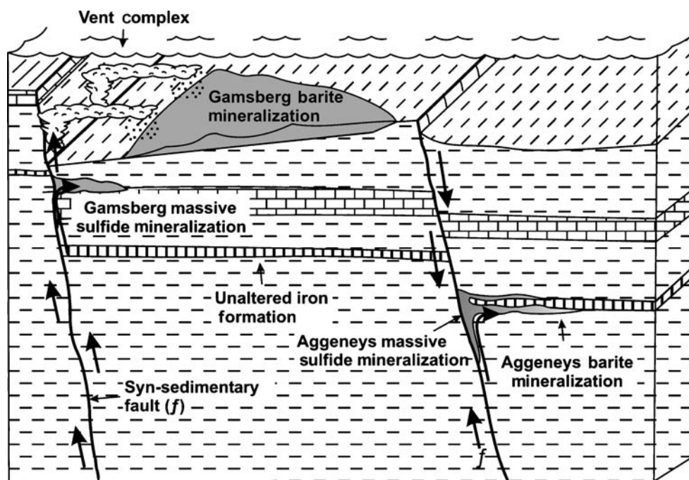
Fig. 7 Schematic diagram illustrating the formation of stratiform and stratabound barite and associated massive sulfides via sub-seafloor replacement of an iron-formation in the Aggeneys deposits, and seafloor exhalation in the Gamsberg deposit. Both deposit styles are related to mixing of an upwelling metal-liferous hydrothermal fluid and downward moving sulfate-rich seawater. Modified from Robb (2005)
