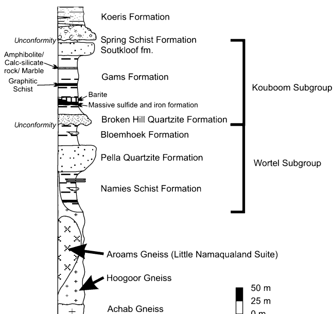
Fig. 2 Generalized stratigraphic column for the Bushmanland Group in and around the Aggeneys-Gamsberg Broken Hill-type Pb–Zn–Cu–Ag–Ba district
