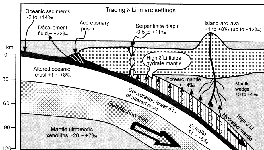
FIG. 3. Schematic illustration of Li isotope systematics in a subduction-zone setting, modified from Zack et al. (2003). Heavy Li in fluids from the décollement zone and serpentinite diapiers reflect Li isotopic fractionation during the dehydration of altered oceanic crust. The high \delta^7\text{Li} of fluids escaping the slab at low temperatures likely enrich the forearc mantle wedge and hydrate the adjacent mantle in ^7\text{Li} , which may be the sources of arc lavas. Thus, high \delta^7\text{Li} values in arc lavas (up to +12‰) might be explained by incorporation of the forearc mantle. Data sources are the same as those identified in Figure 1.
