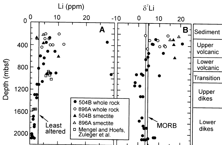
FIG. 4. Variation of Li concentration (A) and isotopic ratios (B) with depth for whole rocks and smectites from DSDP/ODP Sites 504B and 896A, shown with lithologic sections from Chan et al. (2002a). Also shown are concentration data for the transition zone from Mengel and Hoefs (1990) and at 1570 mbsf from Zuleger et al. (1996).
