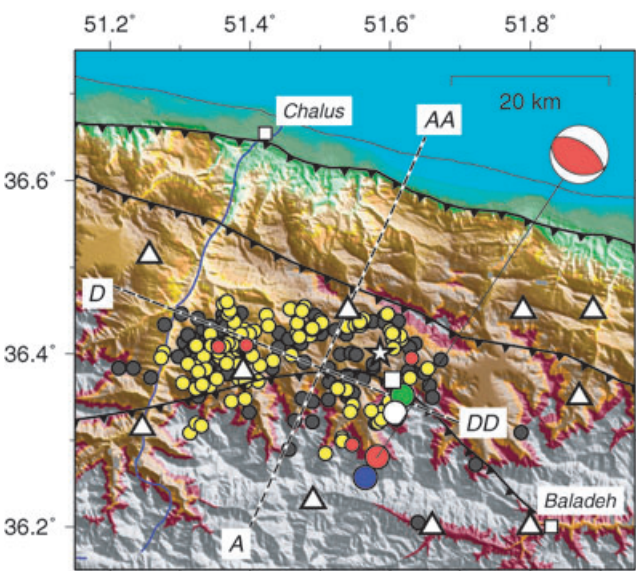
Figure 6. The epicentral area of the 2004 Baladeh earthquake (the white box in Fig. 2), showing the high-quality aftershock locations (group A) in yellow, and lower-quality locations (group B) in gray. White triangles are temporary seismograph stations, and the white star is the strong-motion instrument at Poul (Kojour). Mainshock epicentre estimates are the large circles in blue (from the catalogue of Engdahl et al. 2006), green (from the Institute of Geophysics at Tehran University), red (from the HDC cluster analysis reported here, and white from P (square) or P and S (circle) arrival times at regional Iranian stations: see Table 1. The smaller red circles are four aftershocks that were also located by HDC cluster analysis. The formal uncertainties in the yellow and red epicentres are about twice the size of their respective circles. The red focal sphere is that of the mainshock, as in Fig. 2. The faults shown are the Khazar (north), North Alborz (middle) and Kojour (south): see Fig. 2. A-AA and D-DD are the lines of the cross-sections shown in Fig. 7.
