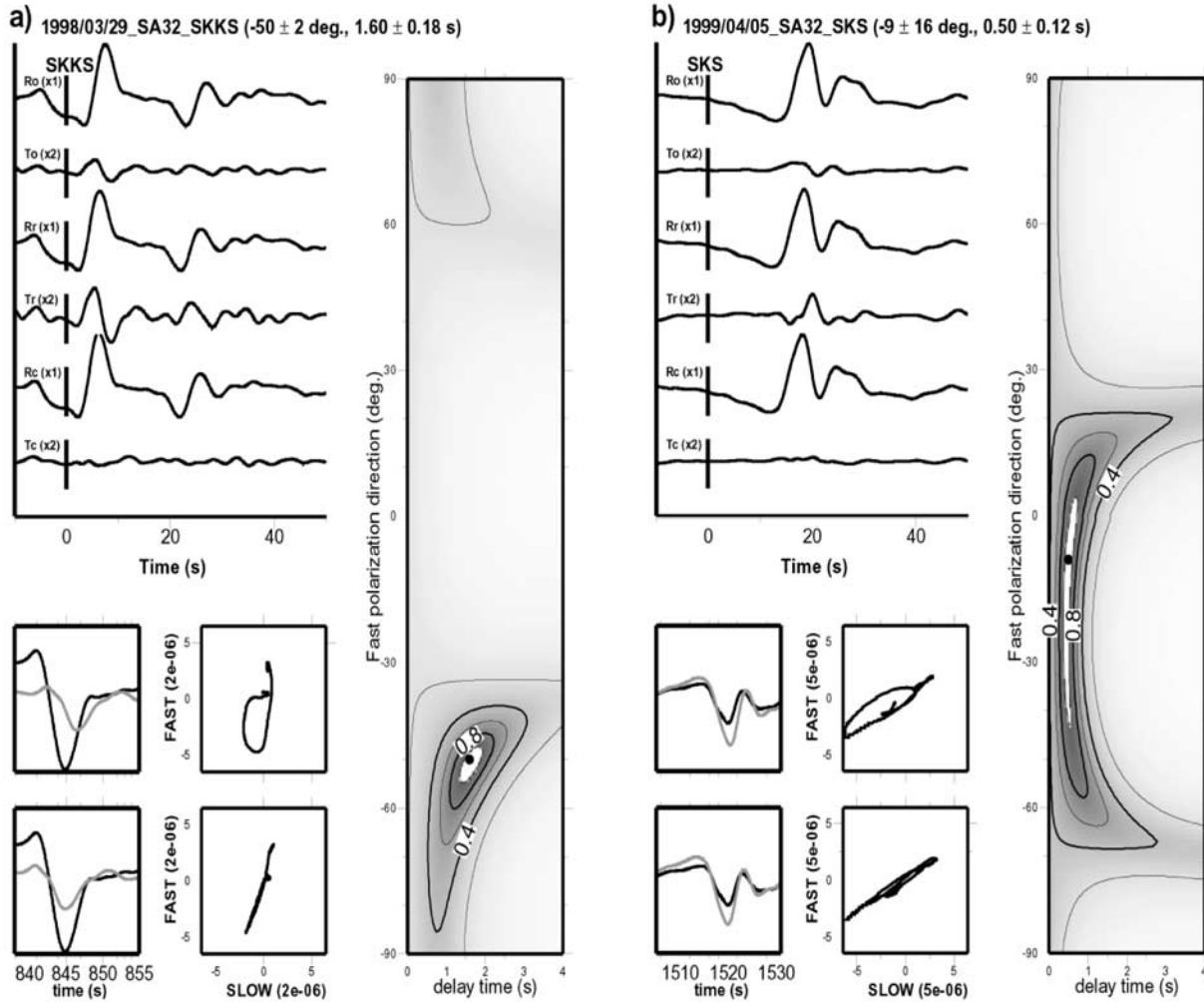
Figure 6. Examples of waveform splitting analyses of the lowermost mantle anisotropy for (a) SKKS of event 1998/03/29 (event 3 in Figure 4a) and (b) SKS of event 1999/04/05 (event 5 in Figure 4a) recorded by station SA32. Figures 6a and 6b are labeled by event_date_station_phase (fast polarization direction \pm 1 sigma error in degree, delay time \pm 1 sigma error in second). (top left) For each example, the original radial (Ro) and tangential (To) displacements, the radial (Rr) and tangential (Tr) displacements of SKS or SKKS waves after corrected for the shallow mantle anisotropy beneath seismic station ( 52^\circ\text{N} , 1.10 s), the unsplit radial (Rc) and tangential (Tc) displacements of SKS or SKKS waves after further corrected for the anisotropy in the lowermost mantle. The vertical black lines show the predicted arrival time of SKS or SKKS based on model IASP 91 [Kennett and Engdahl, 1991]. (bottom left) Superposition of fast (black) and slow (gray) components, (middle left) uncorrected and (bottom left) corrected, and their corresponding horizontal particle motions (in millimeter), (middle right) uncorrected and (bottom right) corrected. (right) Contour plot of normalized energy on the corrected transverse component as a function of fast polarization direction and delay time. The solid black dot indicates the optimum fast polarization direction and delay time that minimize energy on the tangential component of SKS or SKKS waveforms, and the white area represents best fitting parameters at the 95% confidence level. The energy is normalized to that of the best fitting fast polarization direction and delay time at the 95% confidence level.
