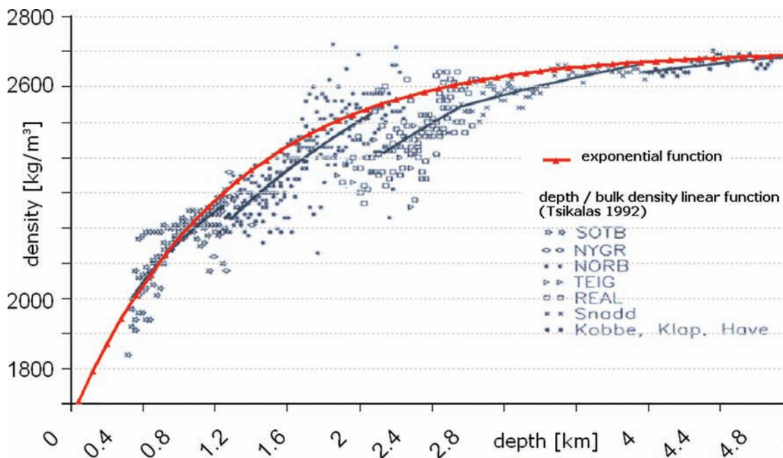
Figure 3. Density–depth function for sediments. We use an exponential function to describe the increased sediment density with depth. This function considers the effect of decreased porosity with depth. The density–depth function is adjusted to borehole measurements from Tsikalas (1992).
