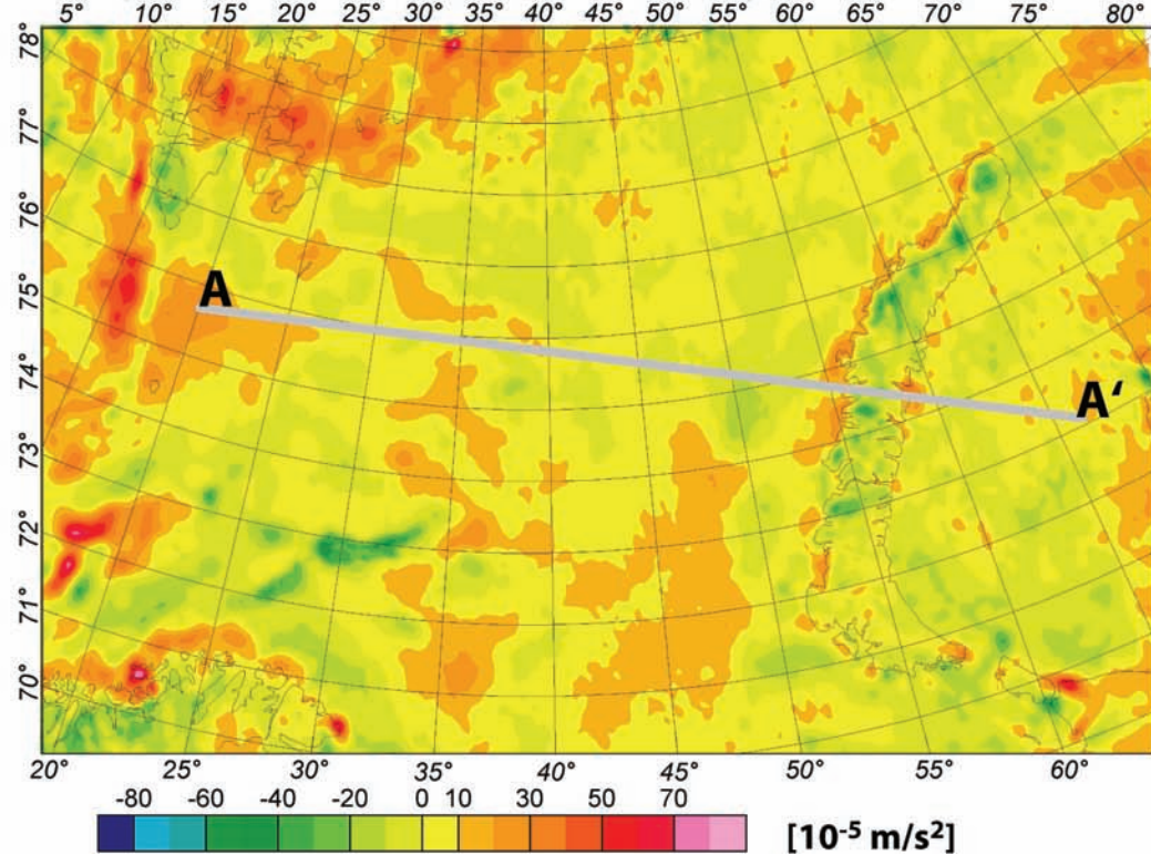
Figure 10. Maps showing residual gravity for the 3-D models. (a) Gravity residual for the model that includes only isostatic mantle densities and the intracrustal horizon in the computation. (b) Gravity residual for the model that also includes small lower-crustal density variations. The profile A–A' is plotted in Figs 9(a) and (b).
