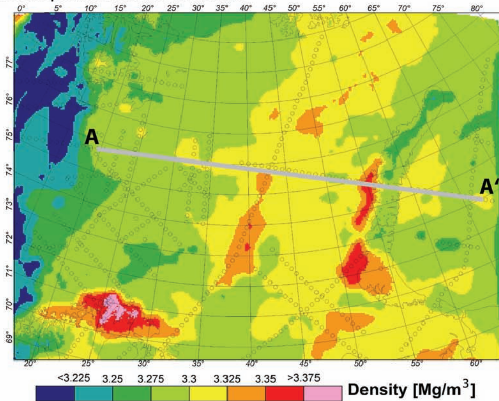
Figure 8. Maps showing (a) lower crustal density and (b) lithospheric mantle density variations. The varying densities allow local isostatic equilibrium to be achieved and give a modelled gravity field that fits the observed gravity to a large degree. The profile marked A–A' is plotted in Fig. 9. This profile shows the complete crustal structure.
