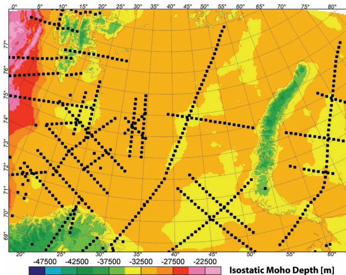
Figure 6. The simple Airy isostatic Moho depth (root) was calculated by taking into account the loading of bathymetry/topography and sediments as well as a density contrast between the lower crust and upper mantle of 400 \text{ kg m}^{-3} and a relative normal crustal thickness of 35 km (as for the reference model in Table 1).
