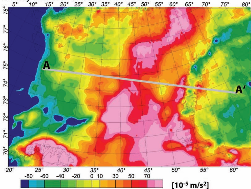
Figure 4. (a) Map showing the gravity effect of the simple 3-D density model based on constant densities for the crust and mantle, the density–depth relation for sediments from Fig. 3 and geometry from Fig. 2. (b) The residual field shows large regional differences between the gravity effect of the 3-D model and the observed Bouguer gravity (Fig. 1b). The profile marked A–A' is plotted in Fig. 5.
