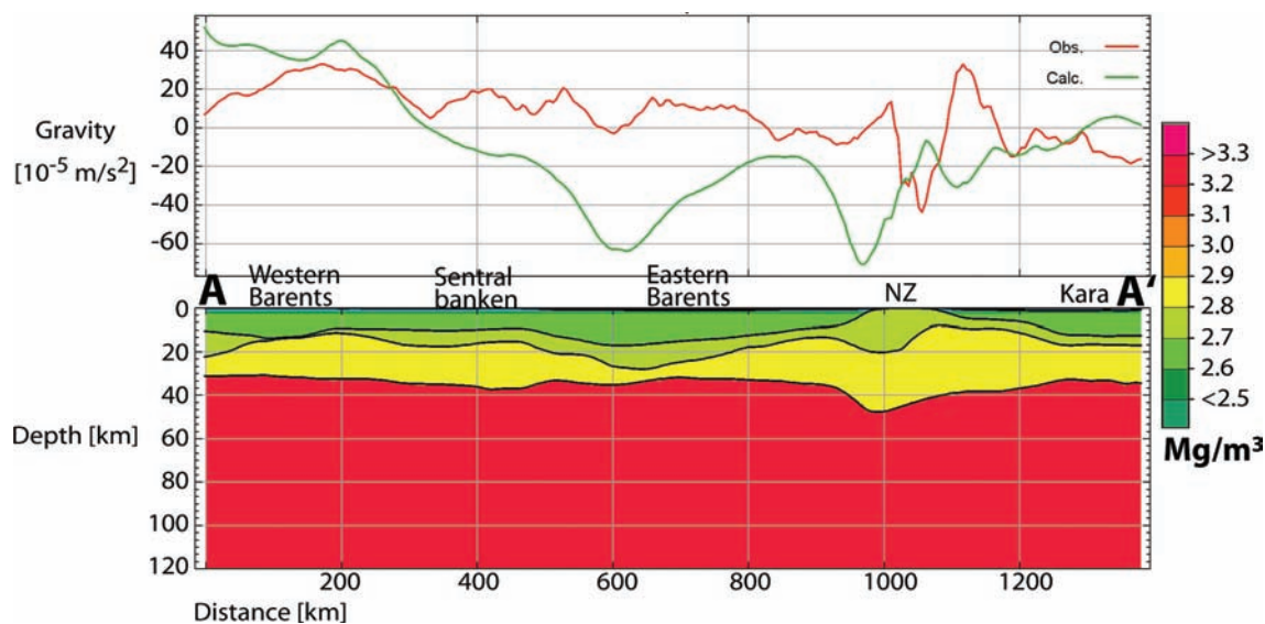
Figure 5. West-east profile through the model from the westernmost border of the Barents Sea to the Kara Sea showing the geometry and density distribution of the initial 3-D density model. The upper panel shows the large differences between the modelled gravity effect (green line) and the observed Bouguer anomaly (red line). For exact profile location and more details see Fig. 4.
