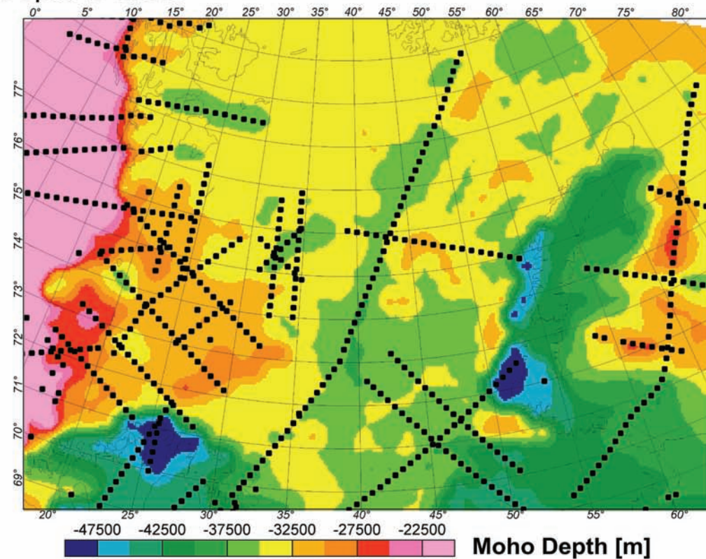
Figure 2. (a) Depth to basement and (b) Moho maps. The maps are adopted from the Barents50 model (Ritzmann et al. 2007) with modifications after Skilbrei (1991, 1995) for the Western Barents Sea. The black dotted lines denote the location of the regional seismic lines used in compiling the Barents50 model.
