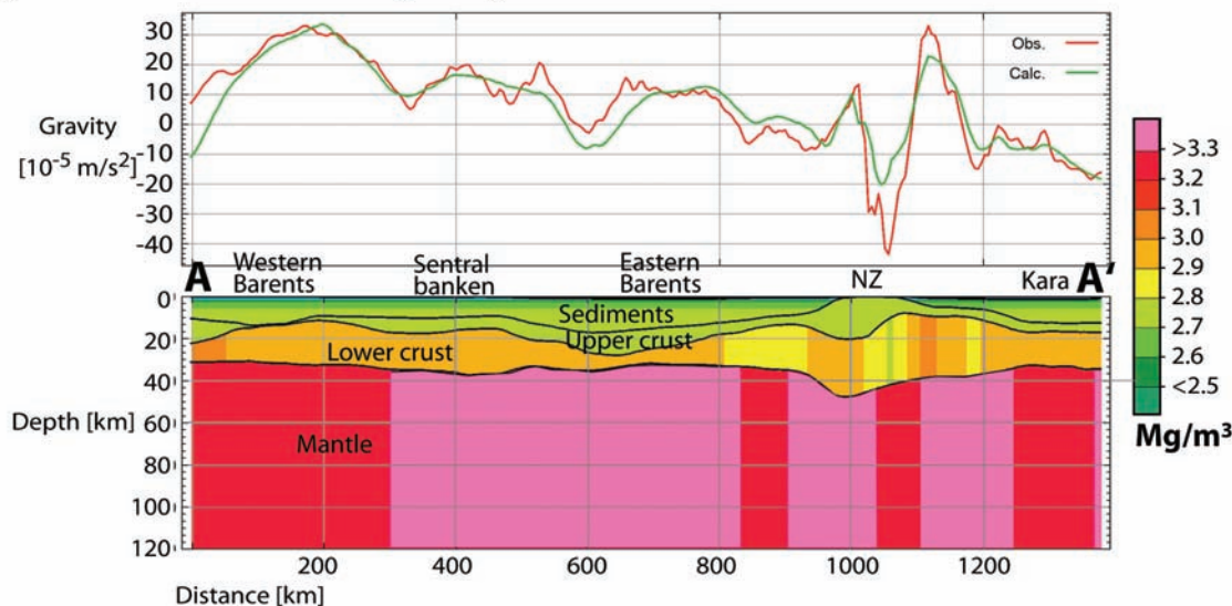
Figure 9. Profiles showing the same geometry as in Fig. 5, but in (a) the densities of the lithospheric mantle are varied to isostatically balance the lithosphere, and in (b) densities in the lower crust are also varied to fit the modelled and observed gravity fields whilst maintaining isostatic balance. The gravity residuals of the entire 3-D model are shown in Figs 10(a) and (b).
