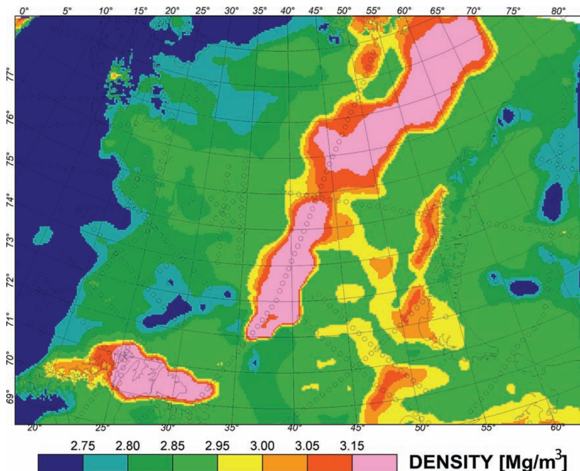
Figure 7. Map showing the distribution of isostatic crustal densities. The lower crustal densities were calculated to isostatically balance the lithosphere without including a variation in mantle densities.
