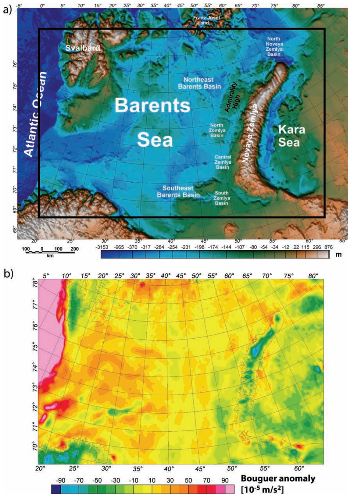
Figure 1. (a) Map showing topography/bathymetry of the greater Barents Sea Region, the location of the study area (black square) and the main structural elements. (b) Bouguer gravity anomaly map based on the gravity data from the Arctic Gravity Project (2002). The Bouguer anomaly is calculated with a complete ice-reduction and a Bouguer density of 2670 \text{ kg m}^{-3} .
