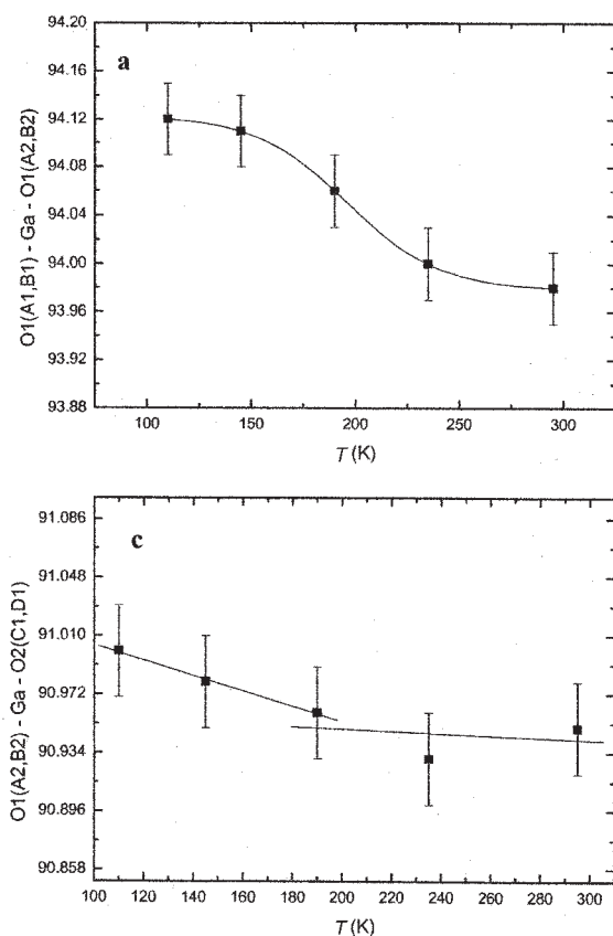
FIGURE 10. Evolution as a function of temperature of the three independent bond angles (a) O1(A1,B1)-Ga-O1(A2,B2), (b) O1(A1,B1)-Ga-O2(C1,D1), and (c) O1(A2,B2)-Ga-O2(C1,D1) for NaGaSi 2 O 6 .
