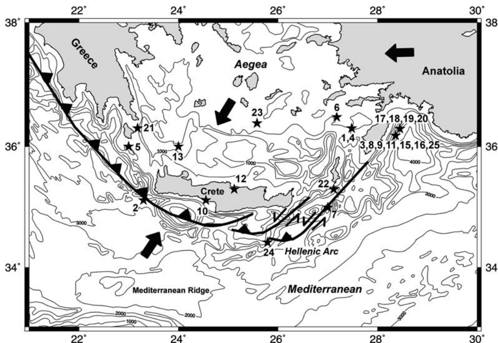
Fig. 5. Reported locations of tsunamigenic earthquakes along the Hellenic arc and trench system (Papadopoulos 2001; Papadopoulos et al. 2007). Large black arrows show relative motions of plates with respect to Eurasia (McClusky et al. 2000, 2003). Bathymetric contours are shown at 500 m interval, and are from GEBCO (1997). Major plate boundaries are as shown in Figure 1. Numbers refer to tsunamigenic events in Table A3.
