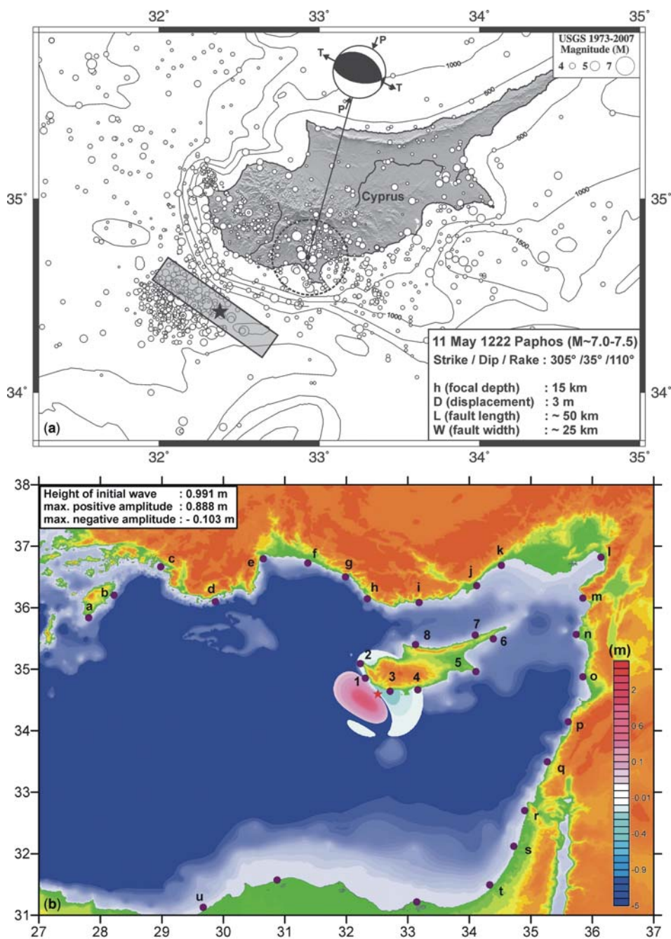
Fig. 7. (a) Seismicity of the Cyprus arc and surroundings as in Figure 6. Box with star refers to approximate location of the 11 May 1222 Paphos earthquake (M ~ 7.5) and tsunami, for which simulations are generated by applying an analogous representative earthquake derived from teleseismic P- and SH-wave modelling studies of current earthquakes. The parameters of tsunami simulations are shown in the box in the lower right corner, and a representative fault-plane solution obtained from current earthquake source mechanisms is shown above in a lower hemisphere projection. (b) Snapshot of the initial tsunami generated with the parameters given in (a). Letters and numbers refer to geographical locations where macroseismic observations have been partly reported (Guidoboni & Comastri 2005a), and synthetic tsunami mareograms generated at pseudo-tide-gauge locations, and details are shown in Figure 8a and b.
