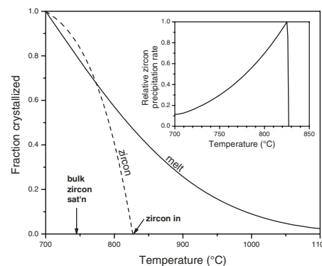
Figure 3. Assumed crystallization sequence for intermediate granitoid magma cooling from 1100 °C (solid curve). The cumulative growth of zircon growth (dashed line) indicates onset of zircon crystallization at 827 °C, or ~80 °C hotter than the calculated zircon saturation temperature. Zircon growth rate shown in the inset.
