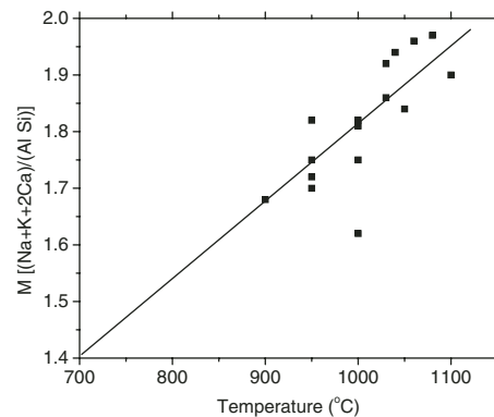
Figure 2. Plot of glass compositions from Carroll and Wyllie (1989, 1990) in terms of M versus temperature (850 °C datum omitted). A similar relationship is obtained from tonalite experiments only.
