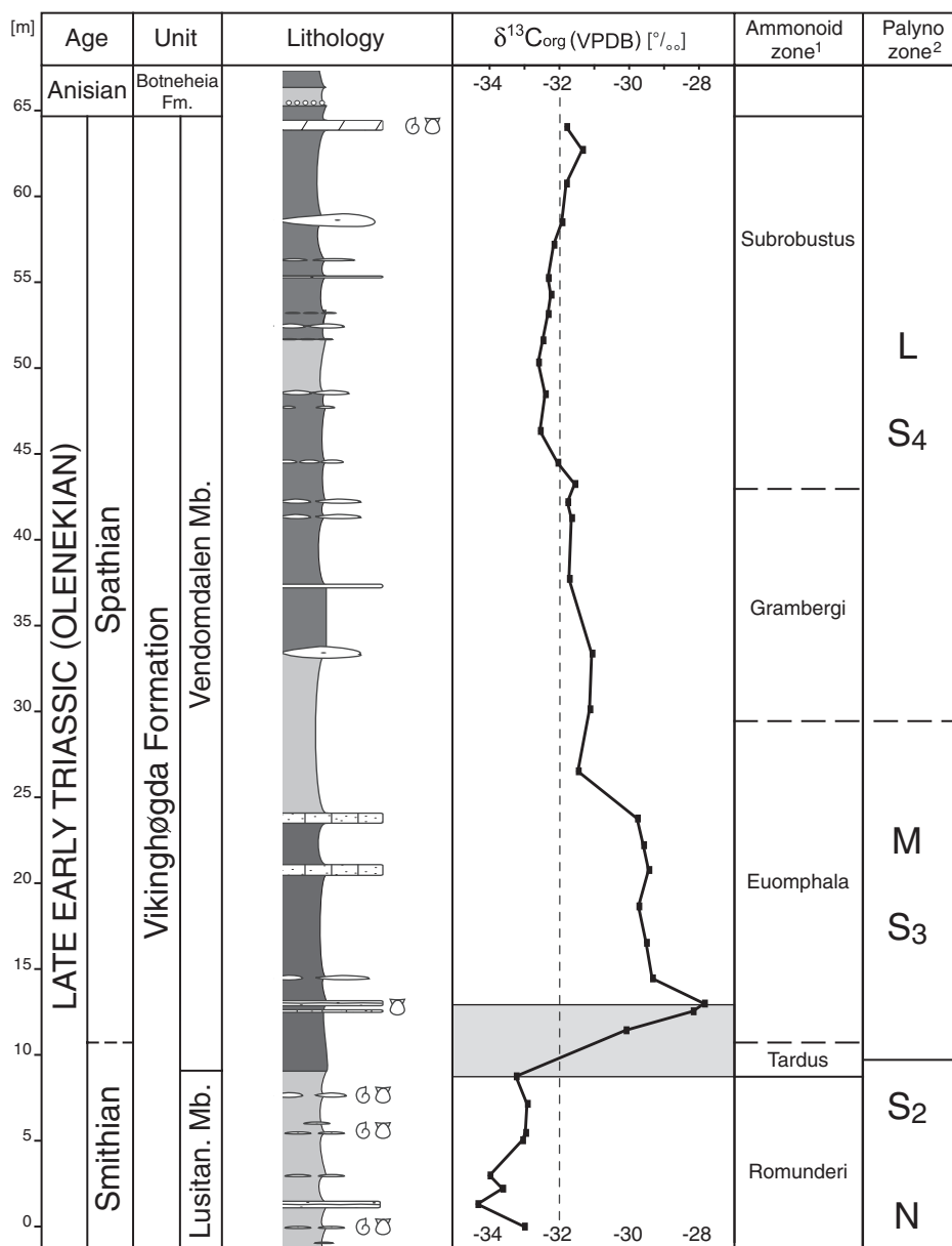
Figure 1. Lithology and bulk organic carbon isotope record of Dicksonfjellet section (Spitsbergen). Ammonoid zones (1) are after Weitschat and Dagys (1989); palynozones (2) are after Hochuli et al. (1989) and Vigran et al. (1998). VPDB—Vienna Pee Dee belemnite.
