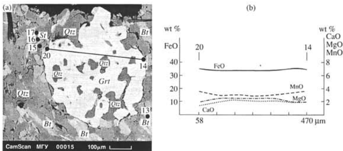
Fig. 4. Late-kinematic garnet from the staurolite-andalusite zone. (a) Back-scattered electron image. (b) Microprobe profile.
