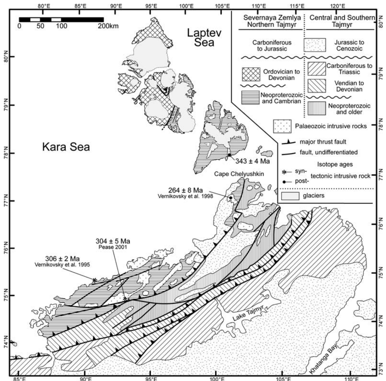
Figure 3. U/Pb and Pb/Pb zircon ages of Carboniferous granitic rocks in the Tajmyr-Severnaya Zemlya area (geological maps simplified from Egiyarov, 1967 and Bezzubtsev et al. 1983).
