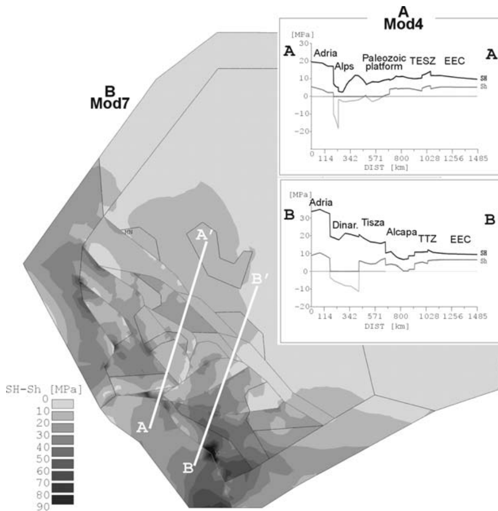
Figure 11. Stress magnitudes: (a) curves of S_H and S_h for Mod4 with constant thickness—stresses are averaged over 100-km-thick lithosphere (location at Fig. 11b); (b) map of differential horizontal stress magnitude for Mod7 with variable stiffness of tectonic units—stresses are averaged relatively to the thickness of a given tectonic unit (see Table 2).
