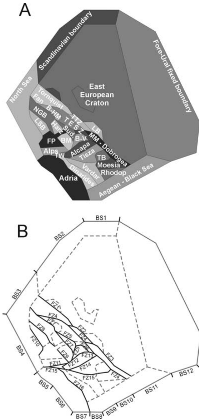
Figure 4. Structural elements of the models: (a) Tectono-mechanical units: BM—Bohemian massif; B-V—Bruno-Vistulicum massif; FP—Franconian platform; LB—Lublin basin; LSB—Lower Saxony basin; MM—Malopolska massif; NGB—North German basin; TB—Transylvanian basin; TTZ—Teisseyre-Tornquist zone; TW—Tauern Window (Table 2). (b) Fault zones and boundary segments; solid lines—faults; dashed lines—continuous boundary between tectonic units; for abbreviations see Tables 3 and 5).
