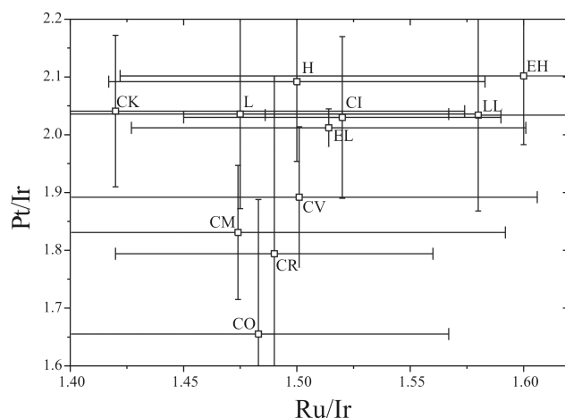
Fig. 9. PGE elemental ratios of chondrites, including only refractory PGE. In contrast to Fig. 8 there is no discrimination between the different chondrite types (database of Tagle 2004).
