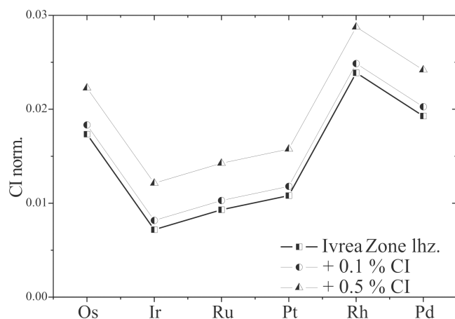
Fig. 5. Model impact melt rock composition resulting from an impact of a CI chondrite on a hypothetical lherzolite target. The PGE-patterns are strongly disturbed by the composition of the target. Therefore, no identification of the projectile is possible. Source of data: CI chondrite (Wasson and Kallemeyn 1988); Ivrea Zone lherzolite (Lorand 1989). Note PGE are plotted in order of decreasing condensation temperatures from solar nebula (after Lodders 2003).
