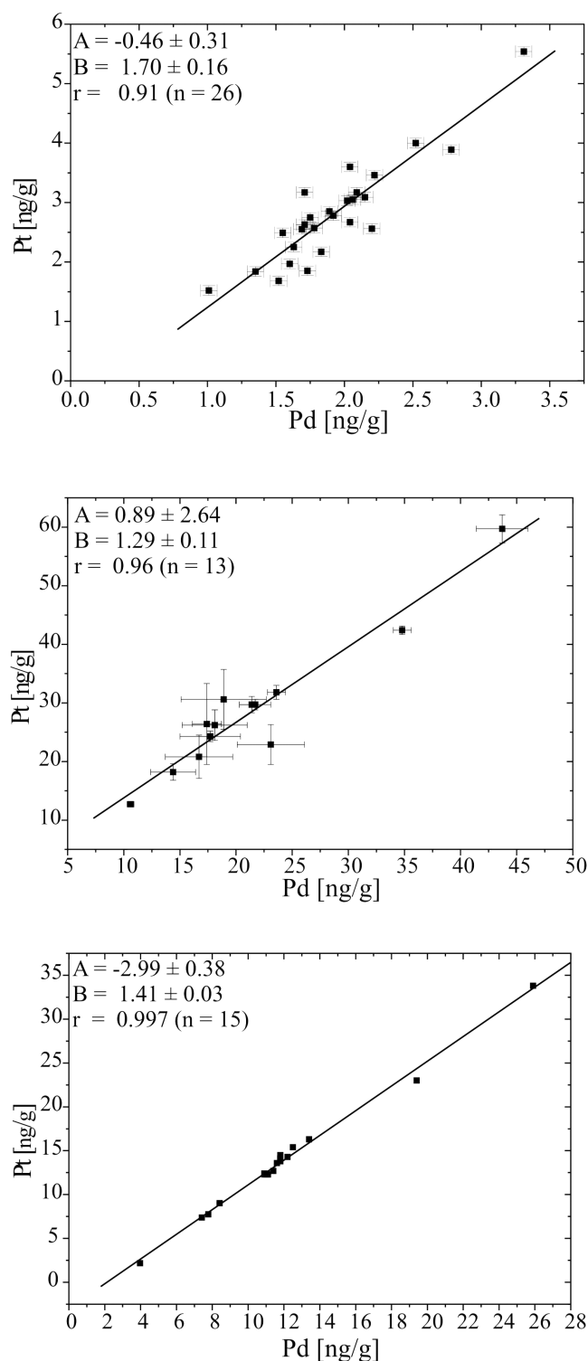
Fig. 7. Regression analysis of Pt versus Pd (linear regressions Y = A + B * X ) in the impact melt rock of (a) Popigai (Tagle and Claeys 2005), (b) Morokweng (McDonald et al. 2001), and (c) Serenitatis basin (Tagle 2005). The slope (B) represents the projectile elemental ratio. The error bars reflect the analytical error given by the respective authors.
