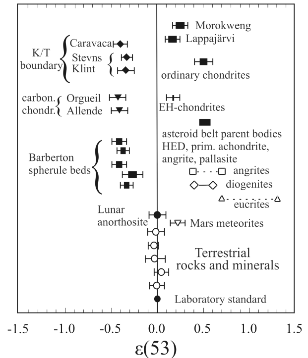
Fig. 4. \epsilon(53) values in terrestrial rocks and impactites, compared to lunar anorthosite, Martian rocks, and different types of meteorites. The figure was redrawn from Shukolyukov and Lugmair (1998), including additional data from Shukolyukov and Lugmair (2000).
