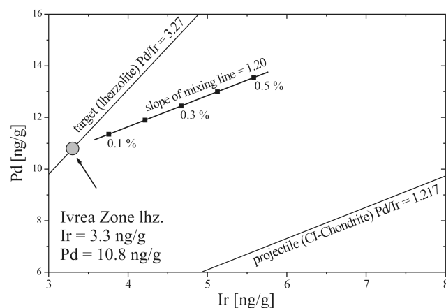
Fig. 6. The mixing trajectory of a model impact melt formed by a lherzolite target and a CI chondrite projectile (same as in Fig. 3). The amount of admixed projectile is given in numbers (0.1–0.5 wt% projectile). The projectile elemental ratio (PER) is determined by linear regression of the slope of the mixing line. Note that the slope of the regression for the impact melt rock is essentially equivalent to the Pd/Ir ratio in a chondritic projectile.
