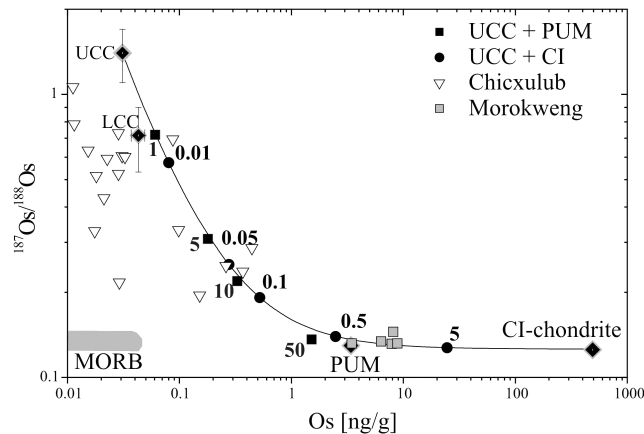
Fig. 3. ^{187}\text{Os}/^{188}\text{Os} ratios versus Os concentrations (ng/g) of some terrestrial rocks, CI chondrites (Wasson and Kallemeyn 1988), and impactites from Morokweng (Koeberl et al. 2002) and Chicxulub (Gelinas et al. 2004). The curve represents the calculated mixing line between CI chondrite values and the upper continental crust (UCC, Os = 0.031 ng/g and ^{187}\text{Os}/^{188}\text{Os} = 1.4, Peucker-Ehrenbrink and Jahn 2001). Percentages of projectile material mixed into hypothetical impact melt are shown as a line with black dots (0.01 to 5 wt%). The mixing trajectory between UCC and primitive upper mantle (PUM, Os = 3 ng/g and ^{187}\text{Os}/^{188}\text{Os} = 0.125, McDonough and Sun 1995; Meisel et al. 2001) is indicated only by solid squares (1 to 50 wt%). Lower continental crust (LCC, Os = 0.043 \pm 0.006 ng/g and ^{187}\text{Os}/^{188}\text{Os} = 0.72 \pm 0.18 was calculated as the range from the values given by (Esperanca et al. 1997; Saal et al. 1998; Peucker-Ehrenbrink and Jahn 2001); MORB = mid-ocean ridge basalt (Schiano et al. 1997).
