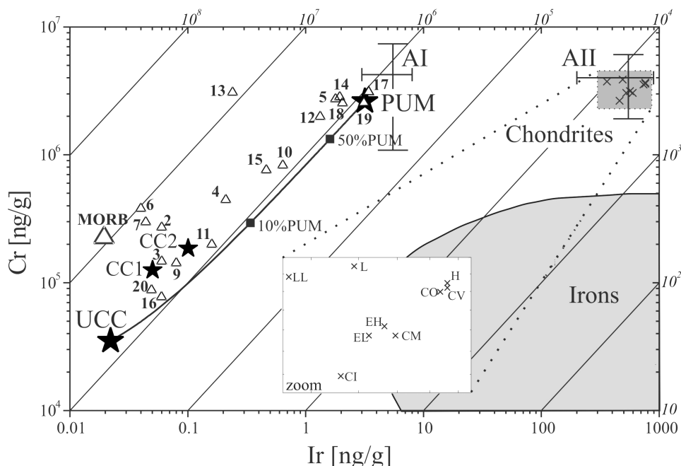
Fig. 1. Cr versus Ir concentrations for terrestrial and extraterrestrial material. AI = PGE-poor achondrites (HED, angrites, and aubrites), AII = PGE-rich achondrites (brachinites, ureilites, lodranites, acapulcoites, and winonaites). Source of data: chondrites (Wasson and Kallemeyn 1988); iron meteorites, achondrites I (AI), and achondrites II (AII) error represent the range of published concentrations (Koblitiz 2000); numbers 1 to 20 represent terrestrial rocks, concentrations and references are given in Table 2. PUM = primitive upper mantle; MORB = mid-ocean ridge basalt; UCC = continental crust; CC = continental crust; values above and right of the diagram represent the Cr/Ir ratio of the respective line; note that for higher resolution of the chondrite a field has been “zoomed” within the middle of the diagram.
