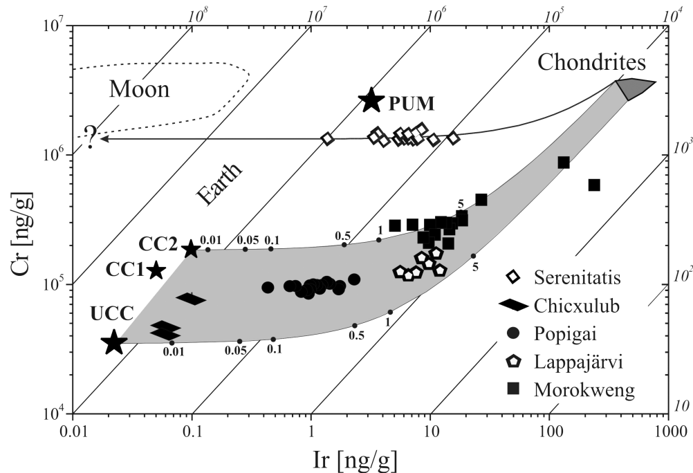
Fig. 2. Cr versus Ir concentrations of terrestrial and lunar target rocks compared to the composition of impact melts of five case studies. The grey field indicates the most likely mixing trajectories between chondritic projectiles and common terrestrial targets. Source of data: terrestrial rocks and chondrites (Fig. 1), Moon = lunar crust, values extracted from Fig. 5b in Richter et al. (2000). Numbers represent wt% chondritic material in the mixing trajectories. Some references of data are also given in the text.
