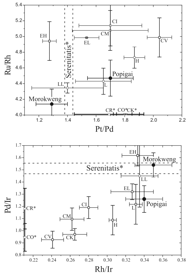
Fig. 8. Comparison of the PGE “projectile elemental ratios” of the impact melt rocks of Popigai, Morokweng, and Serenitatis to the elemental ratios of chondrites calculated from the database of Tagle (2004) for different types of chondrites. The uncertainty bars for the meteorites represent 1\sigma standard deviations. * = only one ratio known.
