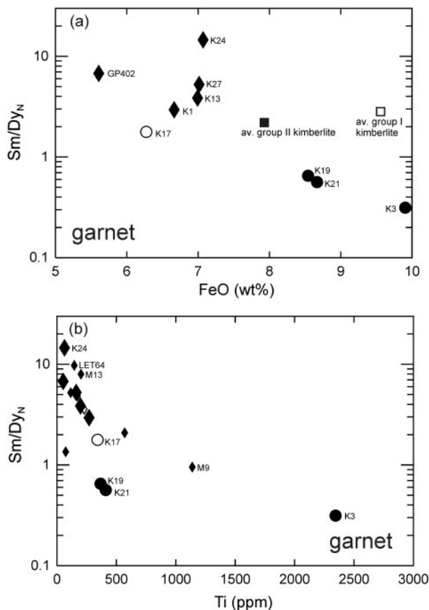
Fig. 14. \text{Sm}/\text{Dy}_N vs \text{FeO} (wt%) (a) and \text{Ti} (ppm) (b) contents in garnets. Also shown are the compositions of average Type I and II kimberlites (squares, Nowell et al. , 2004). Symbols are as in Fig. 6.
