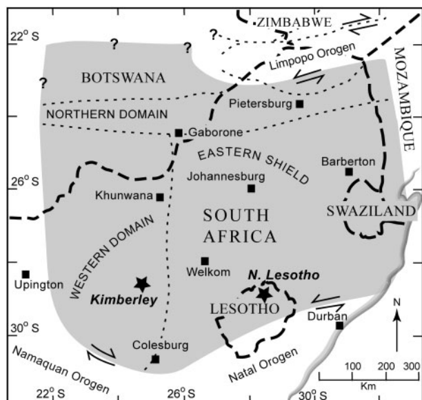
Fig. 1. Simplified geological map modified from Schmitz (2002). The dashed line between Colesburg and Gaborone denotes the Colburg magnetic lineament, interpreted to mark the suture between the Eastern and Western Kaapvaal blocks. Note the location of Kimberley west of the suture and the position of northern Lesotho close to the southern edge of the craton.
