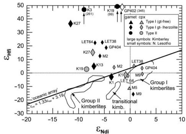
Fig. 10. \epsilon_{Hf} vs \epsilon_{Nd} isotope diagram showing the data for garnets and cpx from xenoliths from Lesotho and Kimberley. The fields for Group I, Group II and transitional kimberlites are also shown (data from Nowell et al. , 2004). Oceanic mantle array (regression line through ocean island and mid-ocean ridge basalt data) from Vervoort & Blichert-Toft (1999). K27, K19 and K3 garnets plot outside the diagram in \epsilon_{Hf} (values in parentheses, Table 4).
