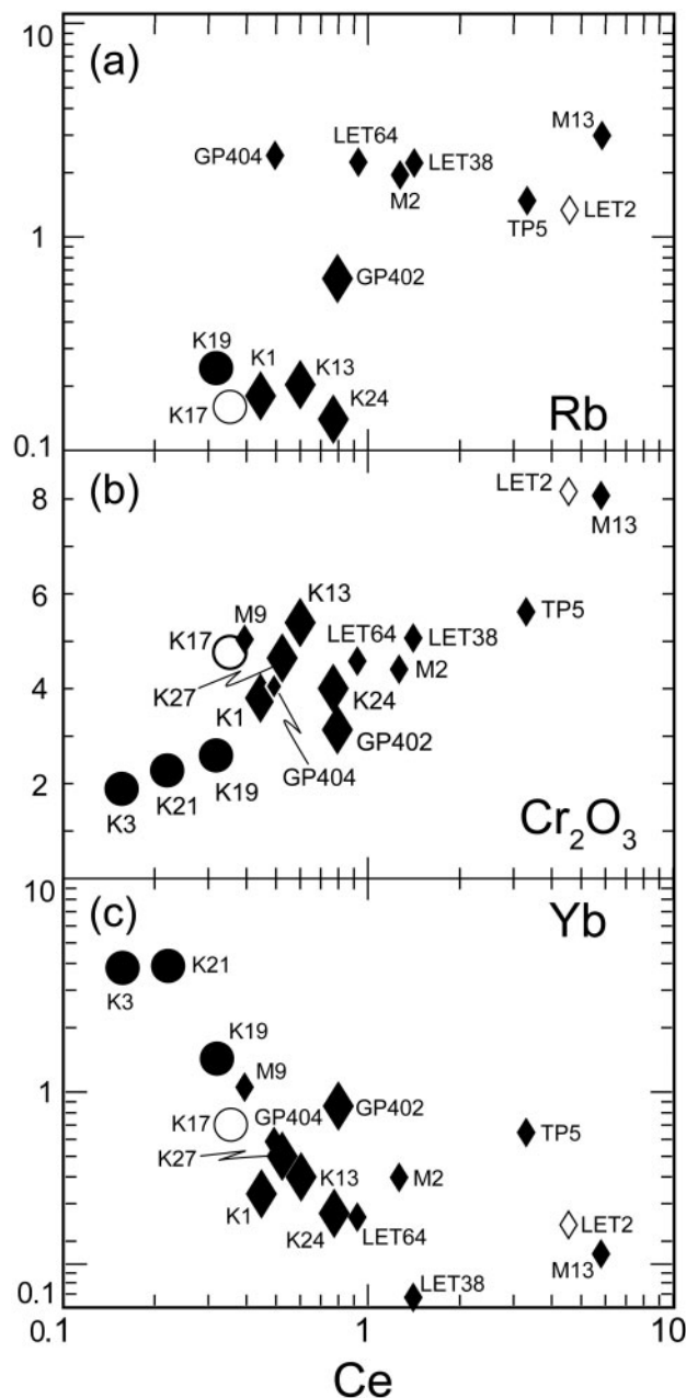
Fig. 15. Correlation of LREE (Ce) content in garnet with (a) Rb, (b) \text{Cr}_2\text{O}_3 (wt%) and (c) Yb. All but \text{Cr}_2\text{O}_3 in ppm. Symbols are as in Fig. 6.
