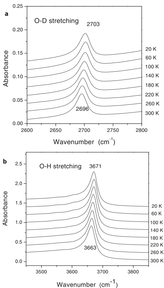
FIGURE 1. (a) IR powder absorption spectra of \text{Ca}_3\text{Al}_2(\text{O}_4\text{D}_4)_3 between 20 and 300 K (the spectra are shifted for clarity); (b) IR powder absorption spectra of O-H stretching bands between 20 and 300 K (the spectra are shifted for clarity); and (c) temperature dependence of the integrated band intensity (i.e., the band area between 2650 and 2750 \text{cm}^{-1} after linear baseline corrections) of the O-D stretching band near 2696 \text{cm}^{-1} . The lines are visual guides. The OH and OD bands of hydrous/deuterated garnets show weak changes in absorption between 20 and 300 K.
