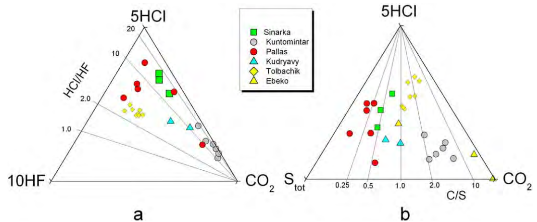
Figure 8. Relative concentrations of “acidic” components in fumarolic gases. (a) Ternary plot for relative concentrations of HCl, HF, and CO 2 and (b) the same for relative concentrations of HCl, CO 2 , and S tot . See text for more details.
