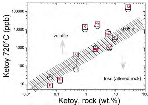
Figure 12. Correlation between rock and condensate compositions for rock-forming elements. See text for discussion.
