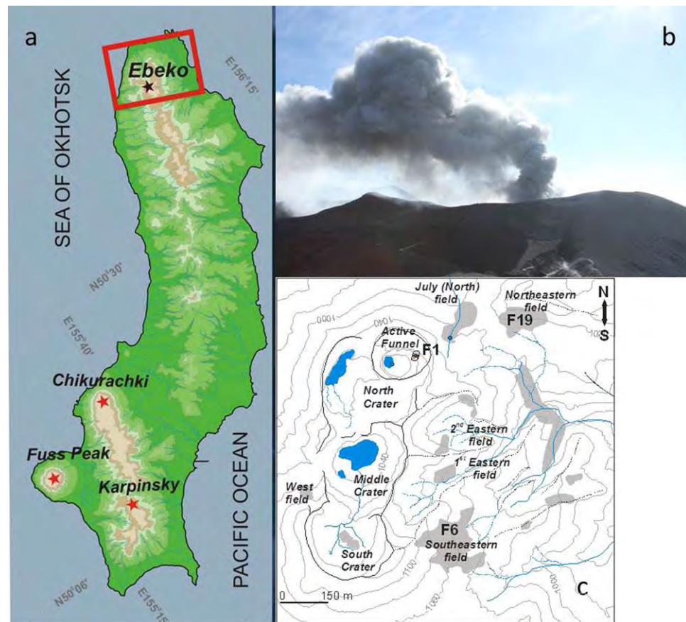
Figure 2. (a) Ebeko volcano on Paramushir Island. (b) Typical ash-steam plume in the summer 2017, photo Iliia Chaplygin. (c) Map of the summit part of Ebeko volcano with fumarolic fields (gray spots) and sampling points as in Table 1.
