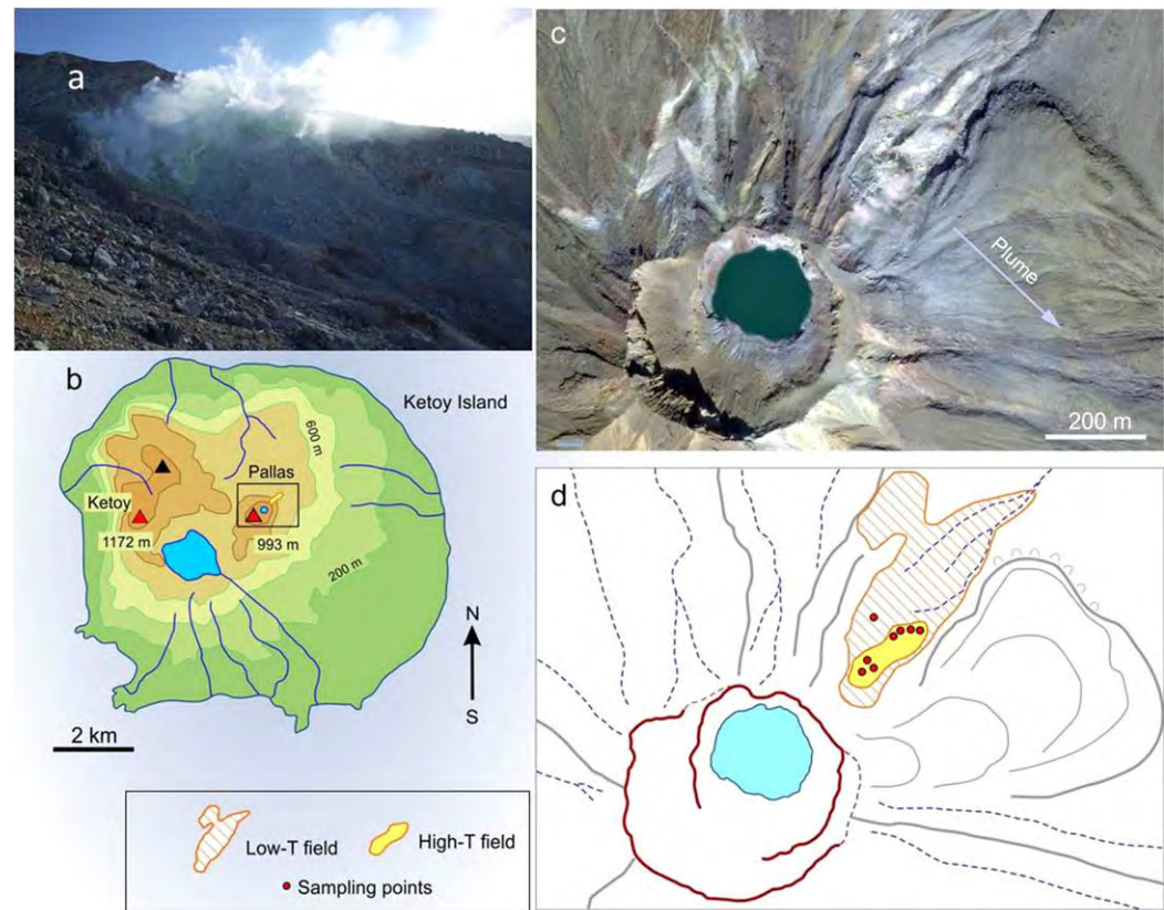
Figure 5. (a) Fumarolic field of Pallas volcano on Ketoy Island. Photo Ilia Chaplygin. (b) Map of Ketoy Island with location of Pallas volcano. (c) Google map image of the Pallas cone with Glazok Lake and fumarolic field. (d) Location of the fumarolic gas sample sites.
