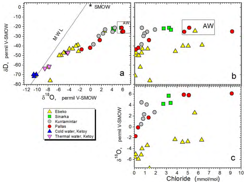
Figure 16. Isotopic composition of the volcanic gas condensate and chlorine content. (a) \delta\text{D} versus \delta^{18}\text{O} plot for all sampled condensates and meteoric waters (Table 3) and (b, c) \delta\text{D} and \delta^{18}\text{O} versus chlorine content. MWL, Meteoric Water Line; AW, "Andesitic" (Arc) Water (Taran et al., 1989).
