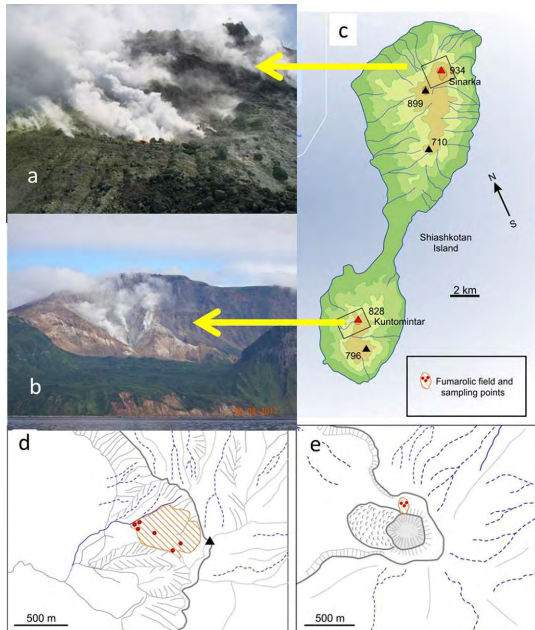
Figure 4. (a, b) Fumarolic fields of (a) Sinarka and (b) Kuntomintar volcanoes on Shiashkotan Island. Photo Mikhail Zelen-ski and Elena Kalacheva. (c) Map of Shiashkotan Island with locations of Sinarka and Kuntomintar volcanoes. (d, e) Sketch maps of the craters ((d) Kuntomintar and (e) Sinarka) with locations of the fumarolic gas sampling points.
