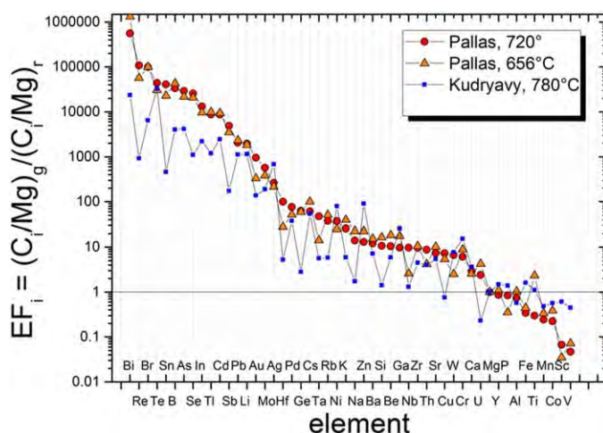
Figure 11. Enrichment factors (EF) normalized to Mg for two high-temperature volcanic gas condensates from Pallas volcano and a 780°C condensate from Kudryavy volcano. EF sorted by descending for the 720°C condensate of Pallas.
