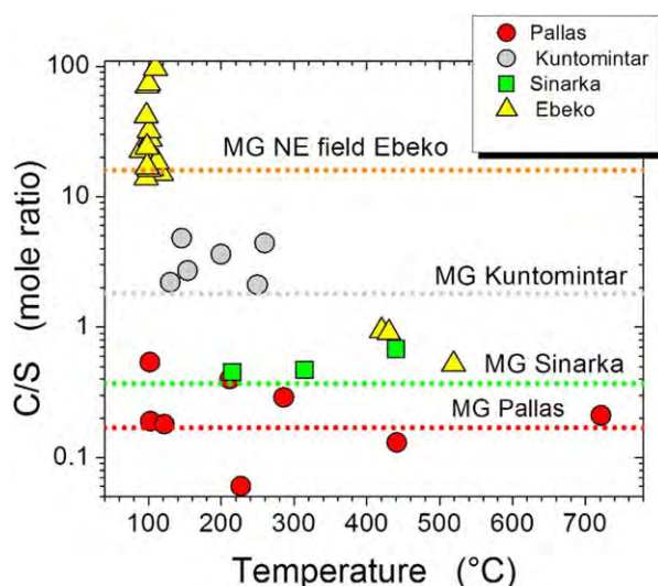
Figure 9. C/S ratios versus temperature of fumaroles. Dotted lines show the average C/S values measured by the MultiGas analyzer. More points for Ebeko are plotted using data from Kalacheva et al. (2016) and Menyailov et al. (1985).
