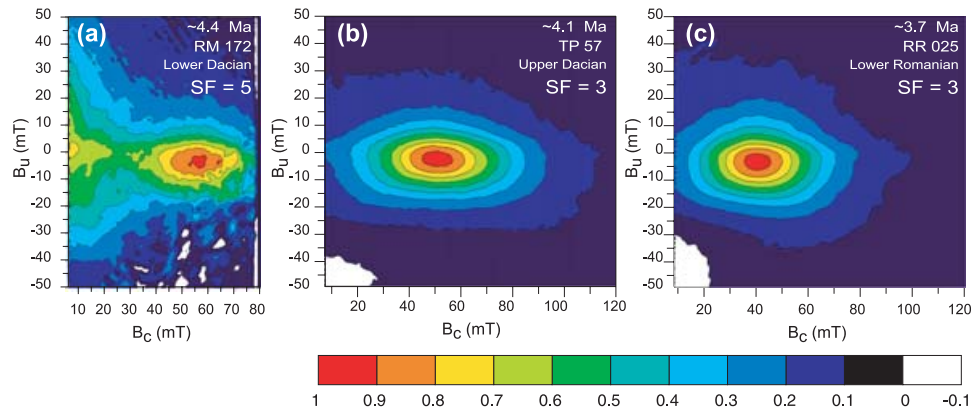
Figure 3. Representative FORC diagrams for three samples from the Carpathian foredeep. Each FORC distribution contains 10 contours. The scale indicates the density of the FORC distribution. In the upper right-hand corner are listed the sample code, age and stage of the sedimentary rocks and the applied smoothing factor (see Pike et al. 1999; Roberts et al. 2000).
