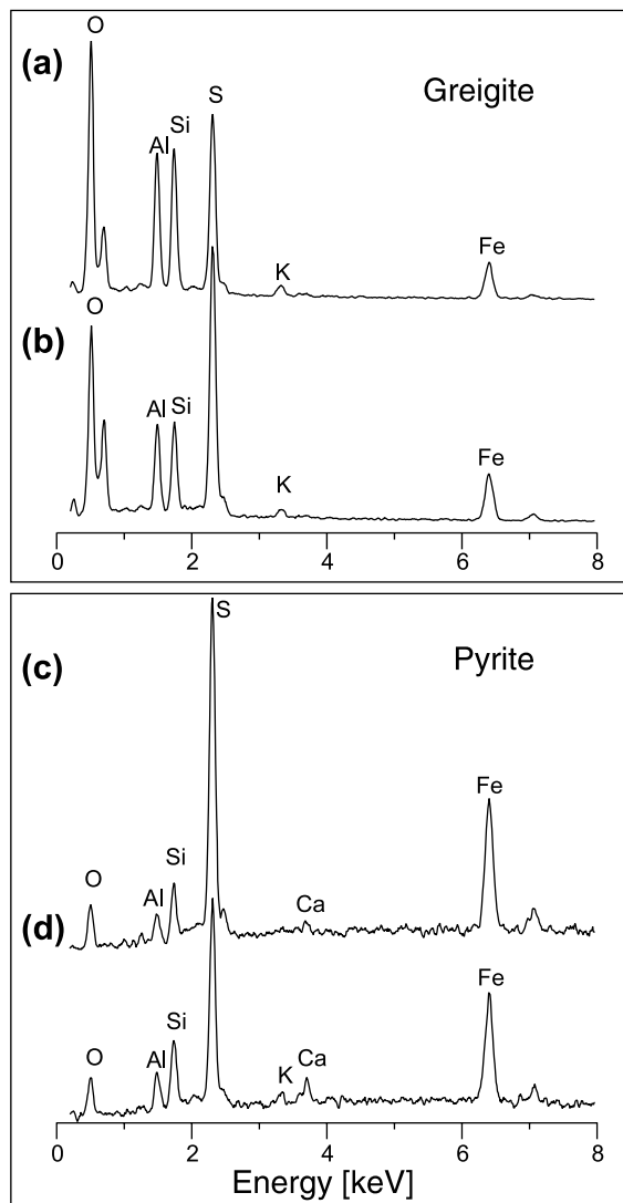
Figure 7. Backscattered electron micrograph of a dispersed magnetic extract from sample BD115. Clusters of fine-grained greigite (a and b) with individual grain sizes <50\text{ nm} . Grains c and d are pyrite particles with an average grain size of 2 \mu\text{m} . The respective elemental spectra are shown below; a cross on the micrograph marks the exact position of the EDS analysis. See also the caption for Fig. 6.
