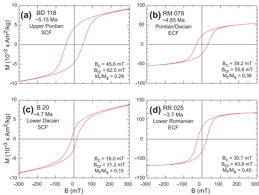
Figure 2. Hysteresis loops for characteristic samples from the Carpathian foredeep. The central parts of the loops are shown up to \pm 300 mT. The loops are displayed after paramagnetic slope correction on a mass-specific basis. The age and stage of the sedimentary rocks is indicated on the upper left-hand side of each panel. Hysteresis parameters are listed on the lower right-hand corner of each panel.
