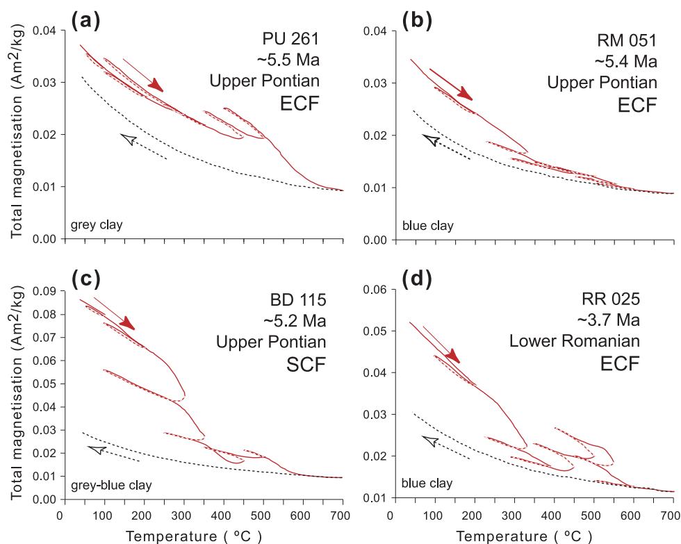
Figure 5. Representative thermomagnetic runs for samples during different heating (solid lines) and cooling (dashed lines) runs that were performed at a rate of 10\text{ }^{\circ}\text{C min}^{-1} . The total magnetization is plotted in a series of runs to increasingly higher temperatures. Arrows refer to heating and cooling segments, respectively. Measurements were made every six seconds, which is equivalent to one every degree Celsius. The applied cycling field varied between 150 and 300 mT. In the upper right-hand corner are the approximate age and the stage corresponding to each sample. An increase in the total magnetization starting at 300\text{ }^{\circ}\text{C} is evident in panel (a), indicating newly formed magnetic minerals, although the original magnetic material does not seem to have been affected. In (b), (c) and (d) an increase in the total magnetization starts at 410\text{--}416\text{ }^{\circ}\text{C} indicating the formation of new magnetic minerals because of oxidation of an iron sulphide (either magnetic or not magnetic).
