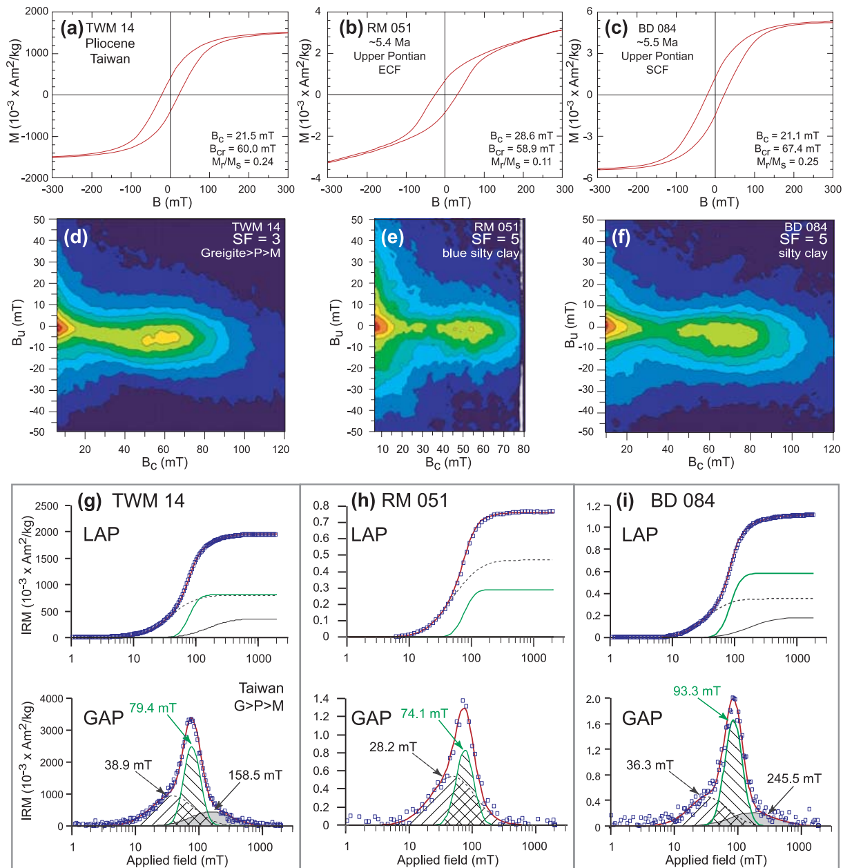
Figure 9. Hysteresis loops, FORC diagrams and IRM component analysis for a magnetic concentrate TWM 14 (panels a, d and g) from Pliocene–Pleistocene sedimentary rocks in Taiwan and for Carpathian foredeep bulk samples RM 051 (panels b, e and h) and BD 084 (panels c, f and i), respectively. See also captions for Figs 3 and 4.
