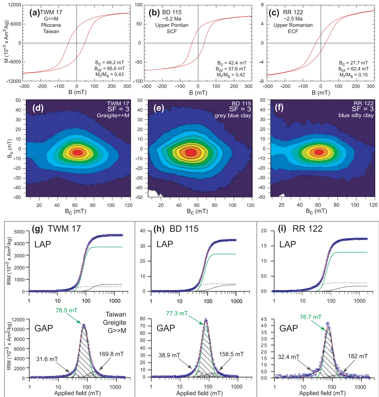
Figure 10. Hysteresis loops, FORC diagrams and IRM component analysis for a magnetic concentrate TWM 17 (panels a, d and g) from Pliocene–Pleistocene sedimentary rocks in Taiwan and for Carpathian foredeep bulk samples BD 115 (panels b, e and h) and RR 122 (panels c, f and i), respectively. See also the caption for Figs 3, 4 and 9.
