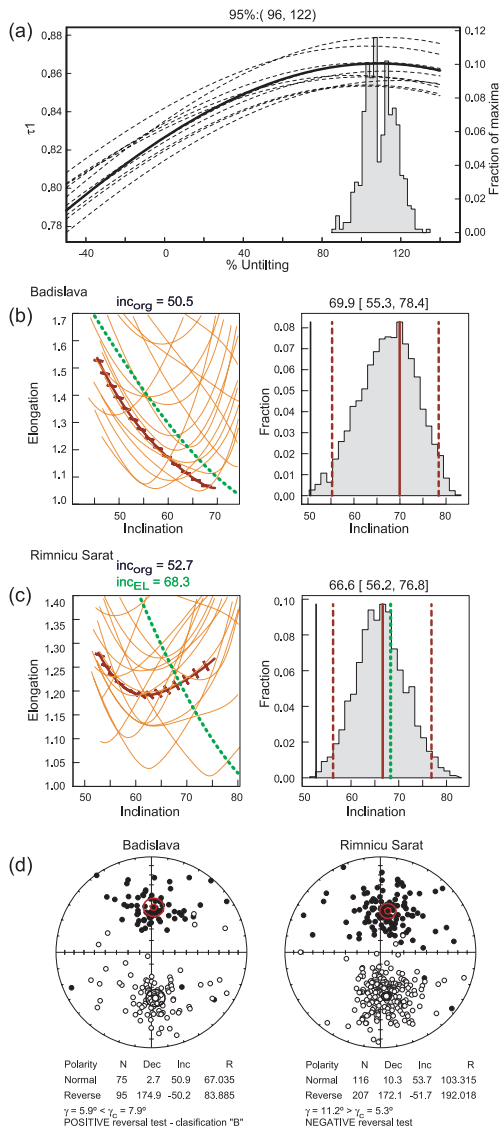
Figure 8. (a) Bootstrap fold test of Tauxe & Watson (1994), applied to both normal and reversed polarity characteristic remanent magnetization (ChRM) directions. Variation of the principal eigenvector \tau_1 with percentage of unfolding is depicted as a solid line; dashed lines are bootstrap examples. The distribution of the maxima of \tau_1 is shown by the histogram. The 95 per cent confidence interval (96–122 per cent) includes the 100 per cent unfolding orientation, which supports a pre-folding magnetization. Panels b and c contain elongation–inclination plots upon flattening for Badislava and Rimnicu Sărat, respectively, following the field model TK03.GAD of Tauxe & Kent (2004). On the left-hand side: thick red line = inclination from the data set, red barbed lines = elongation direction, green dotted line = model, thin lines = examples of bootstraps. The inclination most consistent with the TK03.GAD model is the intersection with the model (green dotted line). On the right-hand side the distribution resulting from 5000 bootstraps is given, including the most frequent inclination (thick red line) and the model (the green dotted line). The 95 per cent confidence limit is shown in grey shading. The inclination of the original data set (black line) is significantly lower than the 95 per cent confidence interval. (d) Equal area projection of ChRM directions in tilt-corrected coordinates for the samples marked with green dots from the Badislava and Rimnicu Sărat records in Fig. 1. Solid (open) circles indicate normal (reversed) polarity. The reversal test is positive for Badislava (classification B according to McFadden & McElhinny (1990), with the angle \gamma between the normal and reversed polarities smaller than the critical angle \gamma_c ). The reversal test is negative for the Rimnicu Sărat section.
