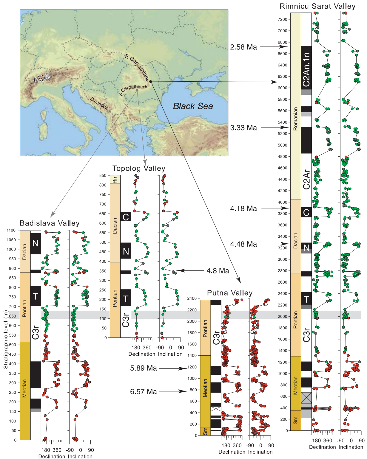
Figure 1. Map of the study areas in the Eastern Carpathian foredeep (ECF) and the Southern Carpathian foredeep (SCF). Polarity zones with palaeomagnetic data for the studied sections for the four sampled valleys: Putna and Rimnicu Sărat from ECF and Bădăslava and Topolog from SCF. Black (white) denotes normal (reversed) polarity. Ages of the most important subchrons are displayed (C = Cochiti, N = Nunivak, T = Thvera). Data are only shown for palaeomagnetic ChRM directions. Red symbols denote samples where the magnetic carrier is exclusively an iron oxide; white symbols denote samples where the magnetic signal is carried by an iron oxide, but where oxidation of an iron sulphide, most probably pyrite, also occurs; green dots indicate samples with an iron sulphide as the magnetic carrier. Next to the polarity column are represented the limits between different (local) stages of the Miocene (Sarmatian, Meotian, Pontian) and of the Pliocene (Pontian, Dacian and Romanian) according to geological maps in use (see also Vasiliev et al. 2004, 2005). The grey rectangle (below the Thvera subchron) indicates the approximate level of the Miocene/Pliocene boundary.
