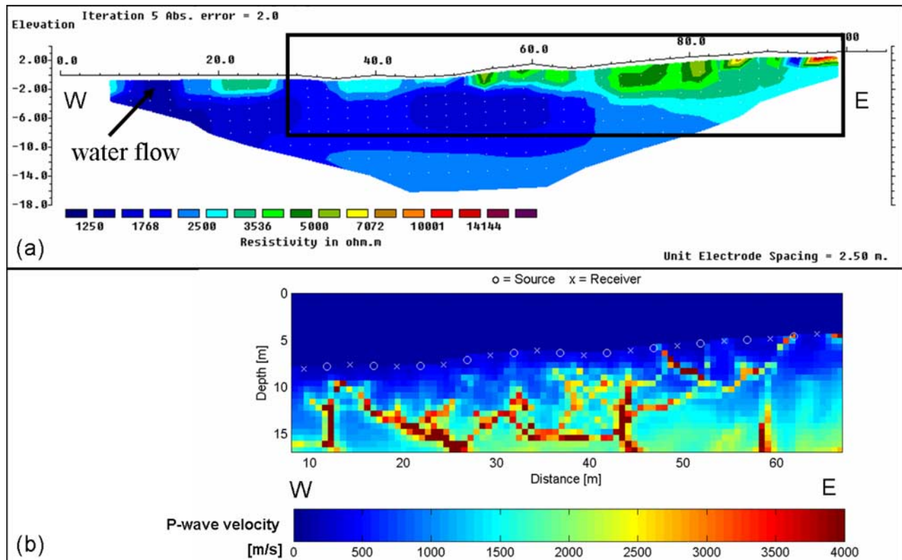
Figure 8. (a) ERT survey results and (b) seismic refraction results at Incinerador site (site D). Black rectangle marks location of seismic profile. For location of profile, see Figure 3.
