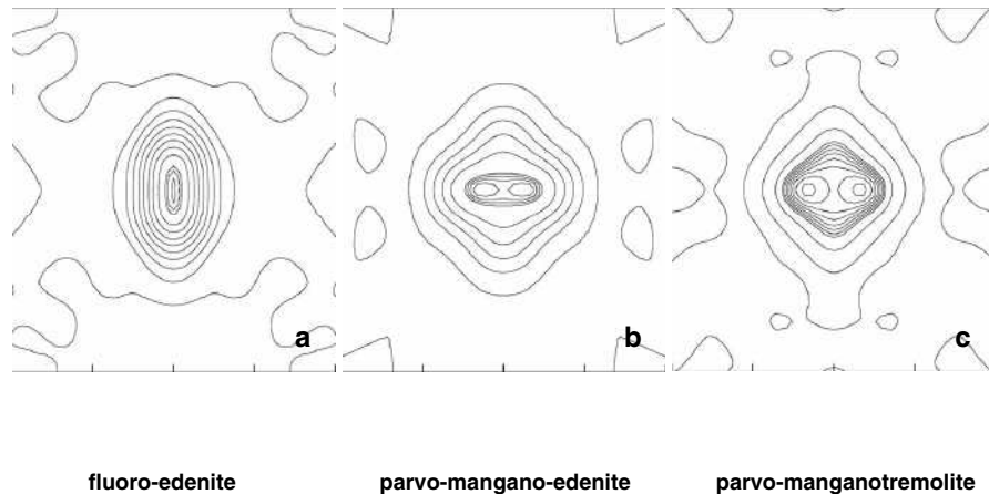
FIGURE 2. Difference-Fourier sections at the A-group sites. Sections are approximately parallel to (\bar{2}01) . The contour intervals are: (a) 1 e/\text{\AA}^3 below 10 e/\text{\AA}^3 and 0.2 e/\text{\AA}^3 above 10 e/\text{\AA}^3 , (b) 1 e/\text{\AA}^3 below 6 e/\text{\AA}^3 and 0.1 e/\text{\AA}^3 above 6 e/\text{\AA}^3 , (c) 1 e/\text{\AA}^3 below 3.5 e/\text{\AA}^3 and 0.1 e/\text{\AA}^3 above 3.5 e/\text{\AA}^3 .
