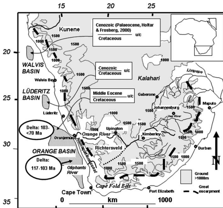
Fig. 1. Outline map of southern Africa showing the depositional basins on the continental shelf, the region of >1000 m elevation and the Great Escarpment. In addition, the ages of the sediments immediately above the top-Cretaceous unconformity within each basin are given, according to the few dates available.
