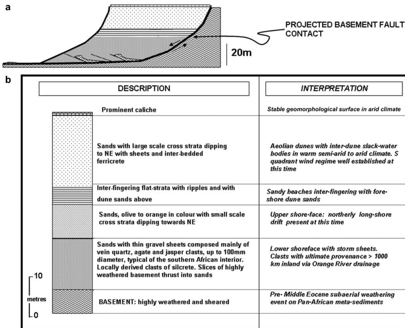
Fig. 3. (a) Diagrammatic cross-section of the exposure of the downfaulted, Middle Eocene sediments at Buntfeldschuh. (b) Measured section with description and interpretation of the Buntfeldschuh section. Intertidal sands interfinger with dune sands, showing that coastal dune fields were coeval with beaches.
