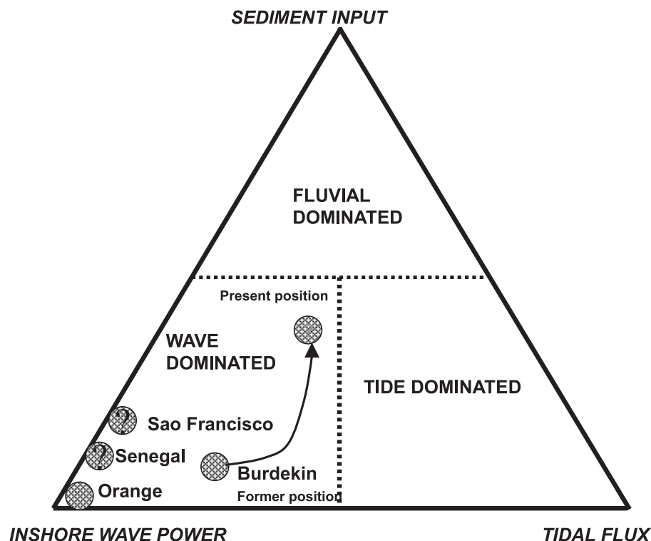
Fig. 7. Summary diagram of the Orange River in the scheme of deltas.
