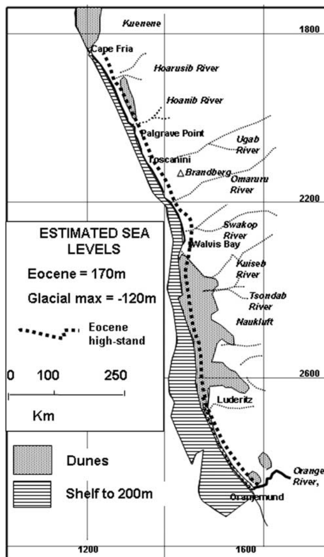
Fig. 5. Map showing variations in shelf extent between the Pleistocene glacial-maximum lowstand of sea level and the Eocene sea-level highstand.
