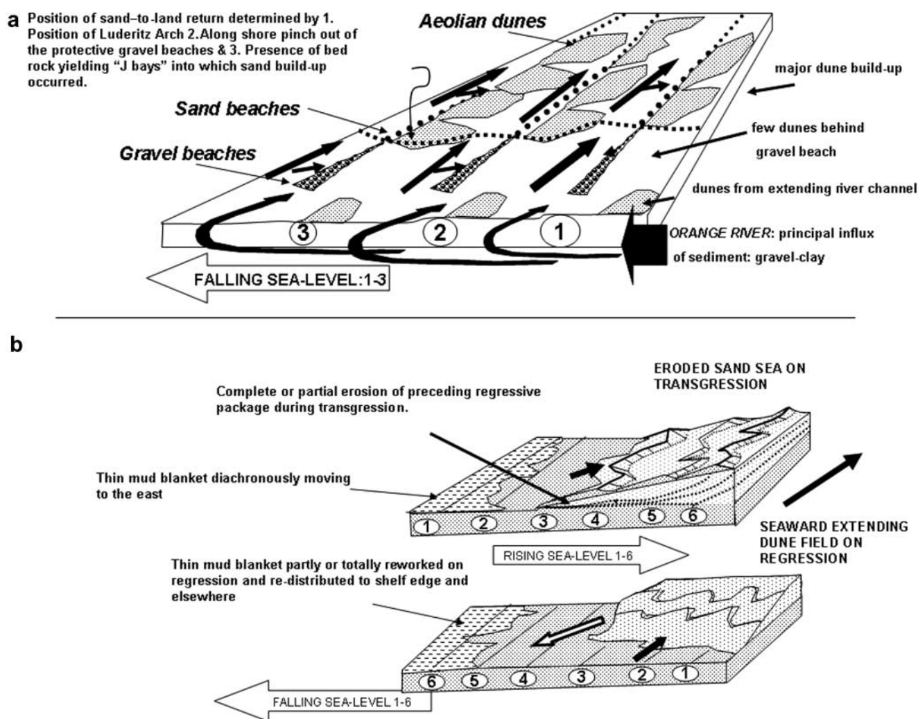
Fig. 6. Diagrammatic illustrations of the processes taking place in shelf areas subject to Tertiary reworking during sea-level changes. (a) Regression (during successive time steps 1–3) has yielded a sequence of gravel beaches and longshore-transported sand that has been displaced onto dune systems. (b) The behaviour of the dune field varies during regressions (lower scenario) and transgressions (upper scenario). (Numbers 1–6 refer to successive positions of the regressing or transgressing shoreline.)
