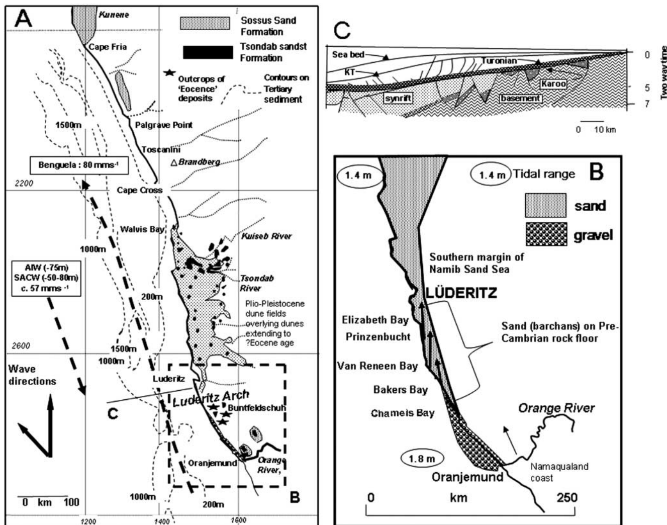
Fig. 2. Dispersal of sediments at the mouth of the Orange River and northwards along the coast. (a) Distribution on land of post-Cretaceous sediments and dated and probable Eocene deposits. Offshore contours show the thickness of Tertiary sediment (Aizawa et al. 2000). Current and wave-orientation data are shown, together with post-Pliocene sediment dispersal paths along the Namibian coast (see text for sources; AIW, Arctic Intermediate Water; SACS, South Atlantic Central Water). Locations of (b) and (c) are shown. (b) Distribution of sediment along the Namibian coast and positions of sand take-offs to the Namib Sand Sea. (c) Interpreted geo-seismic section based on Aizawa et al. (2000). KT, Cretaceous–Cenozoic unconformity of the inner shelf. Two-way time is in seconds.
