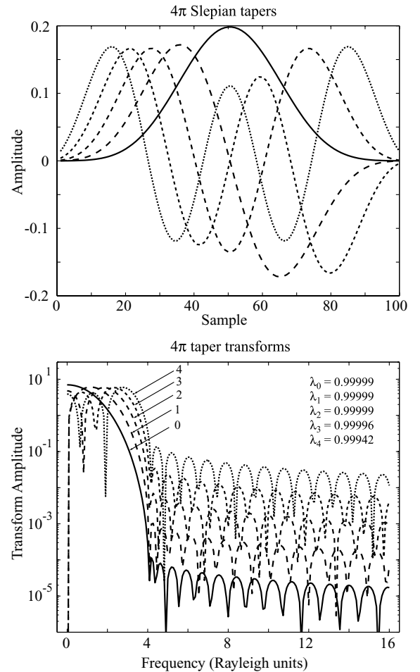
Figure 2. The five lowest order 4\pi Slepian tapers (top panel) and corresponding Fourier transform amplitudes (lower panel). Solid lines correspond to the zero-order sequence v_0(t) , higher-order tapers are plotted with dashed lines. We have used N = 100 and NW = 4 . Estimated eigenvalues are also provided.
