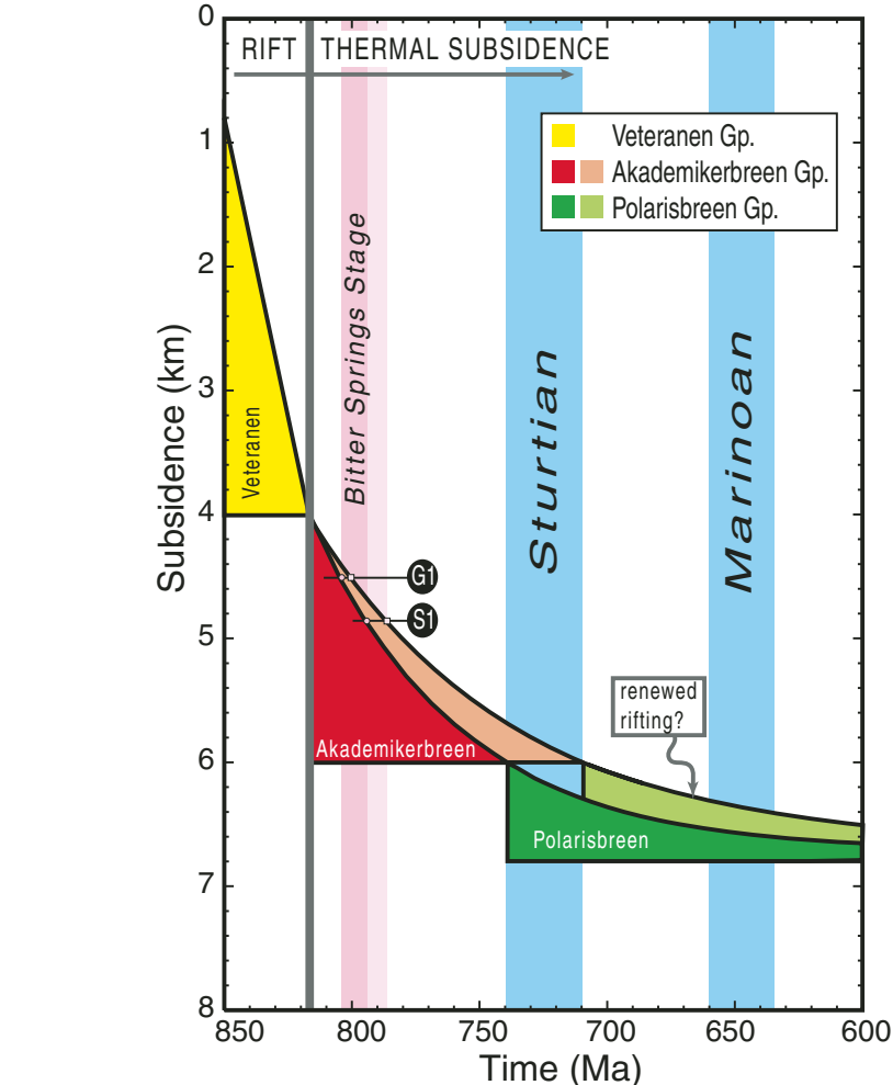
Figure 10. Age model for the Hecla Hoek strata of East Svalbard. The black curves show rifting (Veteranen Group) and thermal subsidence (Akademikerbreen Group) of an originally 35-km-thick continental crust and 100-km-thick lithosphere. The dark/light colored triangular areas beneath the solid curves depict the age distribution of the continuum of stratigraphic levels assuming onset of Sturtian glaciation at ca. 740 and ca. 710 Ma, respectively. The Akademikerbreen Group was deposited in ~90 m.y., and the entire Bitter Springs Stage lasted ~12 m.y. Discussion of the Polarisbreen Group is beyond the scope of this paper; however, it is worth noting that the post-Sturtian subsidence curve is more complicated than shown and should incorporate both (1) compaction of Polarisbreen shales, and (2) the possibility of renewed rifting (Herrington and Fairchild, 1989).
