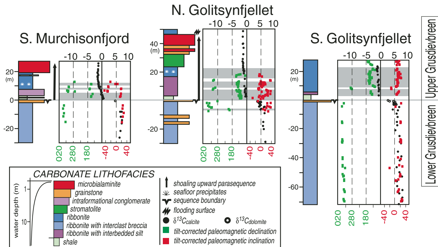
Figure 7. Paleomagnetic and carbon-isotope stratigraphy across the G1 sequence boundary. Carbon isotope data for calcite/dolomite are plotted with solid/open black circles, while tilt-corrected paleomagnetic declination and inclination are plotted with solid green and red squares, respectively. White and gray areas correspond to opposite magnetic polarities. Stratigraphic height is set to 0 meters at the GI sequence boundary. Carbonate lithofacies are color coded, and wider boxes reflect depositional environments in shallower water. Seafloor precipitates are thought to be calcite pseudomorphs after aragonite.
