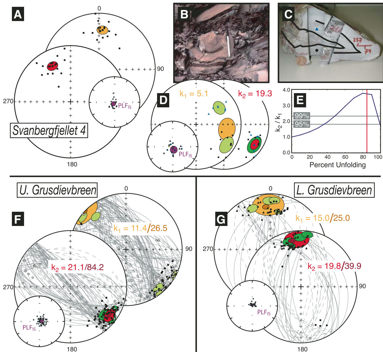
Figure 6. Tests for the presence of prefolding or synfolding magnetization. Equal-area nets show in situ (orange) and tilt-corrected (red) Fisher distributions of the characteristic remanent magnetization (ChRM) direction and in situ distribution of the present-local field (PLF) overprint (purple) for the Lower Grusdievbreen (IGfm) (G), Upper Grusdievbreen (uGfm) (F), and Svanbergfjellet (S4mb) (A). Filled/open circles are lower/upper-hemisphere least-squares line fits to demagnetization curves. Gray arcs are great circle fits to demagnetization curves with overlapping magnetic components. Where multiple stratigraphic sections are present, as in (F) and (G), individual section-mean Fisher statistics are plotted as light green (in situ) and dark green (tilt-corrected) ellipses, while the averages of section-mean directions are plotted as dark orange (in situ) and dark red (tilt-corrected) ellipses. Values k_1 and k_2 are in situ and tilt-corrected Fisher (Fisher, 1953) concentration parameters measuring the dispersion in individual paleomagnetic data (light orange and light red) and site-mean paleomagnetic data (dark orange and dark red). S4mb contains numerous disturbed beds of pink limestone and red marl with detached synsedimentary folds (B) and erosional truncations (left of the pen cap in B). Paleomagnetic directions from the upper limb (blue triangles) and lower limb (black circles) of the fold pictured in C are plotted on the equal-area net in D. The PLF overprint direction fails the fold test, while the primary magnetic component passes the synsedimentary fold test at the 99% confidence level (E). (E) Shows that k_2/k_1 is maximized at 86% unfolding and that the S4mb ChRM was likely acquired prior to, or at the onset of slump folding, and thus dates from the time of sedimentation. (Note: the demagnetization behavior of the ChRM from A and D is identical, and the two directions are considered to reflect the same paleomagnetic component. The difference in absolute direction of the ChRM in D with respect to the ChRM in A is just another reflection of the observation that the ChRM was acquired prior to disruption and folding.) Both the uGfm (F) and IGfm (G) directions were derived from multiple stratigraphic sections separated by >100 km. Although paleomagnetic directions are subparallel to the NNW-trending Caledonian fold axes, k_2/k_1 is maximized at 100% unfolding, and both uGfm and IGfm pass the McElhinny (1964) fold test at greater than the 92% confidence level.
