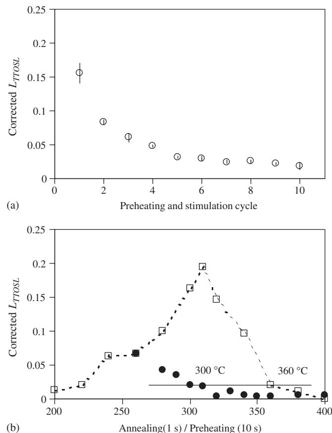
Fig. 2. Sensitivity-corrected thermally transferred OSL signal ( L_{TTOSL} / T_{TTOSL} ) plotted (a) for repeated cycles of preheat ( 260^\circ\text{C} for 10 s) and blue stimulation ( 125^\circ\text{C} for 90 s) as a function of cycle and as a function of (b) annealing (1 s, □) or preheating (10 s, ●) temperature prior to the measurement.
