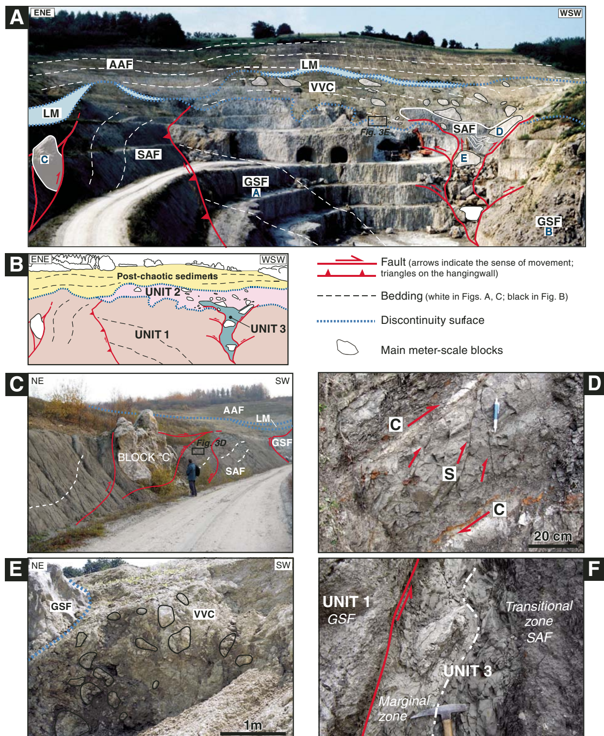
Figure 3. (A) Panoramic view of the Moncucco quarry. SAF—Sant’Agata Fossili marls (upper Tortonian-lower Messinian); GSF—Gessoso Solifera Formation (Messinian); VVC—Valle Versa chaotic complex (upper Messinian); LM—Lago-Mare deposits (upper Messinian); AAF—Argille Azzurre Formation (lower Pliocene). Capital letters (A–E) indicate the blocks described in the text. (B) Drawing of Figure 3A, showing the distribution of the three chaotic units discussed in the text. (C) Unit 1: lozenge-shaped gypsum block tectonically included within the SAF (block C, Fig. 3A). Symbols as in A. (D) Unit 1: S-C structures in the SAF marls. The C planes coincide with the bedding surfaces. Red arrows indicate the sense of shear. Location in C. (E) Unit 2: VVC: angular to rounded gypsum and carbonate blocks floating in a fine-grained matrix. See A for location. (F) Tectonic contact separating Unit 1 and Unit 3. The boundary between the marginal and the transitional zones is also shown (white dotted line). See Figure 7A for location.
