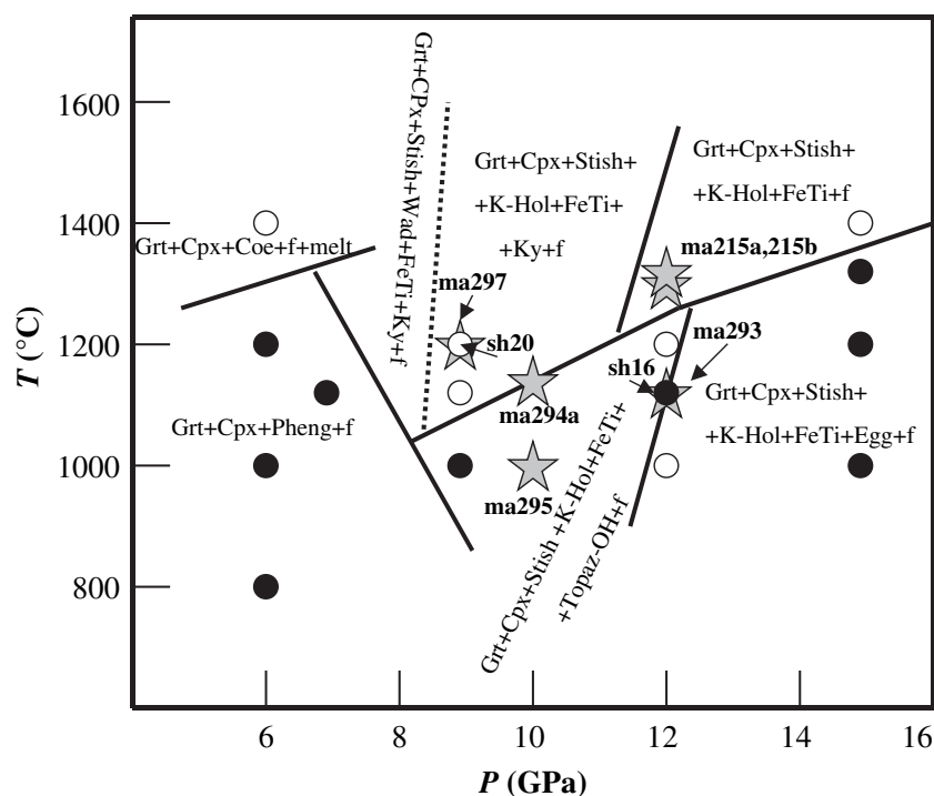
Fig. 5. Experimental data for the typical sediment (pelite) composition adopted from Ono (1998) and our data for comparison plotted onto P - T diagram. P - T regions containing different phases outlined by solid and dashed lines are from Ono (1998). Solid circles – experiments, where hydrous minerals were produced; open circles – with no hydrous phases (Ono, 1998); filled stars – our data. Mineral abbreviations are as Fig. 4.
