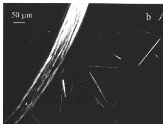
FIGURE 3. Photomicrographs using cross-polarized light with analyzer vibration direction oriented E-W. (A) Sample 12 “byssolitic” actinolite. Low-birefringence fibers lie on (100) and exhibit parallel extinction; high-birefringence fibers do not go to extinction during rotation of the stage. (B) Sample 253 actinolite asbestos. Individual fibers and fibers in bundles show extinction angles ranging from 0 to 16°. Fibers with inclined extinction range in width to approximately 3 \mu\text{m} . (C) Sample 255 actinolite asbestos. All fibers and fiber bundles exhibit parallel extinction.
