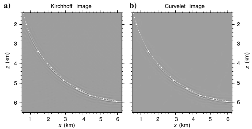
Figure 12. Essentially the same test as in Figure 8, but for a larger traveltime: CO Kirchhoff-migrated result (a) versus the result obtained from the coordinate transformation combined with amplitude scaling (b). The centers of the coordinate-transformed curvelets are indicated by the white circles. In the curvelet image, accuracy is obtained only in neighborhoods of the centers of the transformed curvelets.
