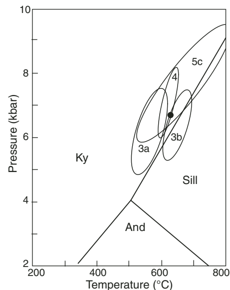
Figure 4. Thermobarometry results, plotted as 2\sigma error ellipses for each sample. Aluminosilicate triple junction shown for reference; average pressure and temperature from the four samples shown by solid dot. And—andalusite; Ky—kyanite; Sill—sillimanite.
