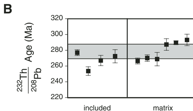
Figure 5. (A) X-ray maps of Mn and Ca concentrations in garnet from sample 5c. Scale bar—500 microns. (B) Th-Pb monazite results from same sample. Grey bar indicates weighted mean of all analyses plus 2\sigma .
