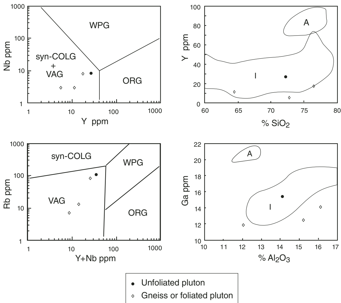
Figure 9. Geochemical discrimination diagrams, after Pearce et al. (1984) and Collins et al. (1982). Fields labels: A—A-type granites; I—I-type granites; ORG—ocean ridge granites; syn-COLG—syn-collision granites; VAG—volcanic arc granites; WPG—within-plate granites.
