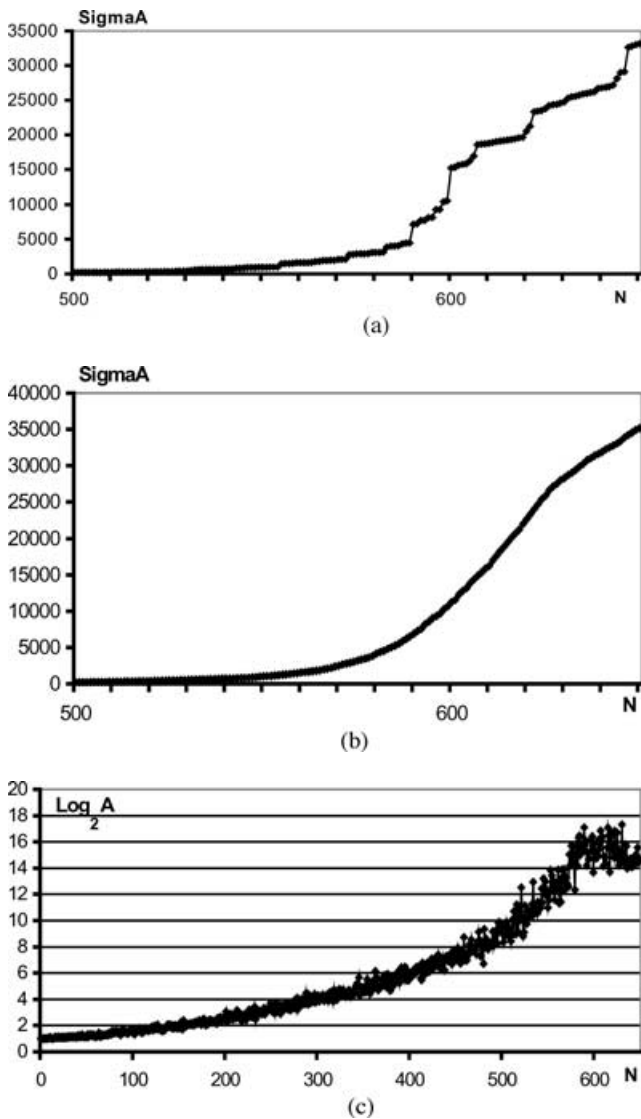
Figure 5. (a) Cumulative graph of amplitude ( \Sigma A ) versus number of damaged sites N for a single run (lattice 30 \times 30 )—analogue of Benioff curve; p_c = 0.67 or N = 600 . (b) Cumulative graph of amplitude ( \Sigma A ) versus number of damaged sites N averaged for 100 runs (lattice 30 \times 30 ); p_c \approx 0.65 or N \approx 600 . (c) Cumulative graph of amplitude versus number of damaged sites N for 100 runs in semilogarithmic scale (lattice 30 \times 30 ); p_c \approx 0.65 or N \approx 600 . Note increase in (averaged) scatter close to p_c .
