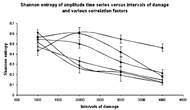
Figure 10. Shannon entropy of amplitude time-series for different damage intervals. Shannon entropy for values of k_h = 1 (diamonds), 8 (squares), 16 (triangles), 32 (crosses), 64 (stars) and 128 (circles) are shown sequentially. Error bars show standard deviation for the same events sequence of shifted windows, containing the same number of events.
