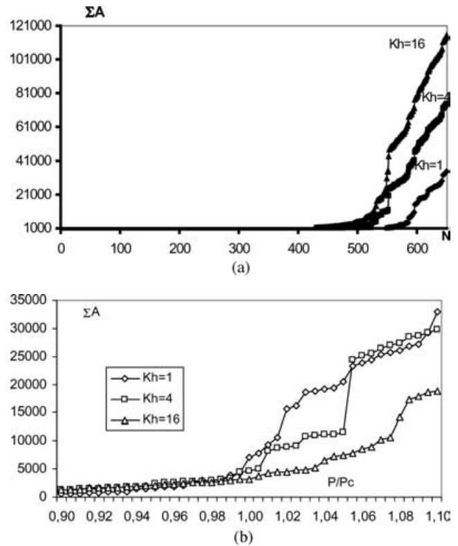
Figure 6. Cumulative graph of amplitudes larger than 1000 ( \Sigma A > 1000 ) versus number of damaged sites N for a single run at different correlation factors Kh = 1, 4, 16 (lattice 30 \times 30 ); note that for Kh = 1 P_c = 0.586 , for Kh = 4 P_c = 0.524 and for Kh = 16 P_c = 0.491 .
