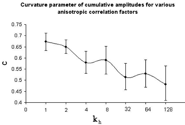
Figure 8. Curvature parameters of amplitude time-series at various anisotropic correlation factors k_h .
