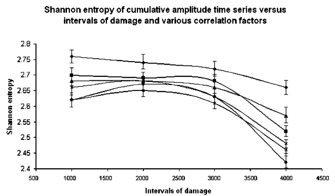
Figure 11. Shannon entropy of cumulated amplitude time-series for different damage intervals. Shannon entropy for values of k_h = 1 (diamonds), 8 (squares), 16 (triangles), 32 (crosses), 64 (stars) and 128 (circles) are shown sequentially. Error bars show standard deviation for the same events sequence of shifted windows, containing the same number of events.
