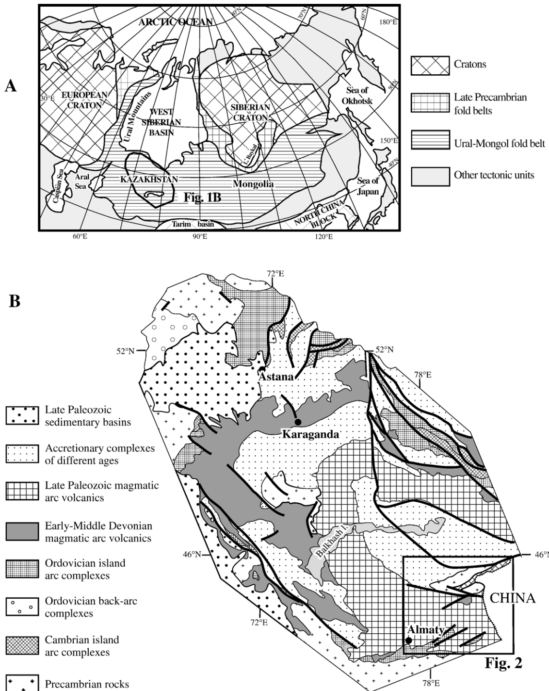
Fig. 1. (A) Location of the Ural–Mongol fold belt within Eurasia and outline of Fig. 1B in Kazakhstan. (B) Schematic map of major rock complexes in Kazakhstan, simplified after Degtyarev (2003) with main faults shown as thick solid lines.
