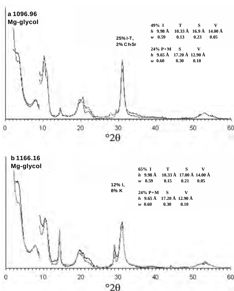
Figure 3. Experimental (solid) and simulated (shadowed) XRD patterns for Mg-saturated and glycolated samples. The scale above 10^\circ 2\theta has been increased by a factor of four in order to demonstrate discrepancies between experimental and calculated patterns: (a) 1096.96; (b) 1166.16. Oriented specimens. Parameters of the models are shown, together with peak positions for the simulated patterns. CoK \alpha radiation.
