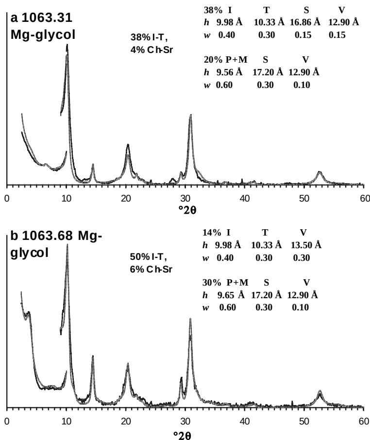
Figure 2. Experimental (solid) and simulated (shadowed) XRD patterns for Mg-saturated and glycolated samples. The scale above 10^\circ 2\theta has been increased by a factor of four in order to demonstrate discrepancies between experimental and calculated patterns; (a) 1063.31; (b) 1063.68. Oriented specimens. Parameters of the models are shown, together with peak positions for the simulated patterns. CoK \alpha radiation.
