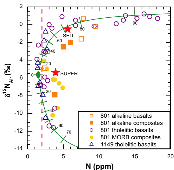
Fig. 6. Diagram of N concentrations and isotopic compositions for individual AOC samples from Sites 801 and 1149 and for composites for Site 801. Note that (1) samples with less than 2 ppm N (mean 1.5 ppm) and \delta^{15}\text{N} values around -5.6\text{‰} may represent characteristics of “fresh” basalts; (2) high N-bearing samples ( >4 ppm) have relatively homogeneous \delta^{15}\text{N} values around +0.4 \pm 0.7\text{‰} , implying that the most significant enrichment of N is from sediments; (3) the N with extremely negative values could possibly be attributed to abiotic reduction of mantle-like \text{N}_2 to \text{NH}_3 and then assimilation of this \text{NH}_3/\text{NH}_4^+ by AOC (see text for discussion). Also shown are two-endmember mixing lines between MORB and sedimentary N (upper line) and between MORB and abiotically reduced N (lower line). Numbers along the mixing lines represent fractions of secondary N from corresponding source. Nitrogen compositions for the three endmembers are: (1), “Fresh” MORB: N = 1.5 ppm and \delta^{15}\text{N} = -5.6\text{‰} , based on the data average of six relatively unaltered basalts from Sites 801 and 1149. (2) Sediments: \delta^{15}\text{N} = +1.8\text{‰} , based on the data average of the lowest overlying sediment samples analyzed at 801 (Sadofsky and Bebout, 2004) and the composite of intercalated sediments in basalts. (3) \text{NH}_3 reduced from mantle-like \text{N}_2 : \delta^{15}\text{N} = -16\text{‰} , based on a N-isotope fractionation of 11\text{‰} at the hydrothermal temperatures (Urey, 1947; Hanschmann, 1981). In these calculations, poorly known N isotope discrimination is neglected for the other steps of N transfer that involve no species change of N.
