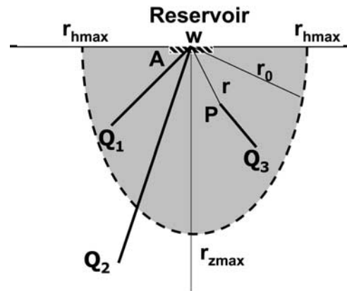
Figure 2. The instantaneous affect of loading a reservoir of width w occurs within the shaded area, at a distance r_0 from the bottom of the reservoir, A. The distance r_0 varies from r_{zmax} below the reservoir to r_{hmax} near the surface. These distances are 6 to 7 and 3 to 4 times the width of the reservoir, w , respectively. The undrained, instantaneous pore pressure increases at any point A or P is B times the average stress increase at that location, where B is the Skempton's coefficient. The delayed pore pressure increases at Q_1 , Q_2 , and Q_3 occur because of the pore pressure diffusion along discrete fractures (solid lines) connecting them to sources of instantaneous elevated pressures at A and P, respectively. If P is connected to A by a discrete fracture there will be a coupled effect at P (see text for details).
