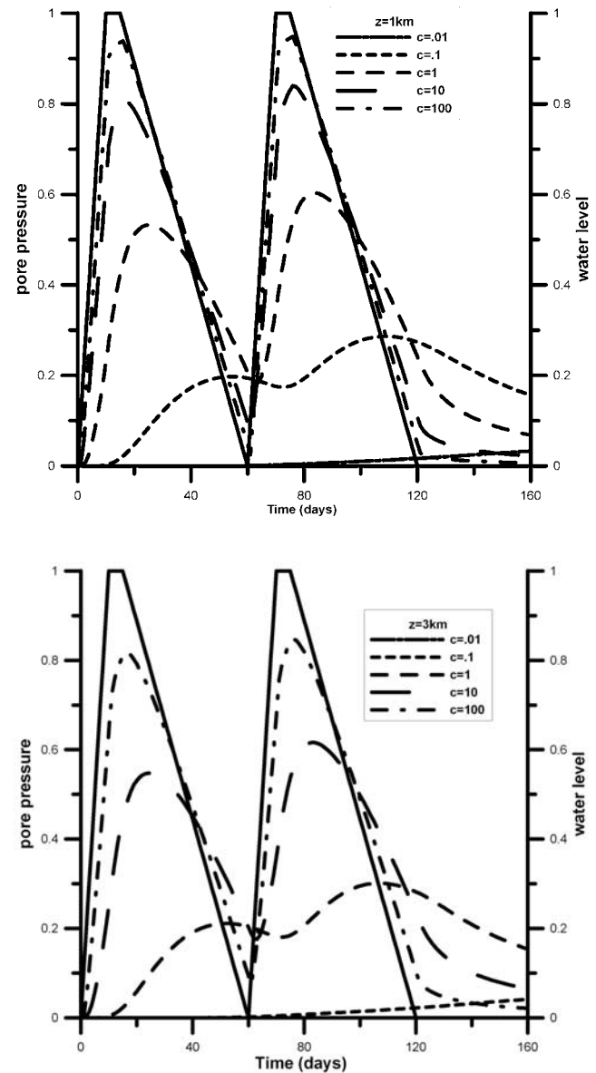
Figure 4. (a and b) Two cycles of filling (solid line) and the corresponding normalized changes in pore pressures due to diffusion at depths of 1 and 3 km for various diffusivity values (in \text{m}^2/\text{s} ). The rate of change of pore pressure ( dp/dt ) at these depths is shown in Figures 4c and 4d. (c and d) An increase in dp/dt after the filling (shaded areas) occurs at 1- and 3-km depths for c = 0.1 and 1 \text{ m}^2/\text{s} , respectively.
