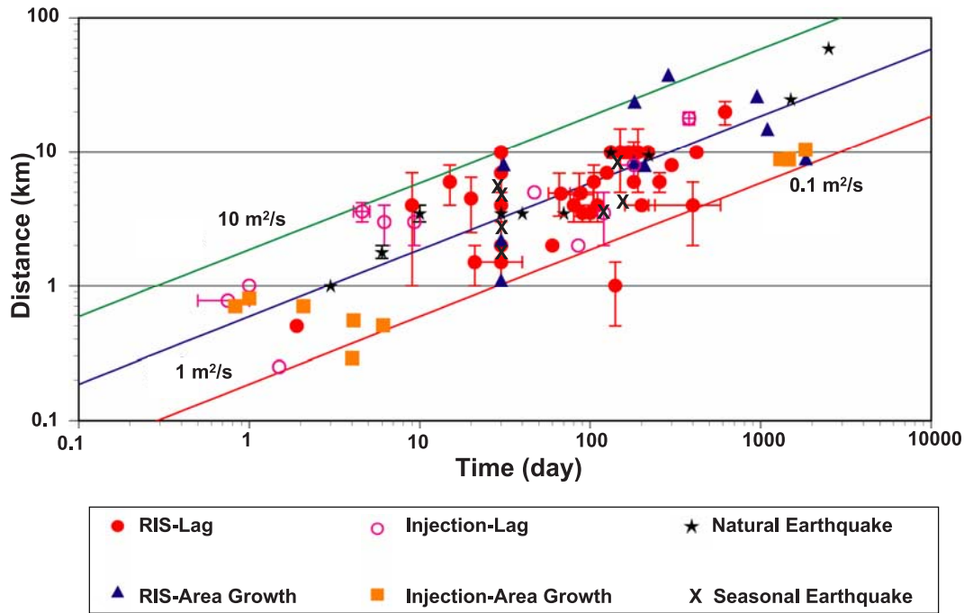
Figure 8. Plot showing the observed distance time delay data. RIS lag and injection lag refer to cases where the time lag between filling and seismicity were used to calculate c . Area growth refer to cases where the rate of epicentral growth was used. Natural earthquakes refer to cases where precursory data were used to calculate c . Seasonal refers to the cases where a seasonal time lag was used. The parallel lines show hydraulic diffusivity values of 0.1, 1, and 10 \text{m}^2/\text{s} calculated using equation (5). Virtually, all the diffusivity values lie between 0.1 and 10 \text{m}^2/\text{s} , a range which is called seismogenic diffusivity c_s .
