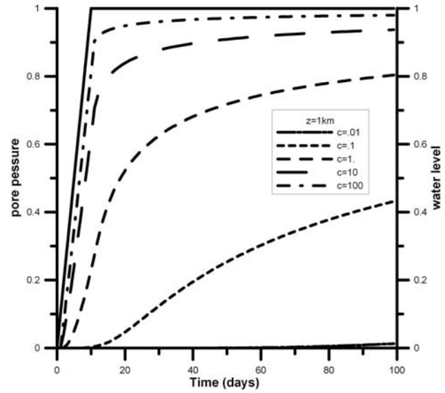
Figure 3. The filling curve at reservoir where the water level is maintained after impoundment (solid line). The dashed curves show the corresponding increase in the pore pressure diffusion at a depth of (a) 1 km and (b) 3 km for various diffusivity values (in square meters per second), and (c and d) their rate of change ( dp/dt ) at those depths. The pore pressures are normalized with respect to the pore pressures corresponding to the lake levels. After the initial filling, an increase in the dp/dt (shaded area) occurs at 1- and 3-km depths corresponding to c = 0.1 and 1 \text{ m}^2/\text{s} , respectively (Figures 3c and 3d).
