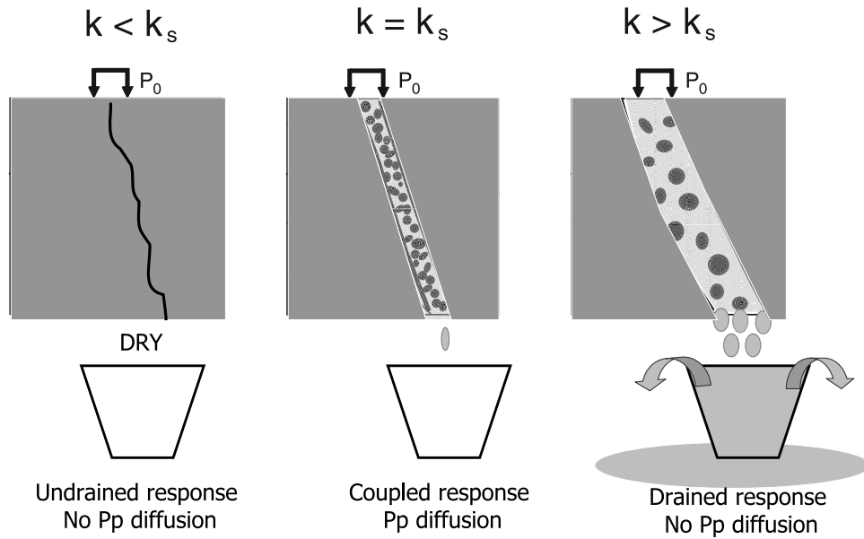
Figure 10. Cartoon to explain the consequences of loading a fracture with permeability k , where k is less than, equal, and greater than k_s .
