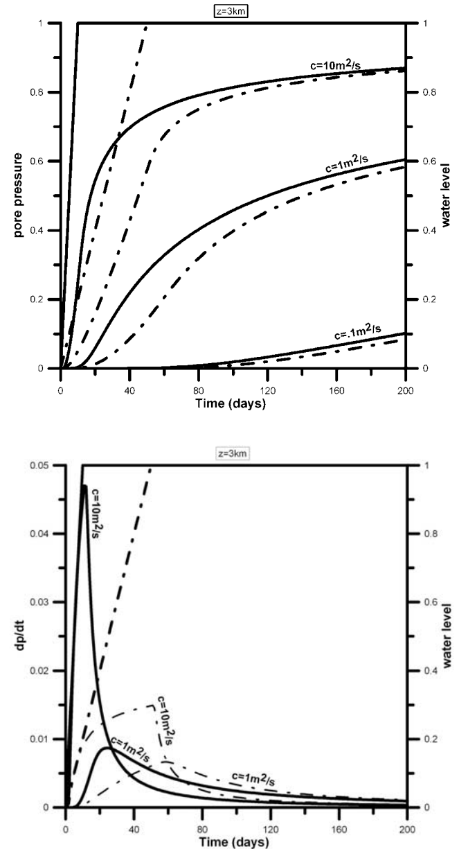
Figure 5. (a) Comparing normalized pore pressures at a depth of 3 km for different values of c (in square meters per second) for two filling curves, (b) and the corresponding changes in dp/dt for c = 10.0 and 1.0 \text{ m}^2/\text{s} . The solid and dashed lines are for reservoir impoundment in 10 and 50 days, respectively, after which the water level is maintained.
