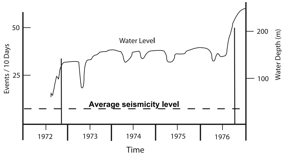
Figure 6. The times of increased seismicity (vertical lines) that followed increases in lake levels in July 1972 and June 1976 at Nurek reservoir. The time lags between times of lake level increases and seismicity onset were used to calculate hydraulic diffusivity (modified from the work of Simpson and Negmatullaev [1981]).
