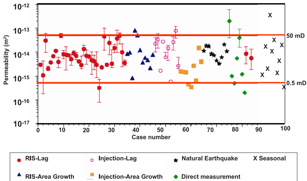
Figure 9. Results of the calculation of intrinsic permeability k using values of c shown in Figure 8 and equation (6), and six direct measurements at locations of induced seismicity. The symbols are the same as were used in Figure 8. The permeability of fractures associated with seismicity lies between 5 \times 10^{-16} and 5 \times 10^{-14} \text{ m}^2 . This range has been labeled seismogenic permeability, k_s .
