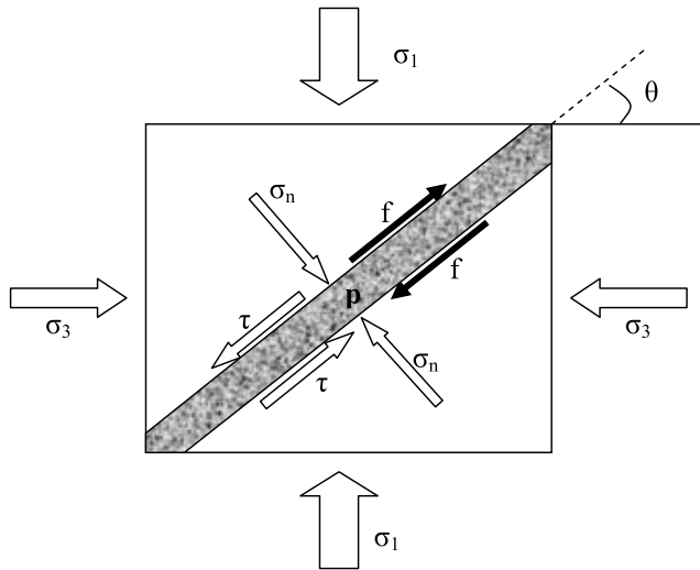
Figure 1. A fluid-filled fracture with pore fluid pressure p subjected to a two-dimensional stress field. \sigma_n , \tau , and f are the normal, shear, and frictional stresses, respectively (modified from the work of Tezuka and Niitsuma [2000]).
