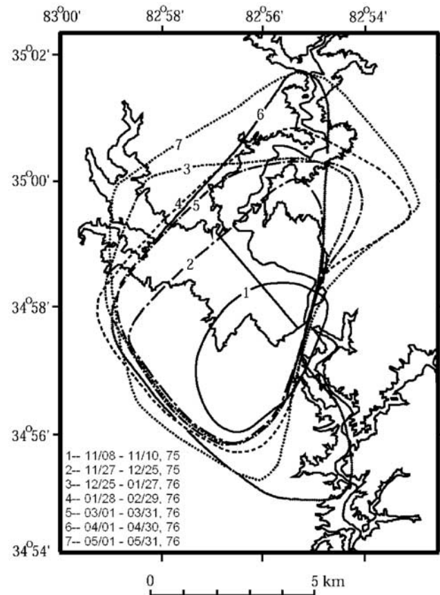
Figure 7. Epicentral growth of seismicity at Lake Jocassee, South Carolina from November 1975 to May 1976 (after Talwani and Acree [1984]). The rate of growth was used to calculate c .
