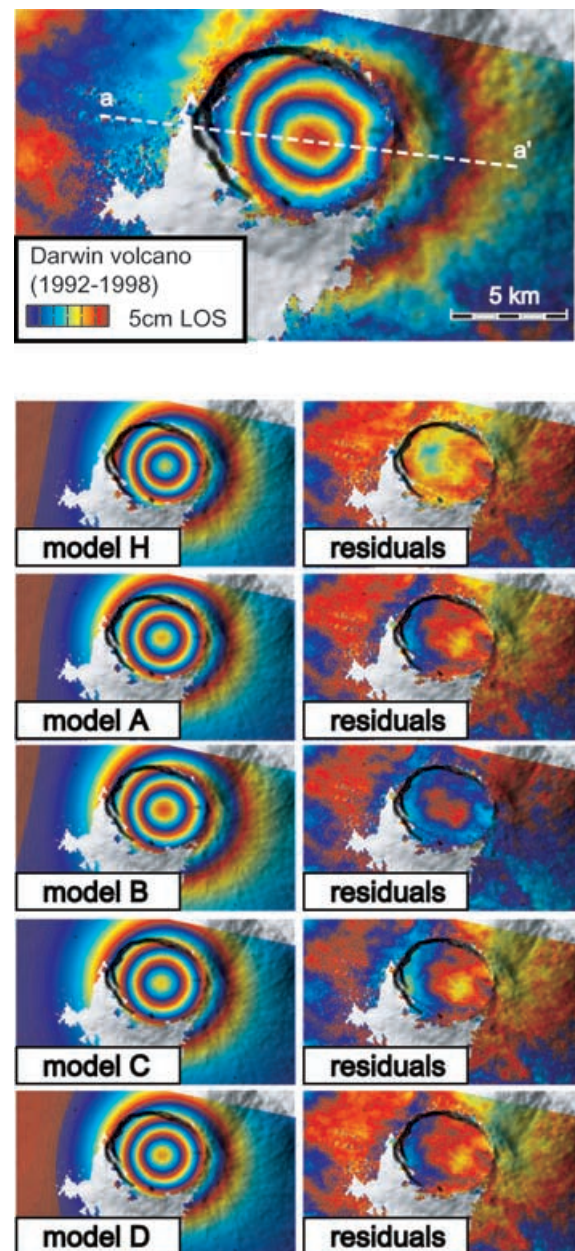
Figure 10. InSAR line-of-sight (LOS) surface displacements at Darwin volcano during 1992–1998. (Top panel): LOS displacements towards ERS-1 and ERS-2 satellites. The images are from track 140, descending orbit. Baseline is 85 m. Azimuth looking angle of the satellites is \sim 283^\circ , whereas incidence angle is \sim 23^\circ . Section a–a' is parallel to the looking angle of the satellite. Each cycle colour represents 5 cm of LOS displacement. See also Amelung et al. (2000) and (down panel) (left column) Synthetic LOS displacements predicted by the five different models considered in this study, with the homogeneous model H, and the heterogeneous layered models A–D; (right column) Residual analysis show that all layered models yield very good results in reproducing the observed surface displacement.
