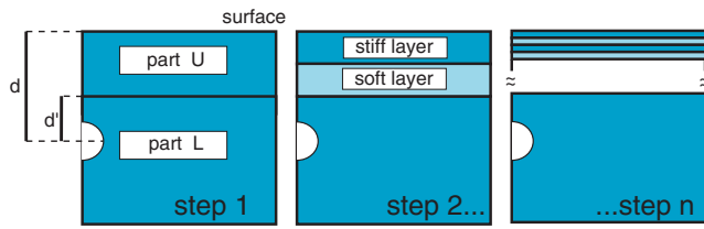
Figure 4. Multilayered heterogeneous models. Scheme used to study the effect of mechanical layering. At step 1 we divide the model into an upper part U and a lower part L. The inflating magma chamber is embedded in the homogeneous part L at depth d from the surface and d' from the layered part U. Further layering is introduced in part U. At each subsequent step, we increase the number of layers in the part U while decreasing their thickness. We keep the same alternation scheme ('stiff-soft', stiff material at the surface) and also consider the opposite alternation scheme ('soft-stiff', soft material at the surface).
