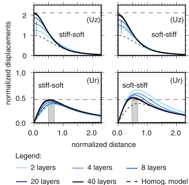
Figure 6. Influence of number and/or thickness of layers on part U (step 2-n, see Fig. 4). Here are shown the results for magma chamber at 3.5 km depth (model A setup). The upper two graphs show vertical displacement U_z , the lower two graphs show radial displacement U_r , the left column is with stiff layer at the surface, the right column with soft layer at the surface. Vertical and horizontal surface displacements in layered models are amplified in respect with the homogeneous half-space (dashed line). Note that displacements of the models on the left ('stiff-soft' scheme) and the models on the right column ('soft-stiff' scheme) converge if more layers are considered.
