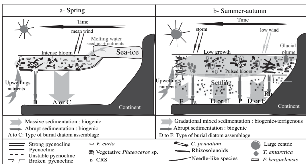
Figure 6 Conceptual model for the deposition of the different laminations and sublaminiae recorded in core MD03-2601 for the spring season (a) and the summer–autumn season (b)
