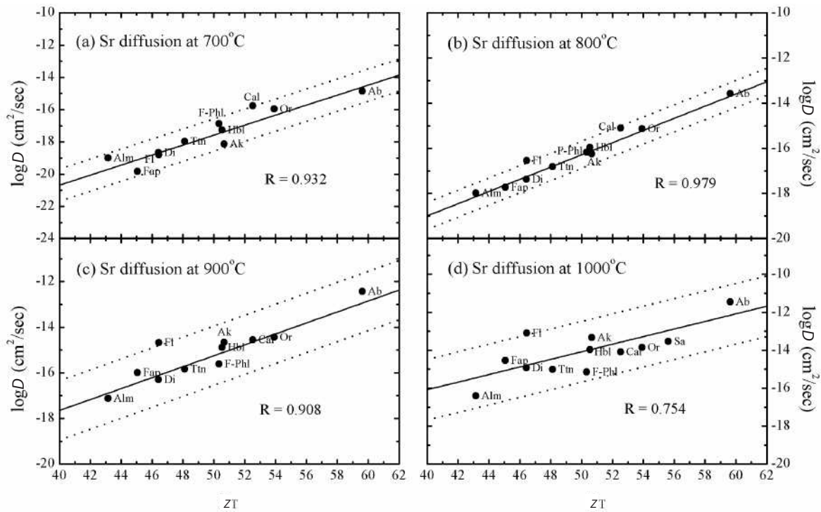
FIGURE 4. Plots of \log D (diffusivity) for Sr vs. total ionic porosity ( Z_T ) in minerals at temperatures of: (a) 700, (b) 800, (c) 900, and (d) 1000 °C. Solid lines denote best linear fits to the experimental data (Eqs. 16–19), whereas dotted lines bracket 1\sigma uncertainties of the regressions. Mineral abbreviations, diffusion parameters, and data references are given in Table 1.
