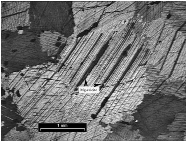
Fig. 10 Microphotograph of calcite grains in sample L6, showing Mg-rich lamellae exsolved in the calcite
