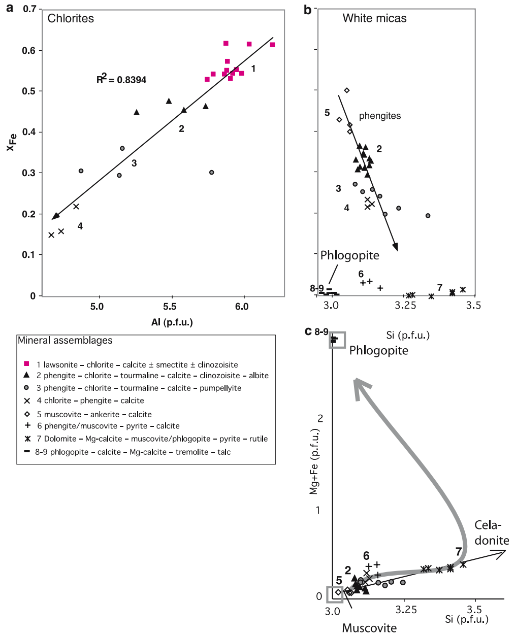
Fig. 7 Chemical composition of Karakorum low metamorphic grade chlorites ( a ) and white micas ( b, c ). Numbers 1 to 9 refer to the successive mineral assemblages found across the metamorphic pile. The arrows indicate the direction of increasing metamorphic grade. X_{Fe} is the ratio of Fe/(Mg + Fe) recalculated as cationic contents
