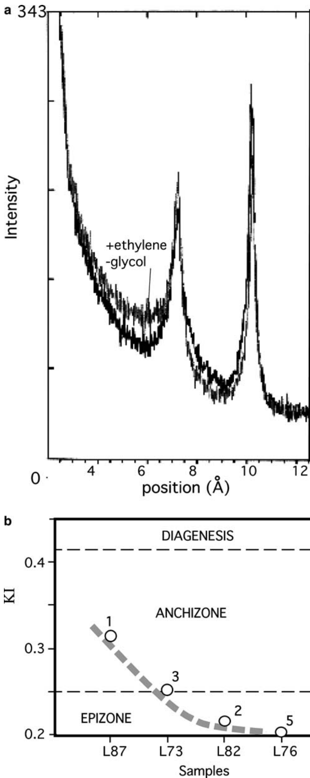
Fig. 8 X-ray diffraction characteristics of Karakorum lower-grade samples. a Comparison of X-ray spectra of smectite-chlorite from sample L87 (assemblage 1) obtained with (grey) and without (black) ethylene-glycol added to sample L73 powder. Positions in Å are recalculated from 2\theta . Indices of clay minerals are from Lanson and Meunier (1995). b Kübler Index (KI) of illite crystallinity in lower-grade samples. Numbers 1, 2, 3 and 5 refer to assemblages numbers, and samples are also indicated (L73-87)
