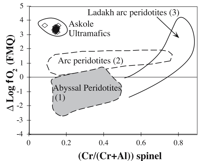
Fig. 12 Spinel Cr# and oxygen fugacity ( \Delta\text{Log}f_{\text{O}_2} ) values of Askole ultramafic bands. For the data of the fields 1 (abyssal peridotites) and 2 (arc peridotites) see Parkinson and Arculus (1999), and 3 (Ladakh arc peridotites), see Rolland et al. (2002a)
