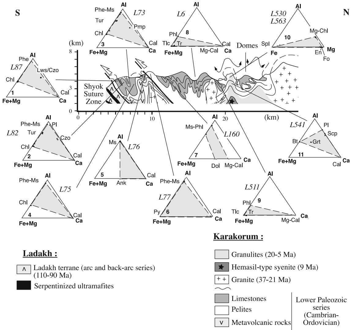
Fig. 5 Successive assemblages observed with increasing metamorphic grade in marbles of the Lower Paleozoic series along a N-S geological cross-section, from the Shyok Suture Zone (south) to the core of the Karakorum terrain (north). Ternary projections of mineral compositions ( small dots ) are done with mineral compositions in cation% with respect to Al, Fe+Mg and Ca. Mineral abbreviations are following Kretz (1983)
