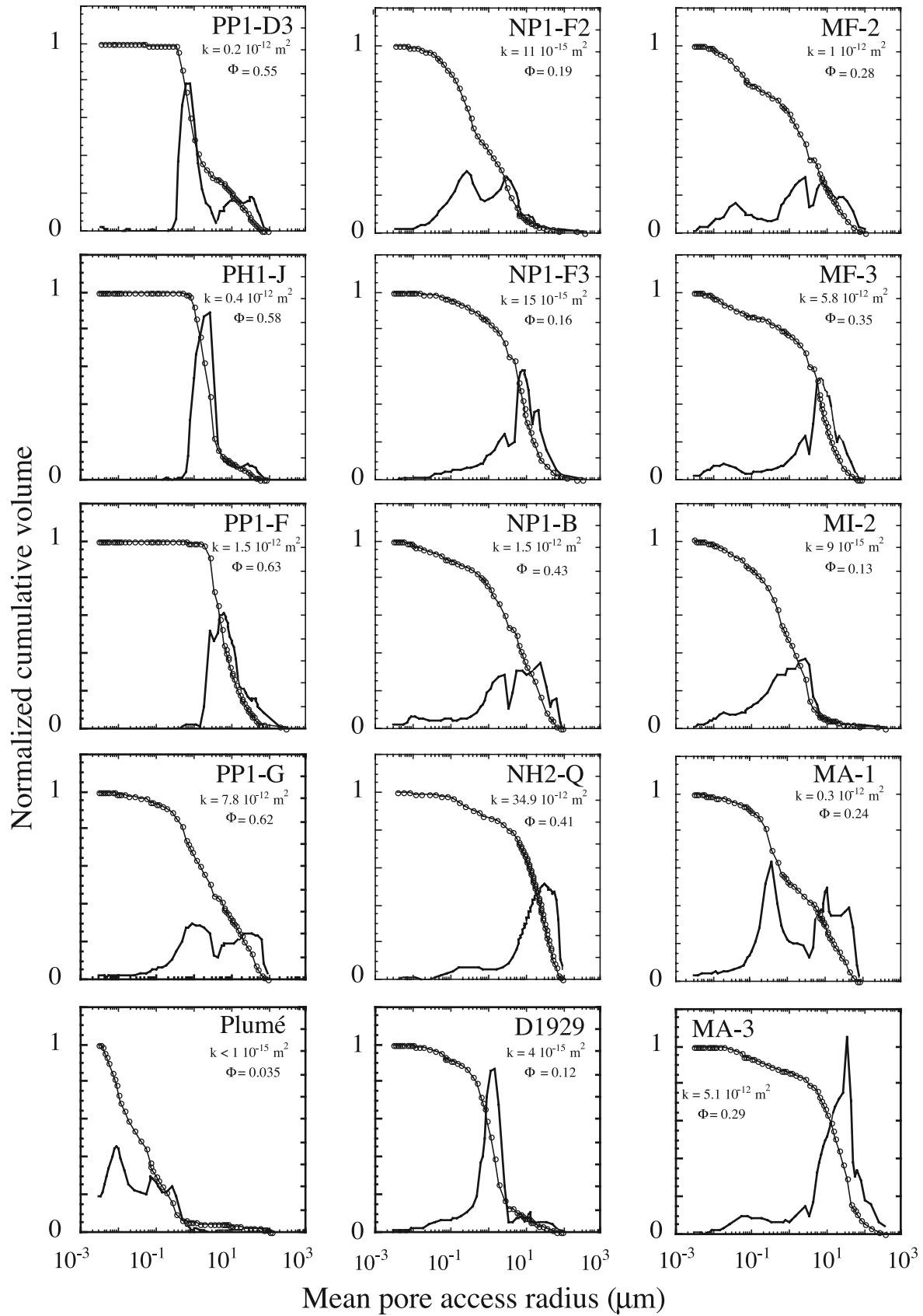
Figure 4. Distributions of pore access radius (solid line) and normalized cumulative volume of mercury injected (solid line with circles) from Hg porosimetry measurements on 15 samples characteristics of Montagne Pel  e deposits. The k and \Phi are the permeability and the porosity, respectively, of the samples. See sample designations in Table 1.
