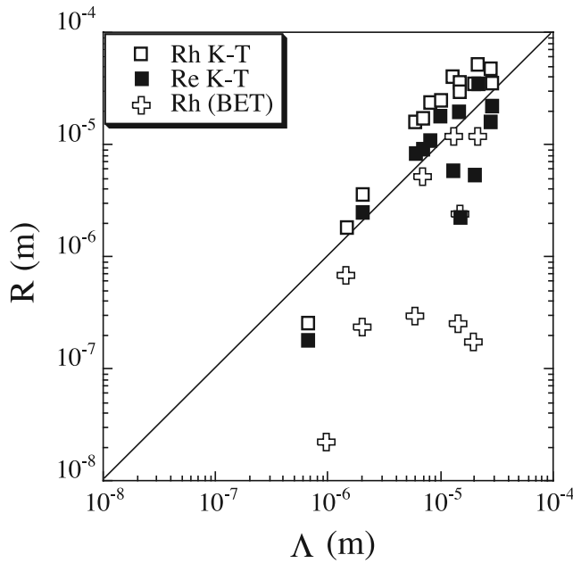
Figure 11. Comparison between different characteristics lengths controlling transport properties. \Lambda is computed using the Johnson and Schwartz [1989] model. R_h BET is deduced from BET measurement. R_h K-T and R_e K-T are estimated from H_g porosimetry experiment and correspond to R_h^{\max} and R_e^{\max} , the two characteristic radius introduced by Katz and Thompson [1987].
